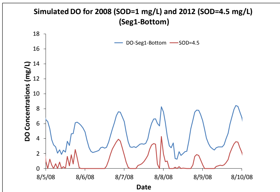
Figure 5.13d. Sensitivity analysis for DO at Segment 1 bottom 2008 and 2012.
