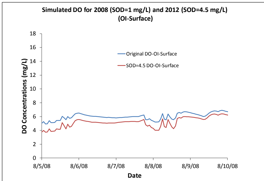
Figure 5.13a. Sensitivity analysis for DO at OI surface 2008 and 2012.
