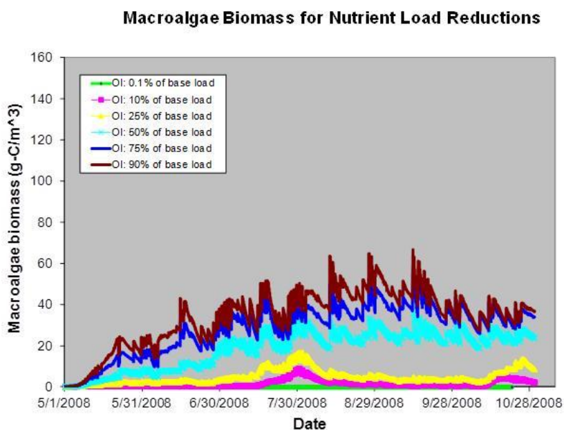
Figure 5.19a. Macroalgae biomass at Ol for nutrient load reduction scenarios.
