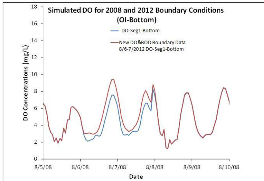
Figure 5.8b. Simulated DO at bottom Segment 1 (blue) between the 2008 and the new 2012 DO (red) data at the boundary.
