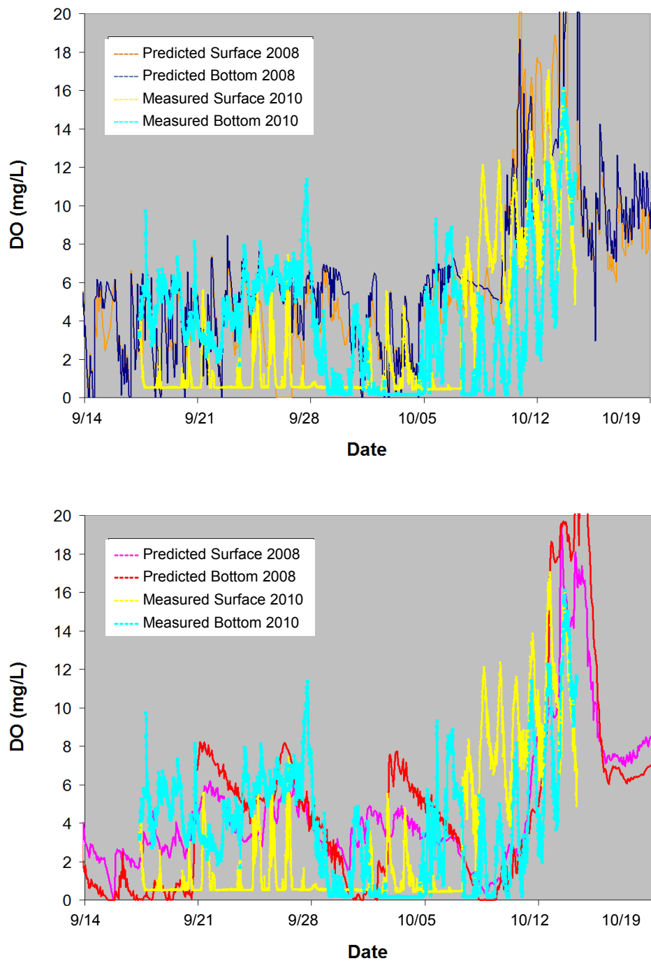
Figure 5.5. Comparison of predicted surface and bottom water dissolved oxygen based on 2008 input data with measured surface and bottom water data in 2010 for Segment 1 (top) and Ocean Inlet (bottom).
