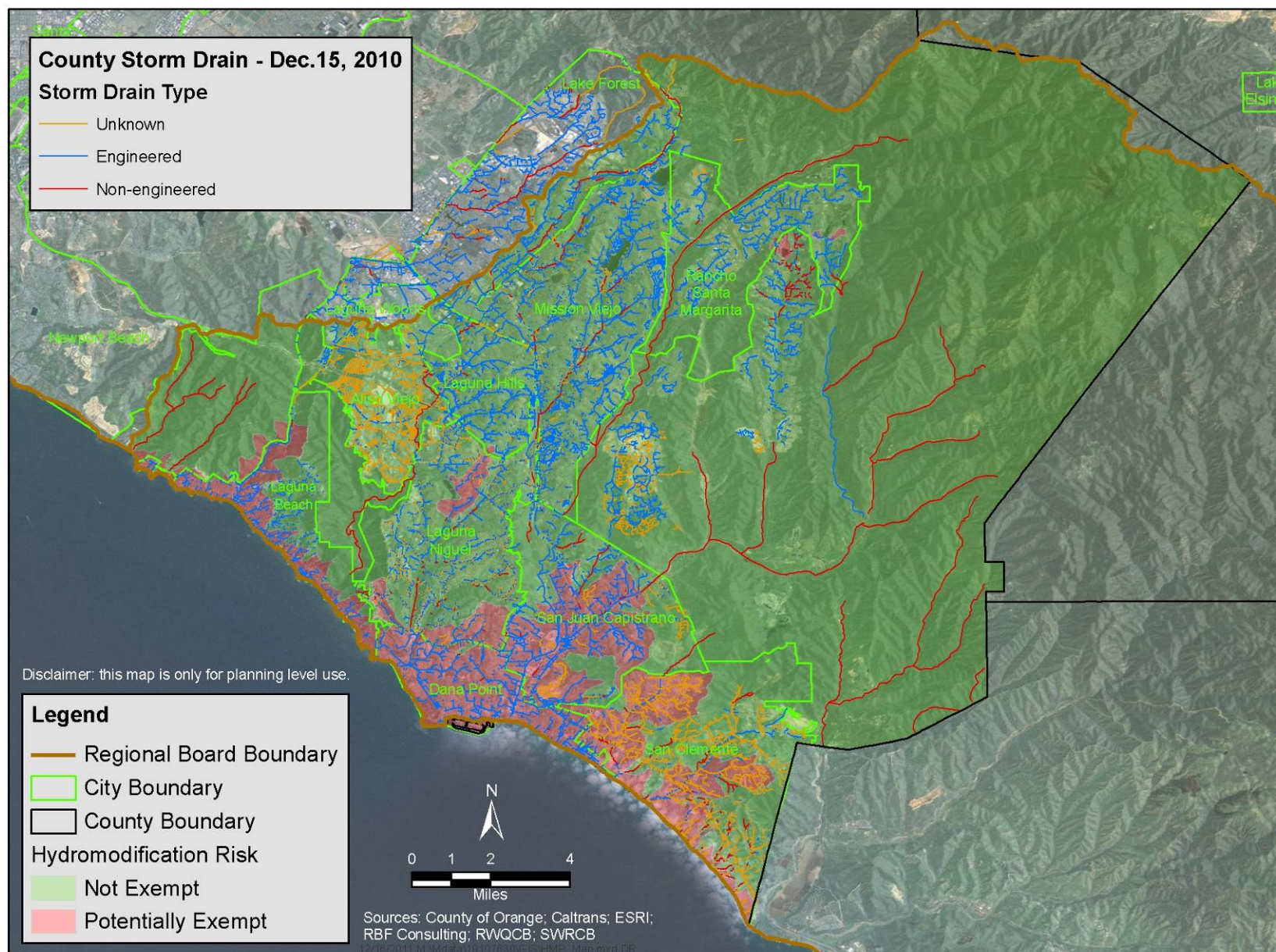
Figure 4-1: South Orange County Storm Drain Inventory 2010
