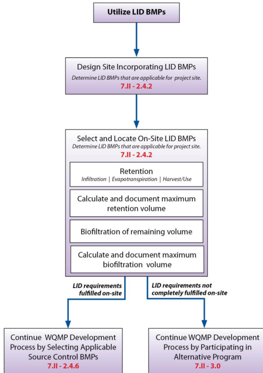
Figure 7.II-5: Design the Site Incorporating LID BMPs – Without HCOCs
