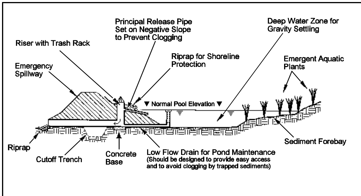
Figure 5-5. Retention Pond
