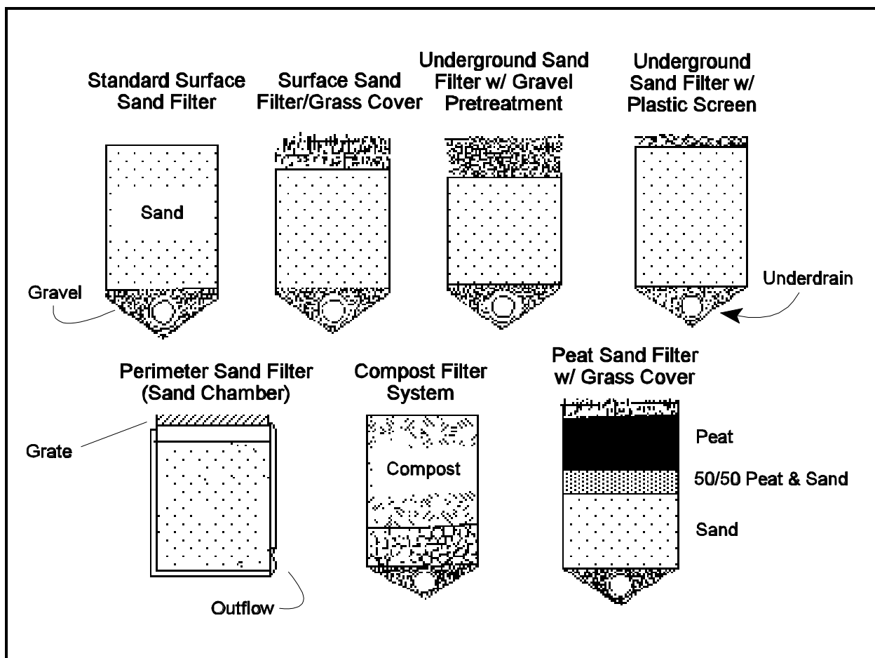
Figure 5-7. Filter Media
