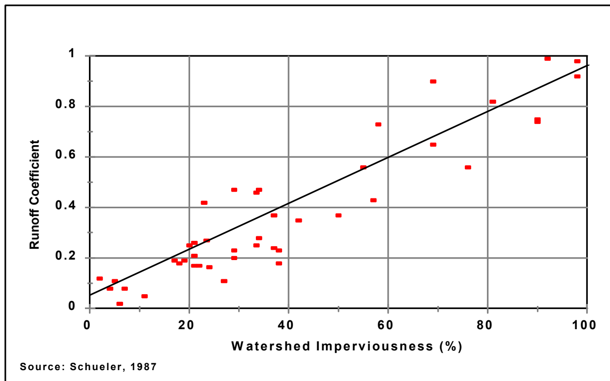
Figure 4-6. Relationship of Watershed Imperviousness to Runoff Coefficient Levels
