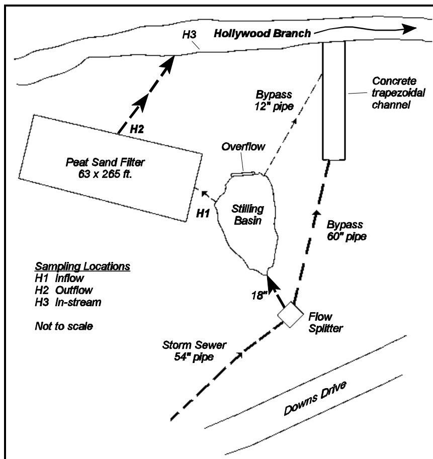
Figure 5-16. Hollywood Branch Peat/Sand Filter
