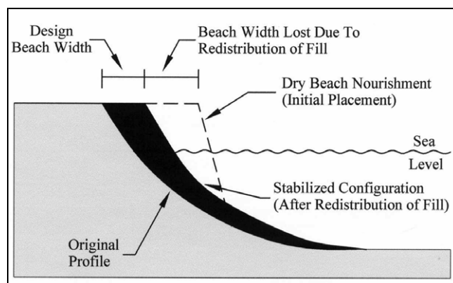
Figure 7.2 Dry Beach Nourishment (CA Dept. of Boating and Waterways and State Coastal Conservancy, 2002)
