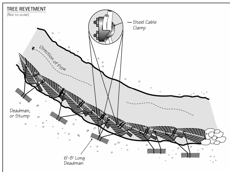
Figure 7.28 Tree Revetment (USDA-FS, 2002)
