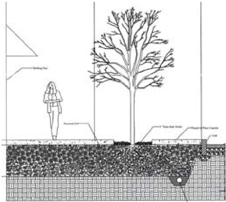
Figure 7. Structural soils provide void space for root growth and load-bearing for sidewalk
