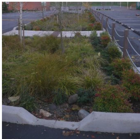
Figure 6. Bioretention facility in Oregon.
