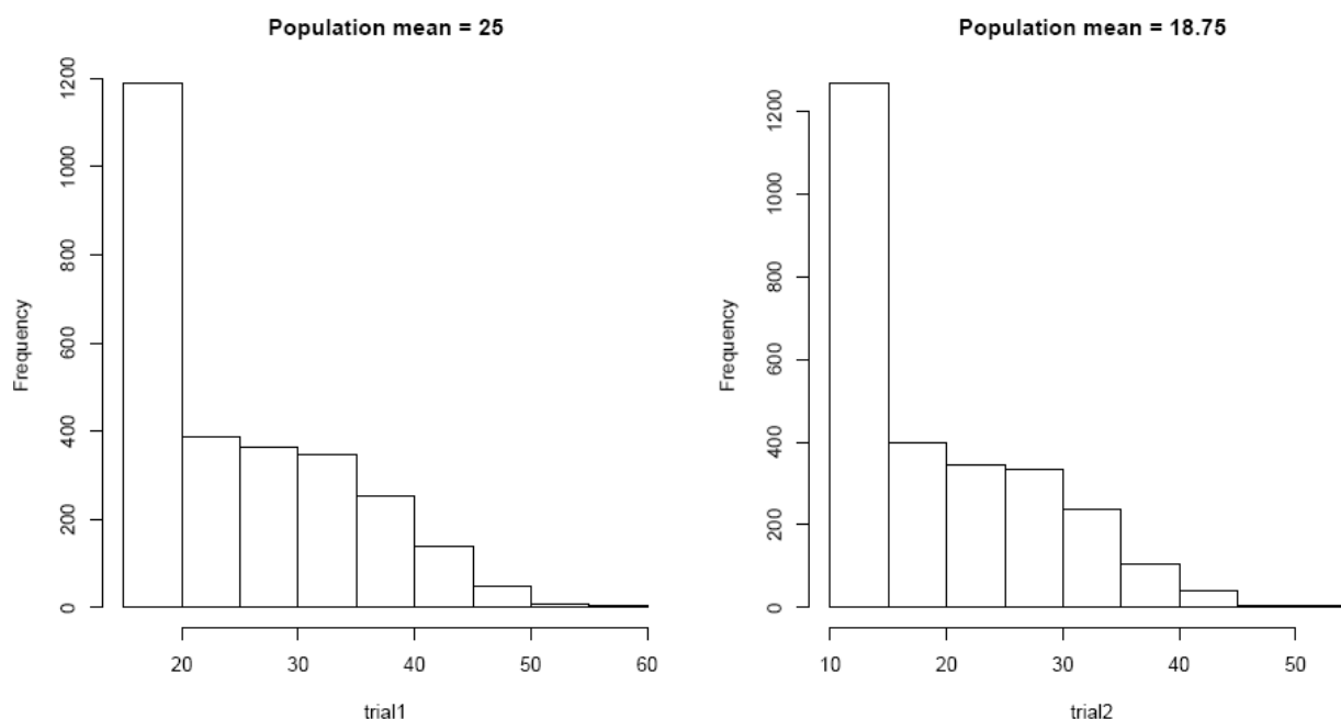
Figure A-3. Simulated frequency distributions of Ceriodaphnia reproduction data with two populations having non-normal data and different means. Both populations have a standard deviation of 7.7.
