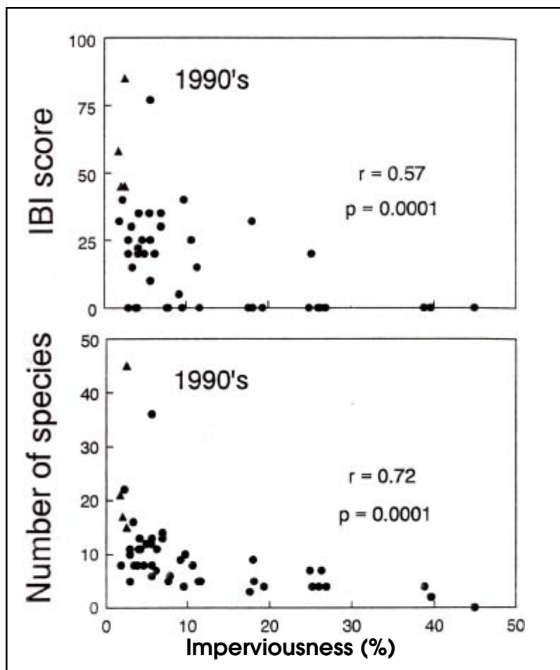
Figure 49: Fish-IBI and Number of Species vs. % IC in Wisconsin Streams (Wang et al. , 1997)
