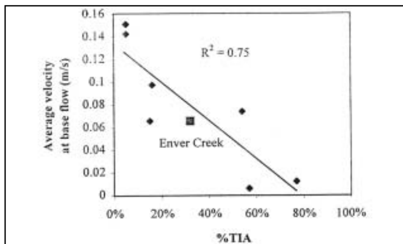
Figure 18: Effect of Watershed IC on Summer Stream Velocity in Vancouver Streams (Finkebine et al. , 2000)
