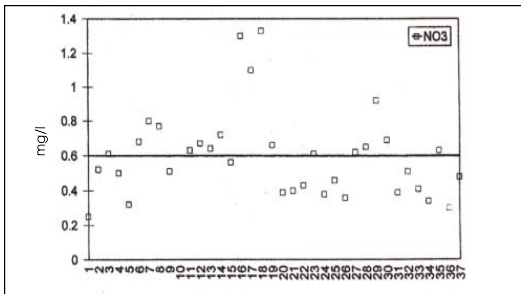
Figure 32: Nitrate-Nitrogen Concentration in Stormwater Runoff at 37 Sites Nationally (Schueler, 1999)
