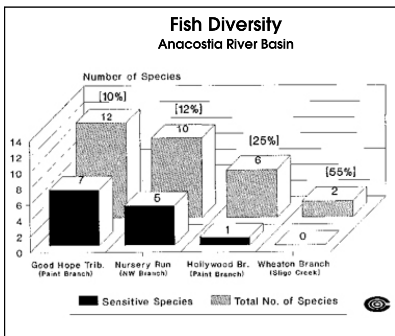
Figure 50: IC and Effects on Fish Species Diversity in Four Maryland Subwatersheds (MWCOG, 1992)
