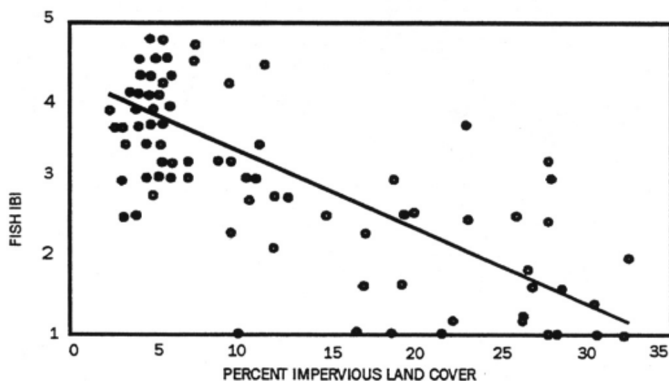
Figure 48: Fish-IBI vs. Watershed IC for Streams in the Patapsco River Basin, MD (Dail et al. , 1998)
