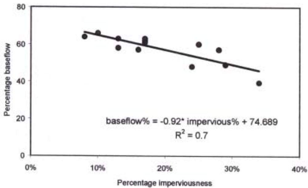
Figure 16: Relationship Between Percentage Baseflow and Percent IC in Massachusetts Streams (Saravanapan, 2002)
