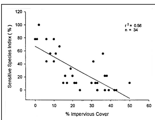
Figure 46: IC vs. Aquatic Insect Sensitivity - EPT Scores in Delaware Streams (Maxted and Shaver, 1997)
