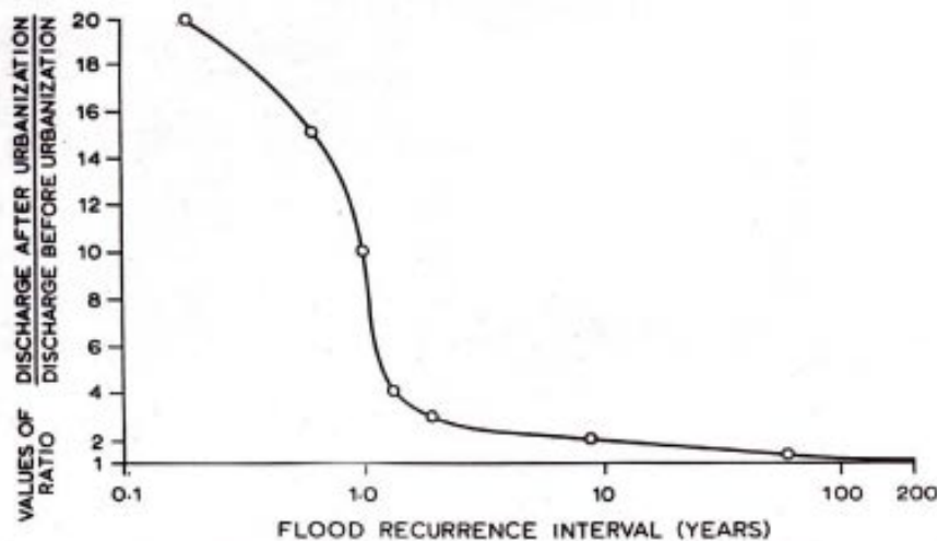
Fig. 3. Effect on flood magnitudes of paving 20% of a basin (based on Figure 2).
