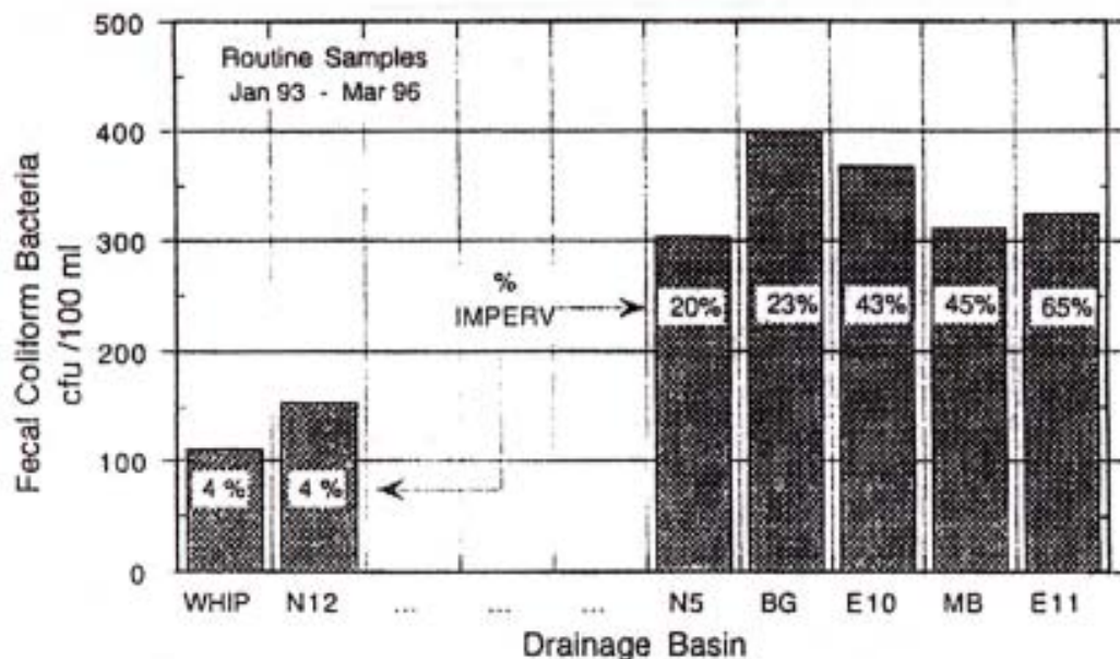
Figure 36: Relationship Between IC and Fecal Coliform Concentrations in New York Streams (Hydroqual, 1996)
