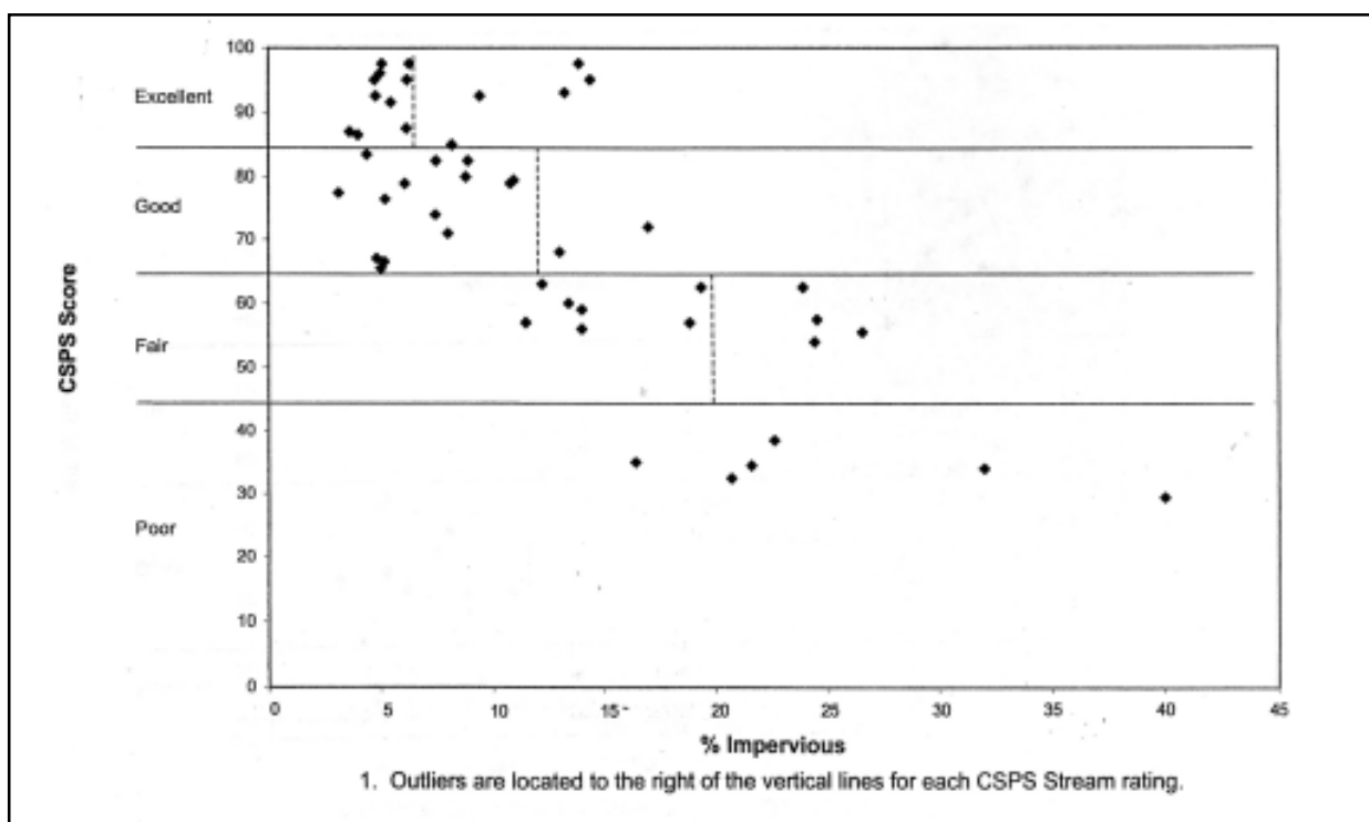
Figure 40: Combined Fish and Benthic IBI vs. IC in Maryland Piedmont Streams (MNCPPC, 2000)
