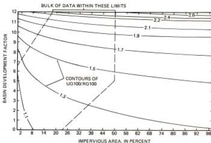
Figure 10: Relationship of Urban/Rural 100-Year Peak Flow Ratio to Basin Development Factor and IC (Sauer et al. , 1983)
