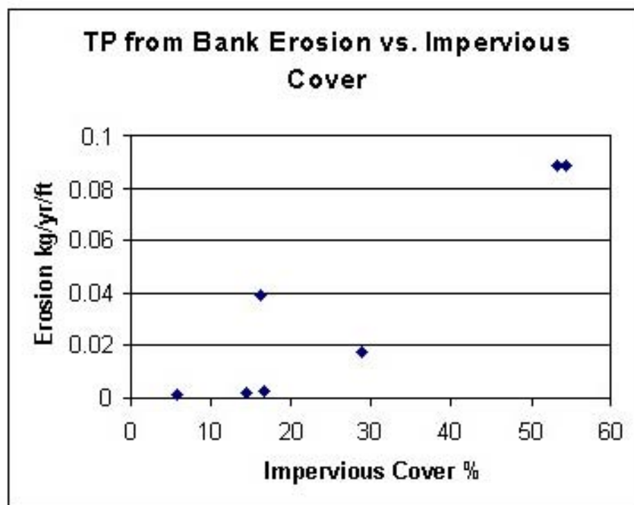
Figure 34: Total Phosphorus from Bank Erosion as a Function of IC in Texas Streams (Dartiguenave et al. , 1997)
