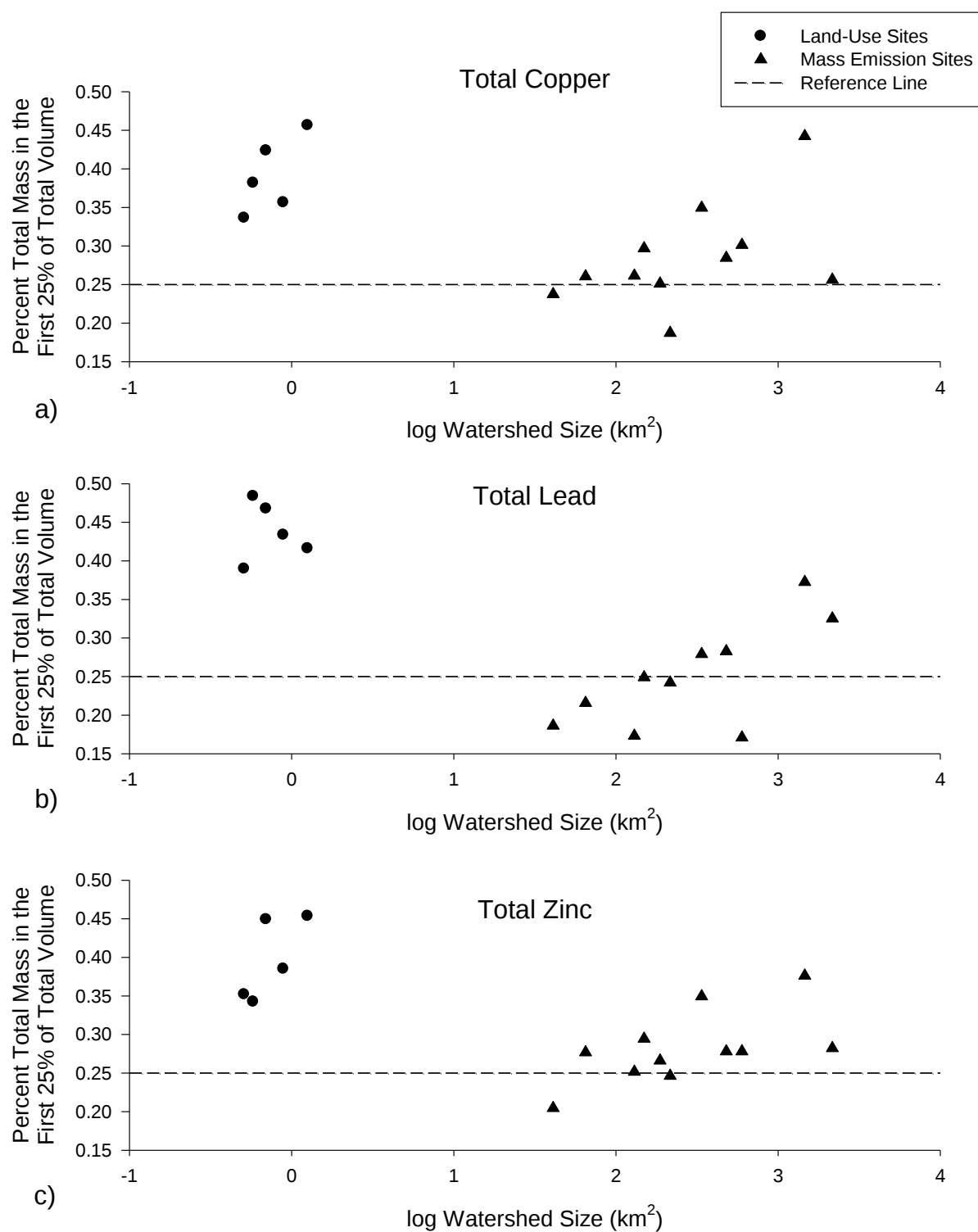
Figure 3-8. First flush patterns of total copper (a), total lead (b), and total zinc (c) in relation to watershed size. Dashed reference line indicates 25% of total mass loading in first 25% of total volume.
