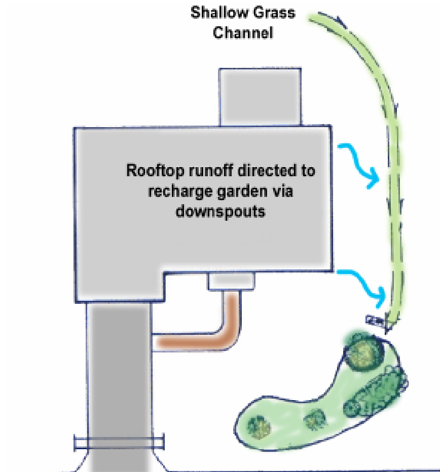
Figure 18. Single-Family Residential Lot Drainage Schematic. Source: Claytor and Schueler, 1995, with modifications by Cahill Associates
