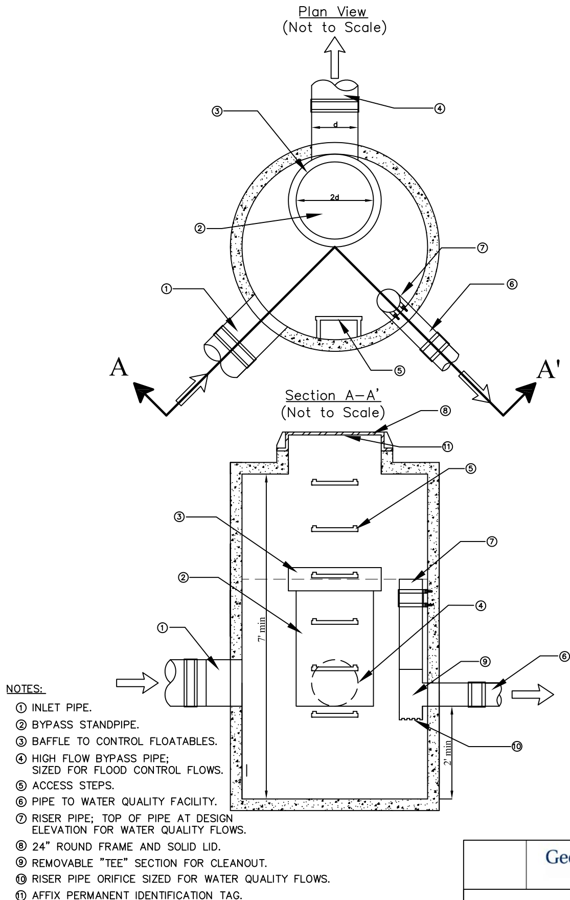
Figure F-2: Flow Splitter Option B
