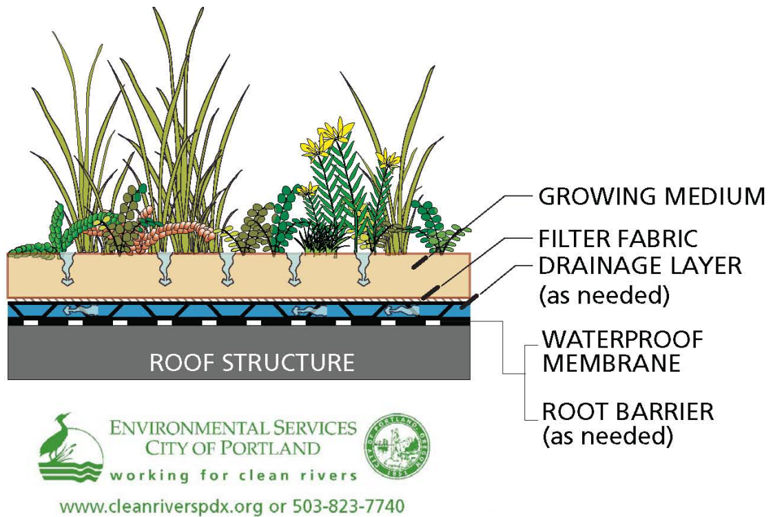
Exhibit A: Green Roof Schematic Courtesy of Portland, OR Environmental Services Department
