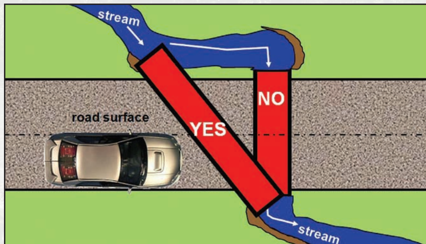
Figure 6.11—Better pipe alignment.
