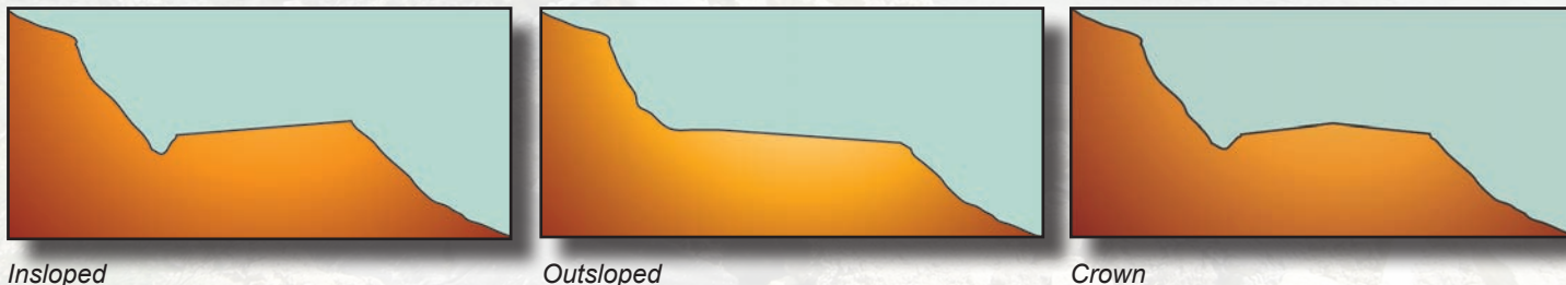
Figures 3.2—Road surface templates.
