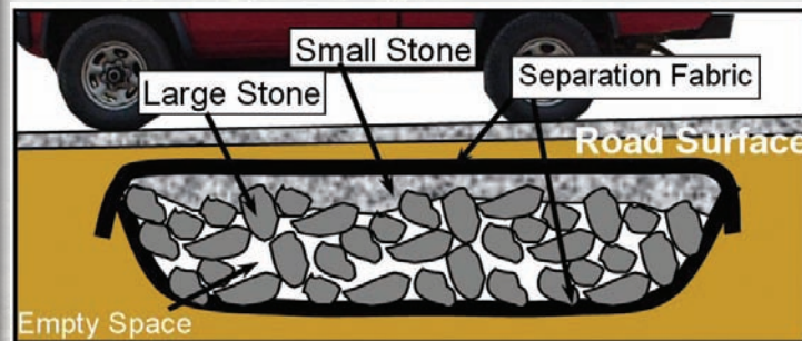
Figure 2.12—Graphical side view of the mattress components.
