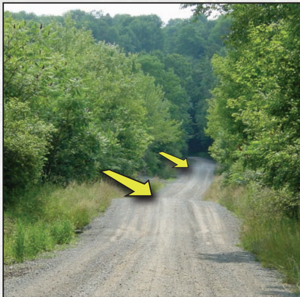
Figure 3.7—The two grade breaks pictured here prevent water from flowing down the road, even if the road's crown were to be lost.
