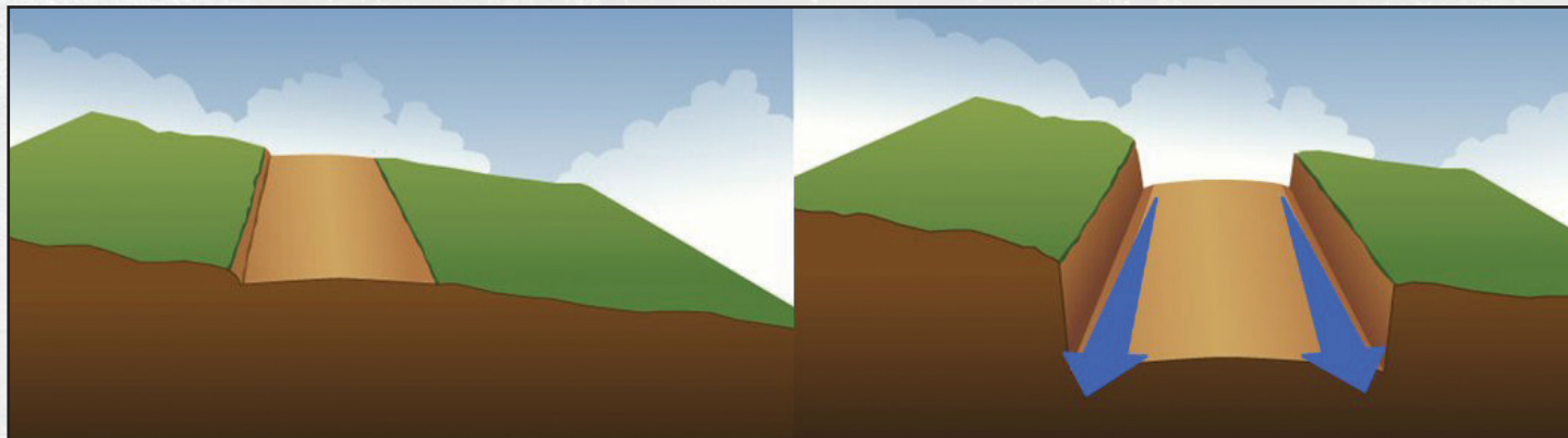
Figure 4.8—Over time, the elevation of many roads, especially unpaved roads, is lowered due to traffic, maintenance, and erosion. When roads become lower than the surrounding terrain, they are referred to as entrenched, and water often is trapped in the road traveled way.
