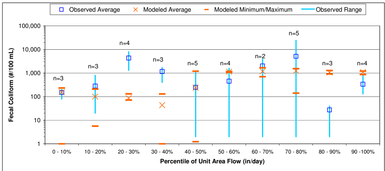
Figure N-23. Graphical comparison of LPSC model results and observed fecal coliform data in the San Diego River watershed (Appendix G, No. 13)
