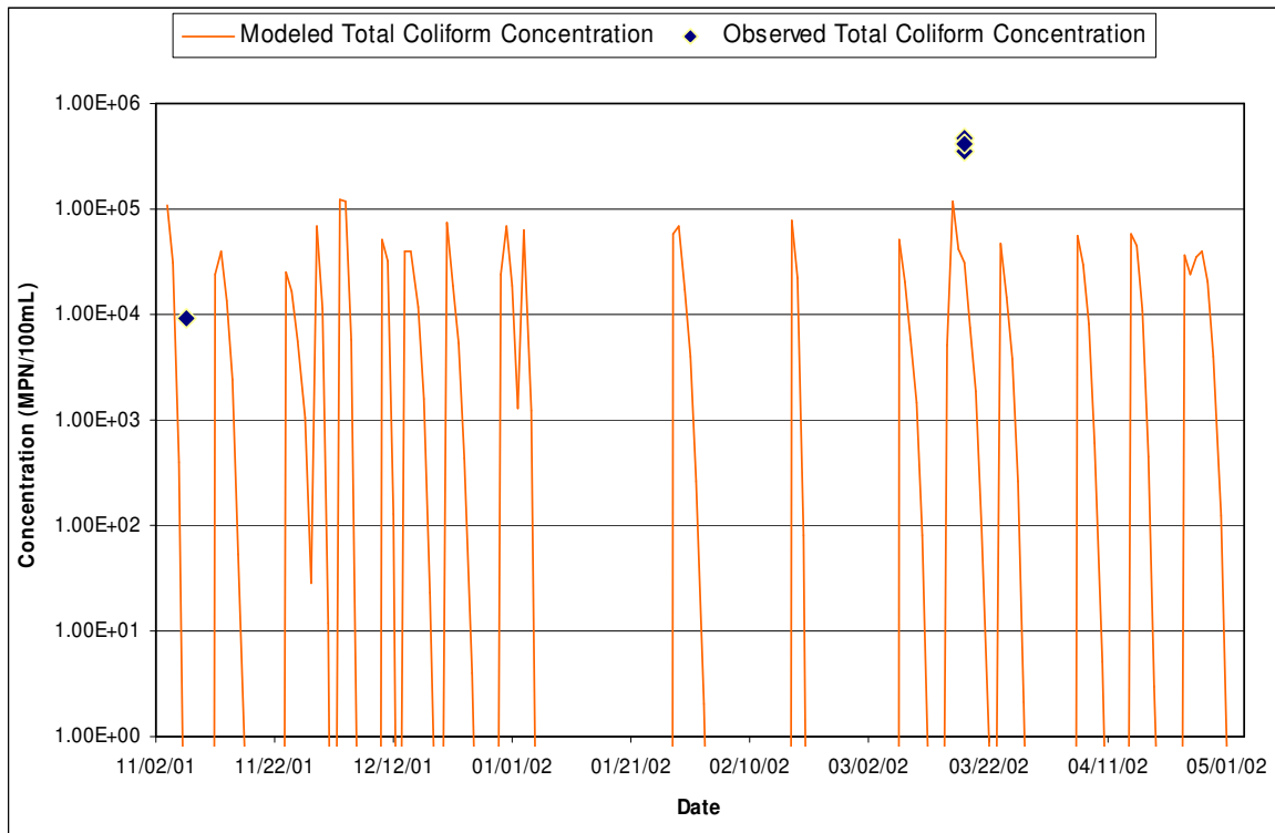
Figure N-7. Time-series comparison of modeled and observed wet weather total coliform densities in the Rose Creek watershed (Appendix G, No. 12 [stations MBW 19, MBW 20 and MBW 21]).
