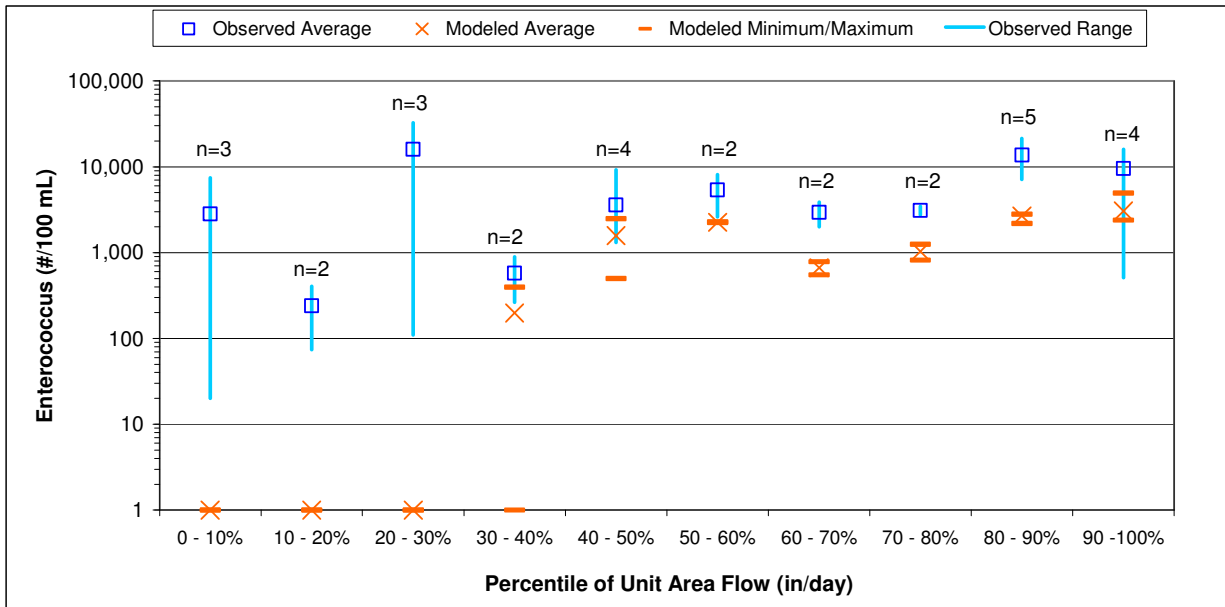
Figure N-22. Graphical comparison of LPSC model results and observed enterococcus data in the Rose Creek and Tecolote Creek watersheds (Appendix G, No. 12)
