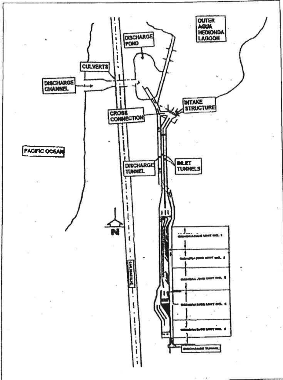
Figure 2. Schematic of Encina Power Station cooling water intake system.
