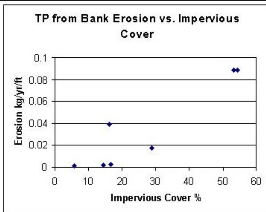
Figure 34: Total Phosphorus from Bank Erosion as a Function of IC in Texas Streams (Dartiguenave et al. , 1997)
