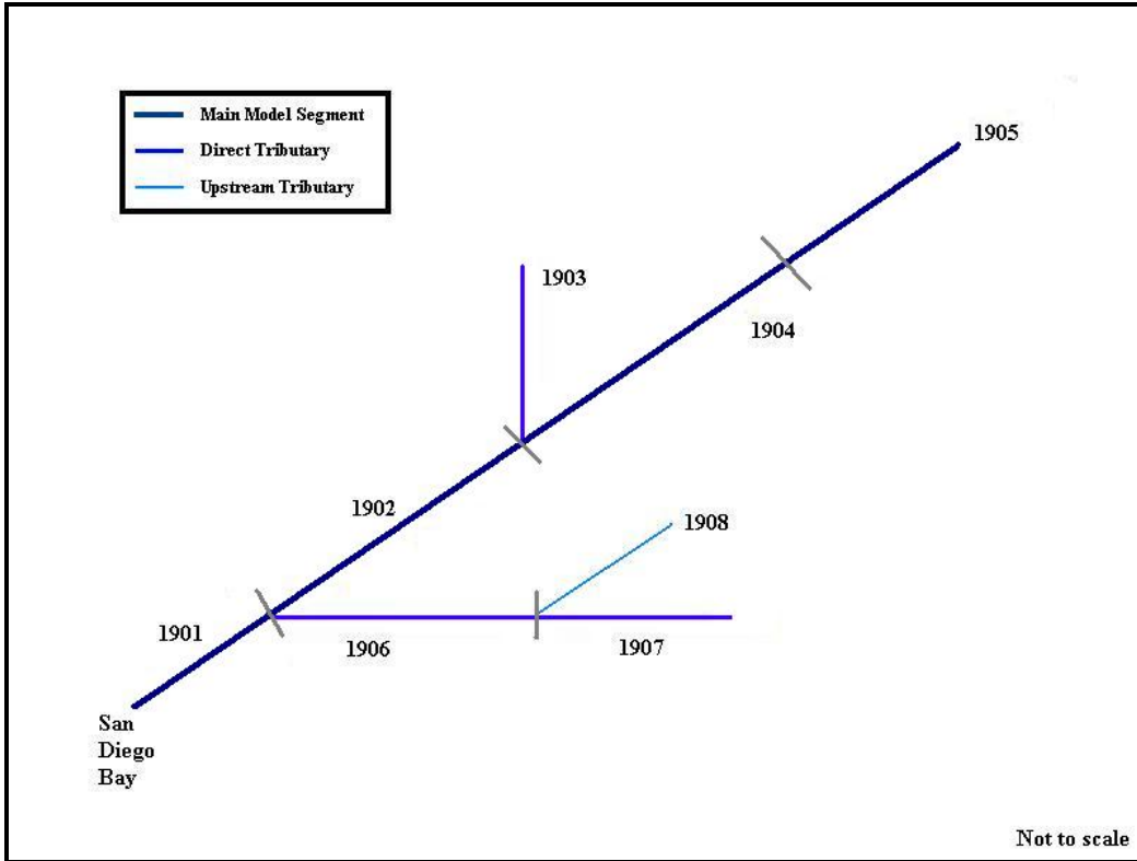
Figure K-2. Schematic of model segments for Chollas Creek and its tributaries
