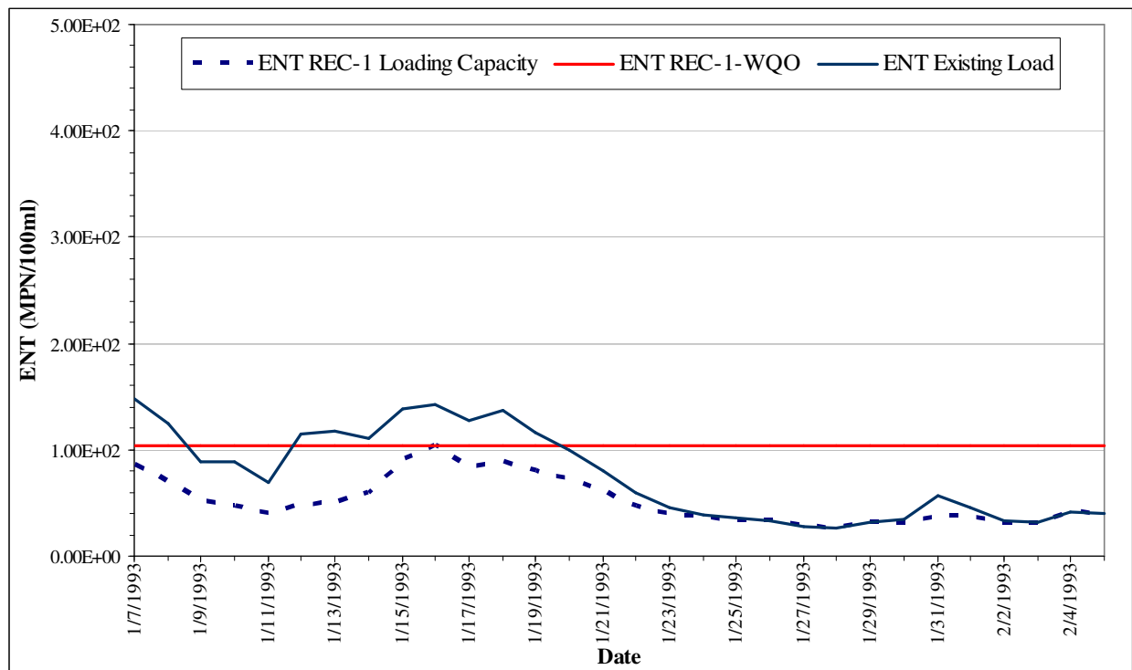
Figure H-6. Existing and Reduced Enterococcus Concentrations at Baby Beach Shoreline, Dana Point Harbor-Wet Weather (Comparison to Single Sample Maximum WQO)
