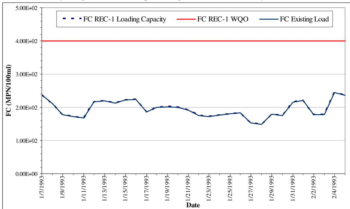
Figure H-5. Existing and Reduced Fecal Coliform Concentrations at Baby Beach Shoreline, Dana Point Harbor-Wet Weather (Comparison to Single Sample Maximum WQO)
