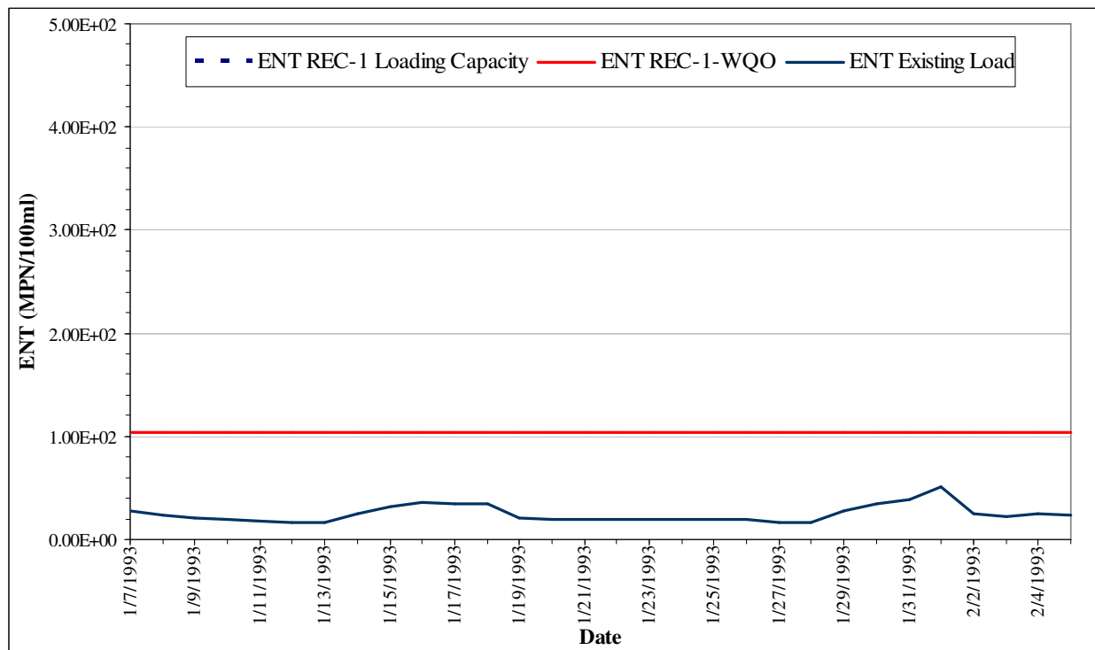
Figure H-3. Existing and Reduced Enterococcus Concentrations at Shelter Island Shoreline Park, San Diego Bay-Wet Weather (Comparison to Single Sample Maximum WQO)
