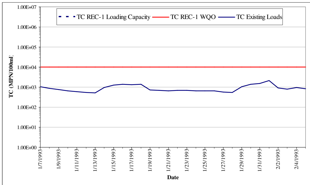
Figure H-1. Existing and Reduced Total Coliform Concentrations at Shelter Island Shoreline Park, San Diego Bay-Wet Weather (Comparison to Single Sample Maximum WQO)
