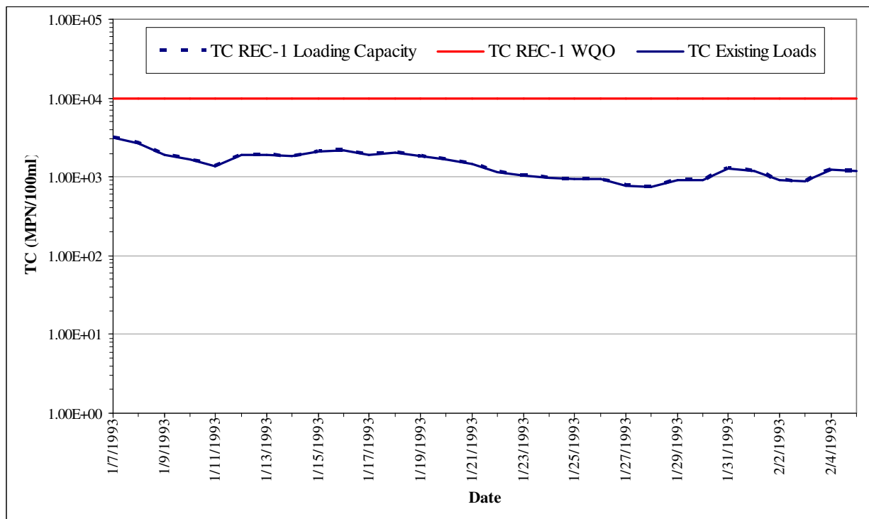
Figure H-4. Existing and Reduced Total Coliform Concentrations at Baby Beach Shoreline, Dana Point Harbor-Wet Weather (Comparison to Single Sample Maximum WQO)
