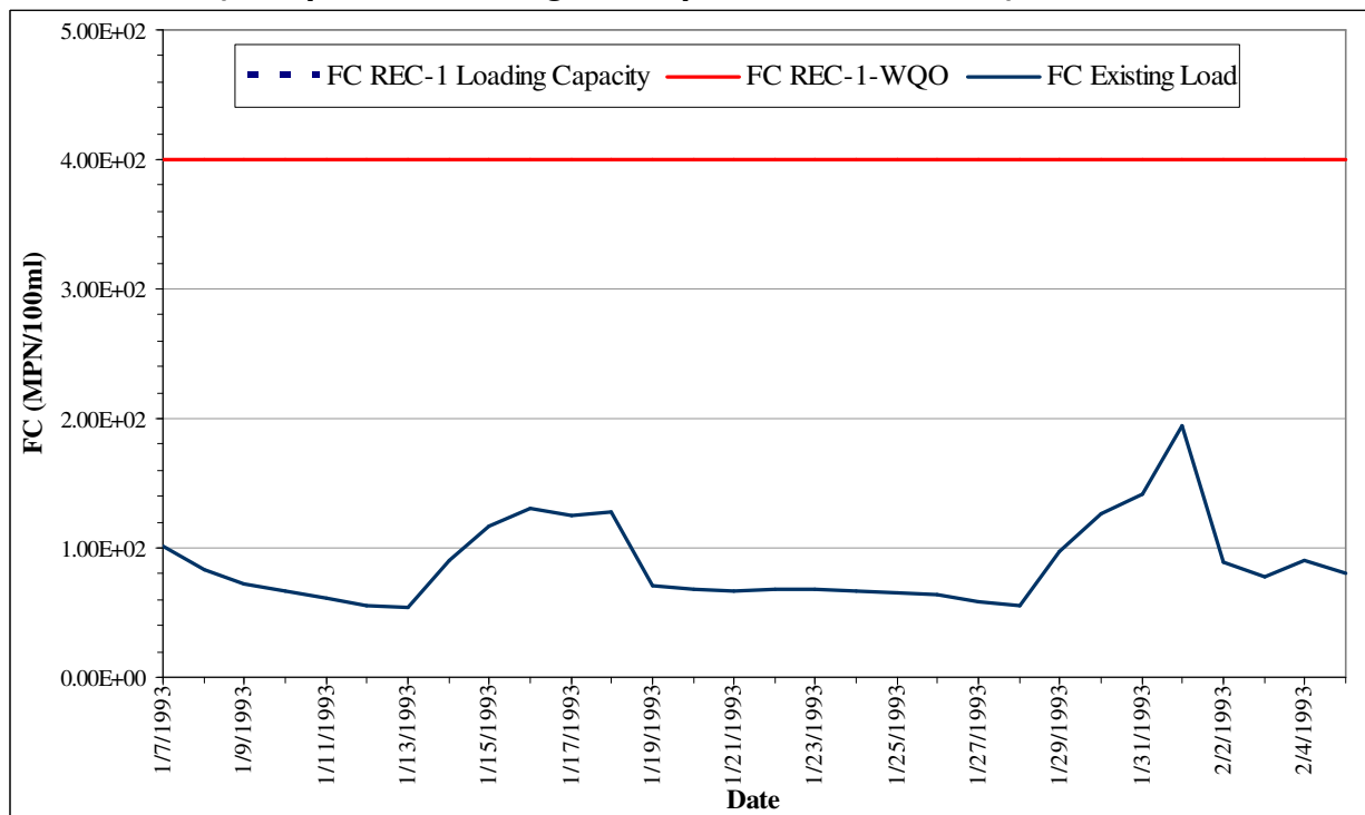
Figure H-2. Existing and Reduced Fecal Coliform Concentrations at Shelter Island Shoreline Park, San Diego Bay-Wet Weather (Comparison to Single Sample Maximum WQO)
