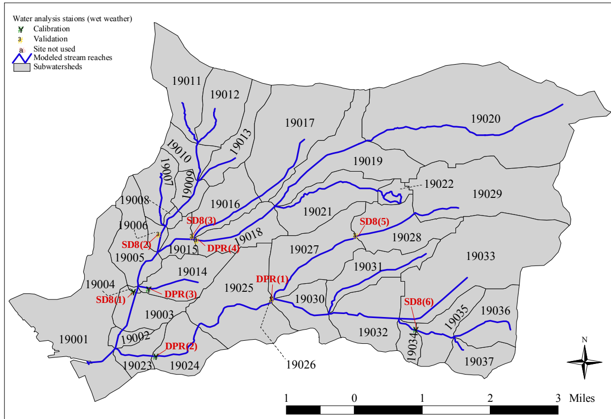
Figure 15. Map of monitoring locations used for model calibration and validation of the wet weather model.
