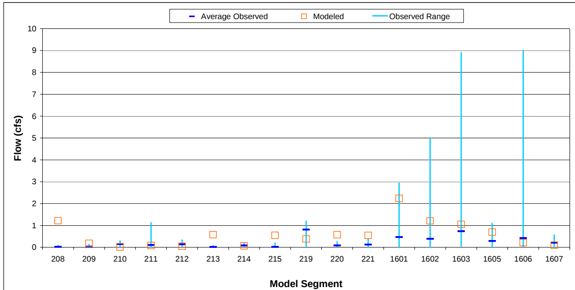
Figure 6. Calibration results of modeled versus observed flow. Model segment numbers are from the San Diego regional hydrologic model. (Tetra Tech, Inc., 2004)
