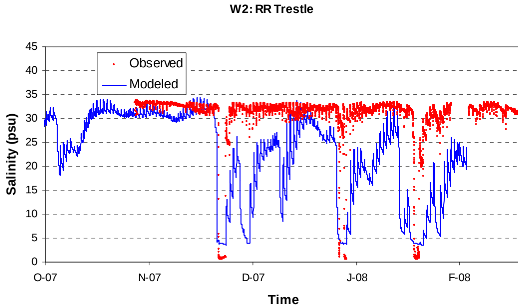
Figure 45. Salinity Calibration results for all stations (including Station W2)
