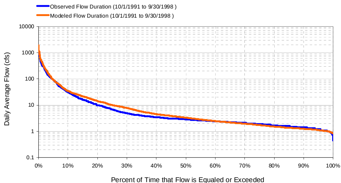
Figure 27. Flow exceedence output comparison – calibration period
