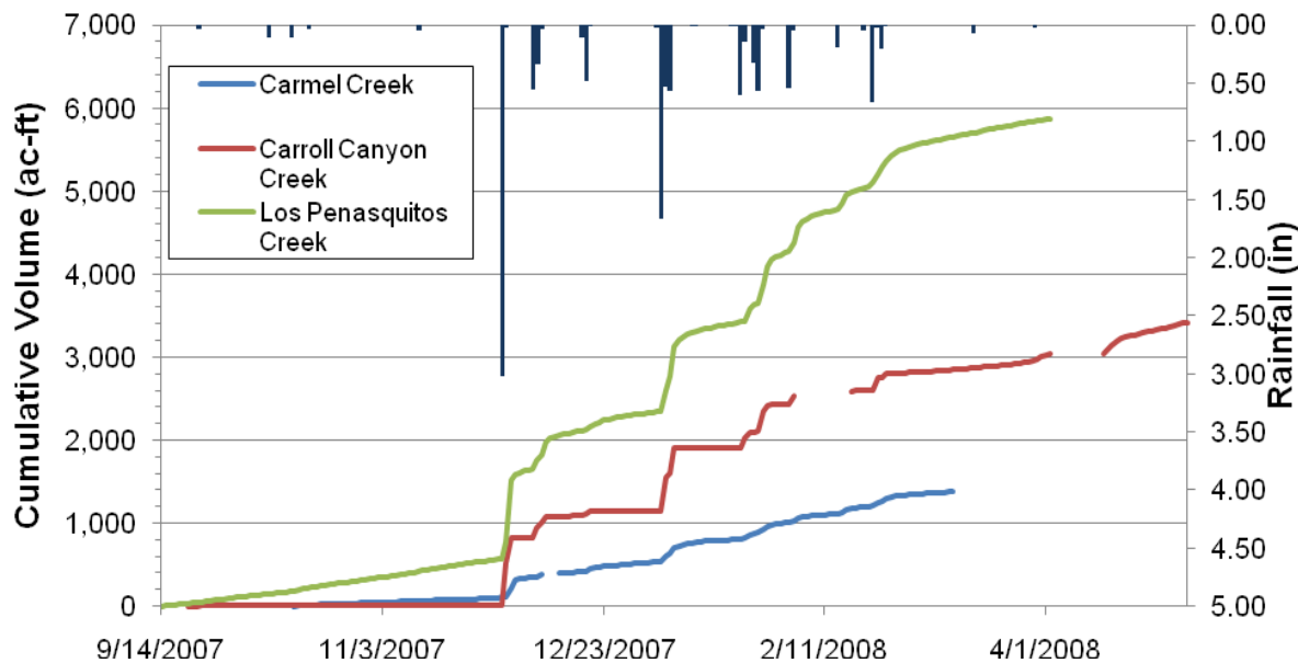
Figure 9. Cumulative volumes at TMDL monitoring locations
