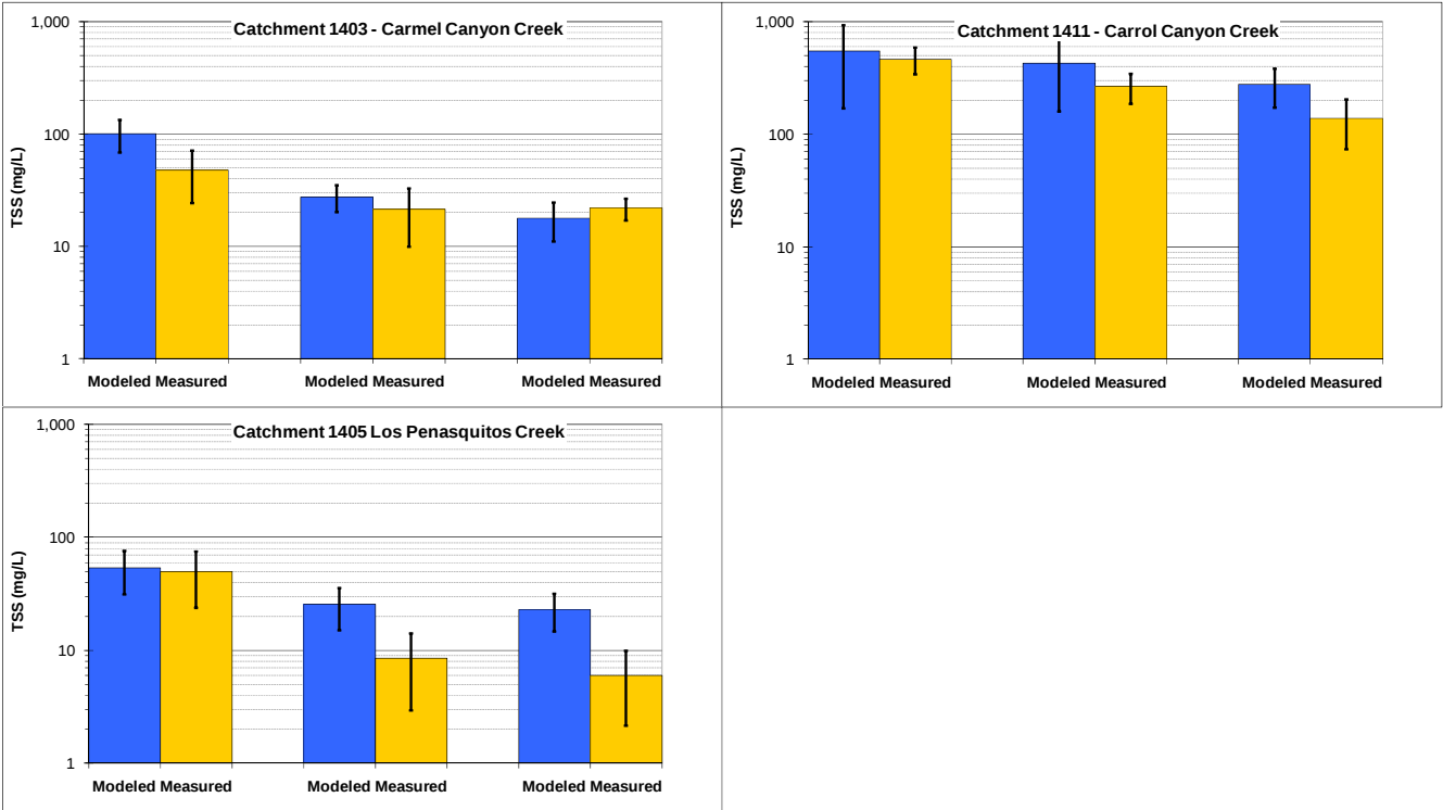
Figure 36. Comparison of EMC and 95 th Percentile TSS data collected during each storm event
