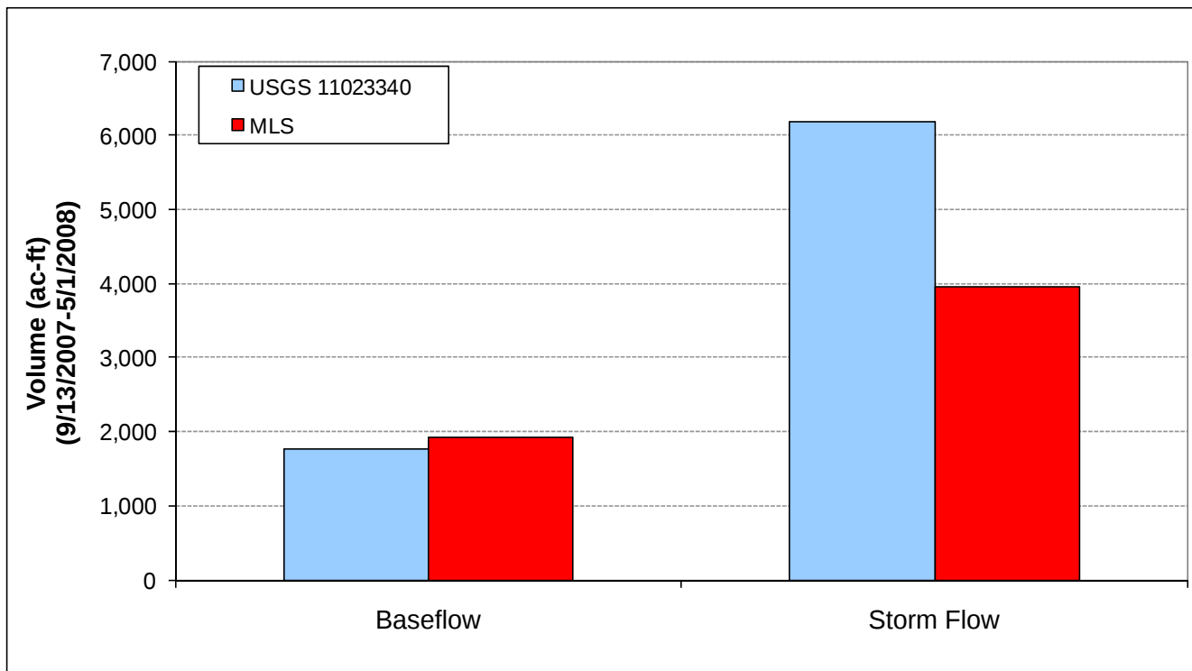
Figure 32. Baseflow and storm volumes measured on Los Peñasquitos Creek
