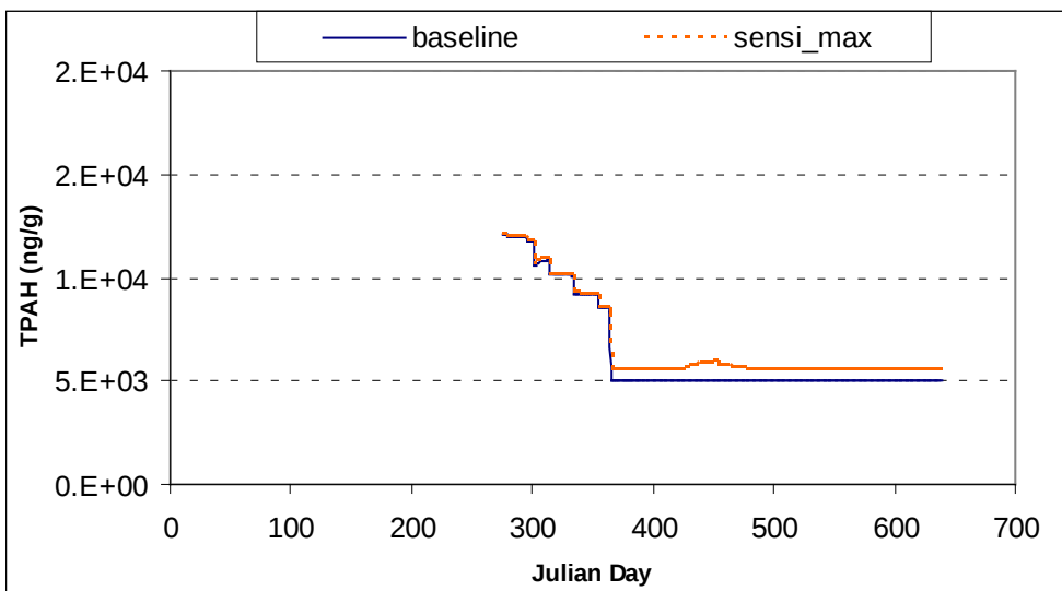
Figure E-1. Comparison of TPAH concentrations at the Paleta Creek mouth for the baseline and sensitivity runs.
