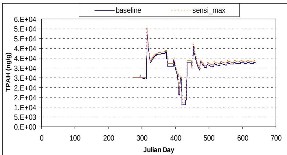
Figure E-2. Comparison of TPAH concentrations at the Chollas Creek mouth for the baseline and sensitivity runs.
