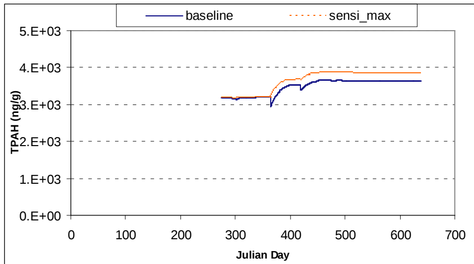
Figure E-5. Comparison of TPAH concentrations at the Downtown Anchorage mouth for the baseline and sensitivity runs.
