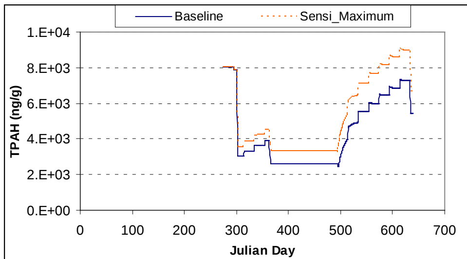
Figure E-3. Comparison of TPAH concentrations at the Switzer Creek mouth for the baseline and sensitivity runs.
