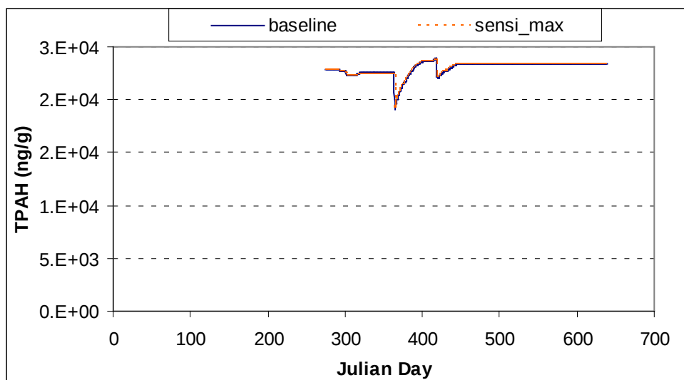
Figure E-4. Comparison of TPAH concentrations at the B-Street mouth for baseline and sensitivity runs.
