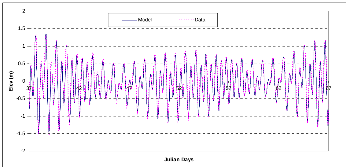
Figure A-1. Calibration results for the San Diego Bay hydrodynamic model.
