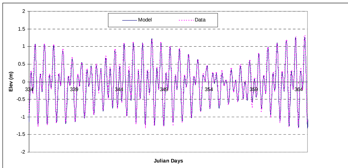
Figure A-4. Extended comparison (validation) of San Diego Bay hydrodynamic model results and data (December 2001).
