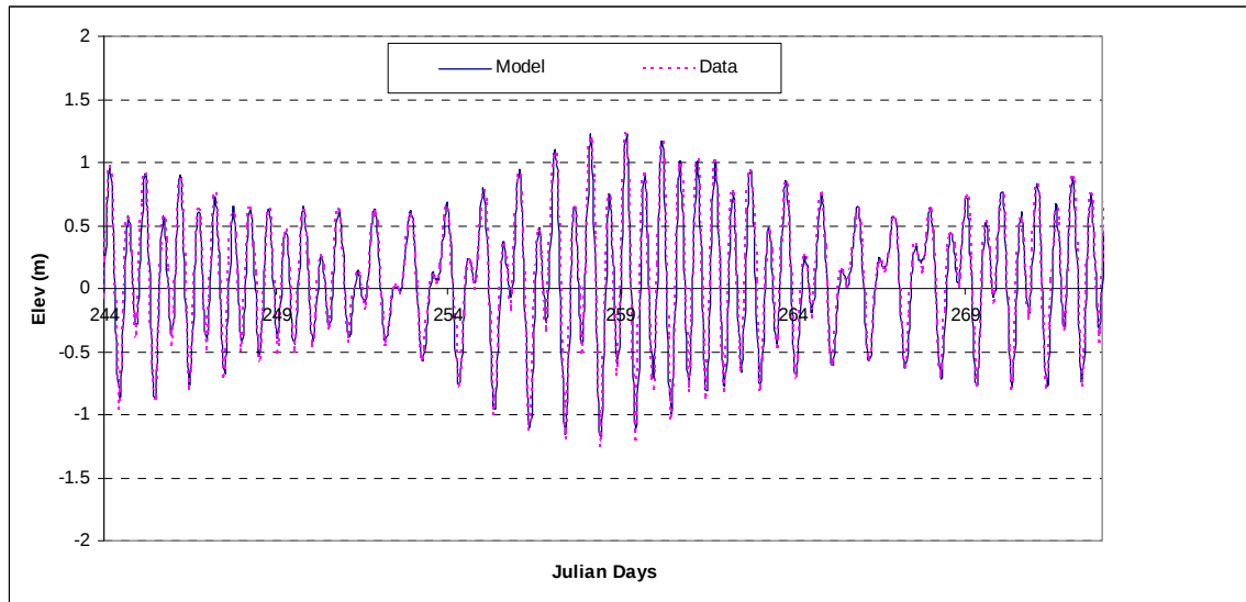
Figure A-3. Extended comparison (validation) of the San Diego Bay hydrodynamic model results and data (September 2001).
