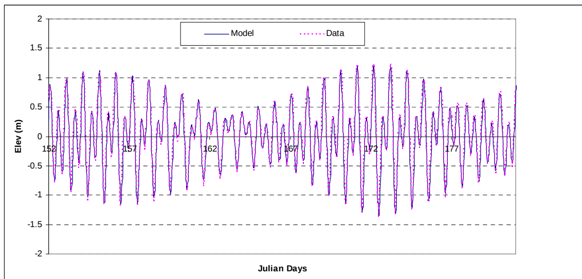
Figure A-2. Extended comparison (validation) of the San Diego Bay hydrodynamic model results and data (June 2001).
