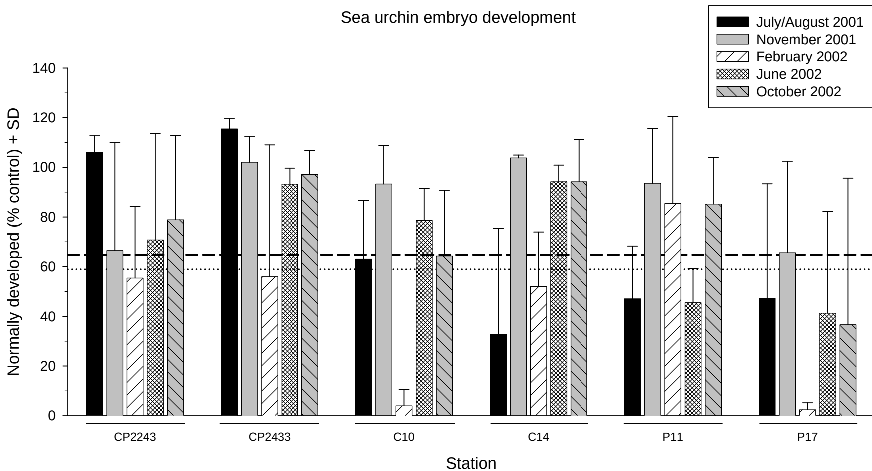
Figure 15. Sea urchin embryo development in quarterly sediment-water interface samples. Data are control adjusted. The dashed line is the lower 95% prediction limit from the Baseline Pool. The dotted line is the 59% normal development threshold.
