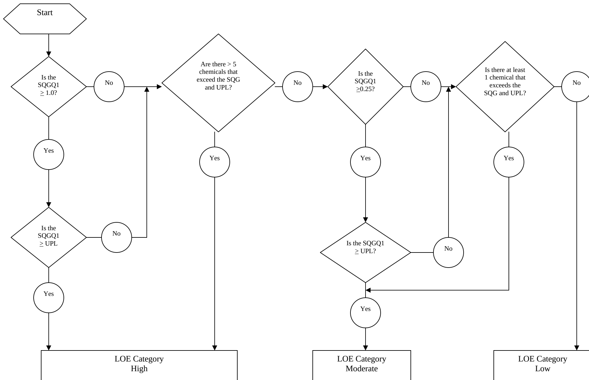
Figure 21. Sediment chemistry Lines of Evidence flow chart.
