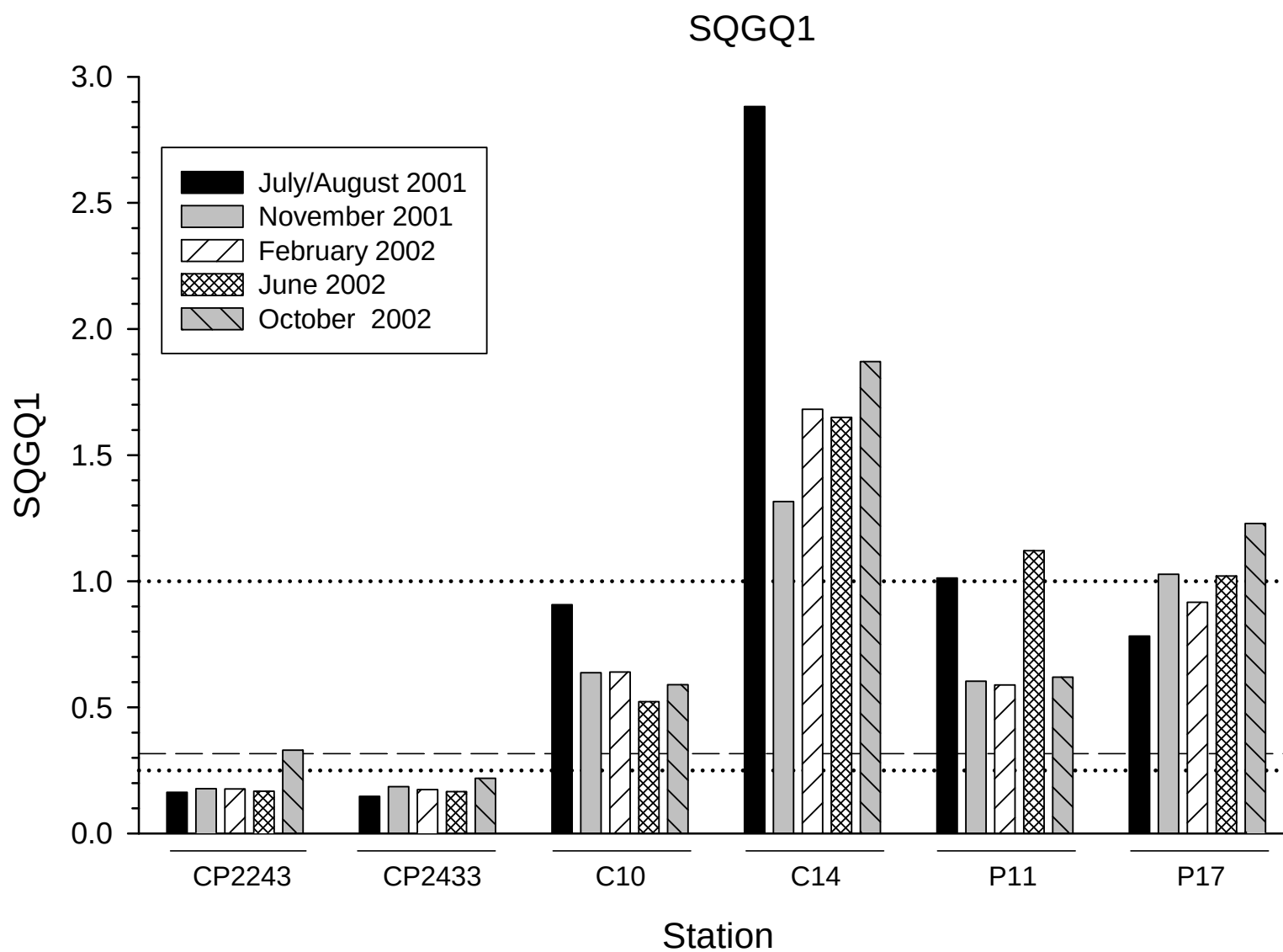
Figure 13. Sediment Quality Guideline Quotient (SQGQ1) in quarterly sediment samples. The dashed line is the 95% prediction limit from the Baseline Pool. The dotted lines represent the thresholds that correspond with unlikely (lower line) and likely (upper line) acute toxicity to amphipods.
