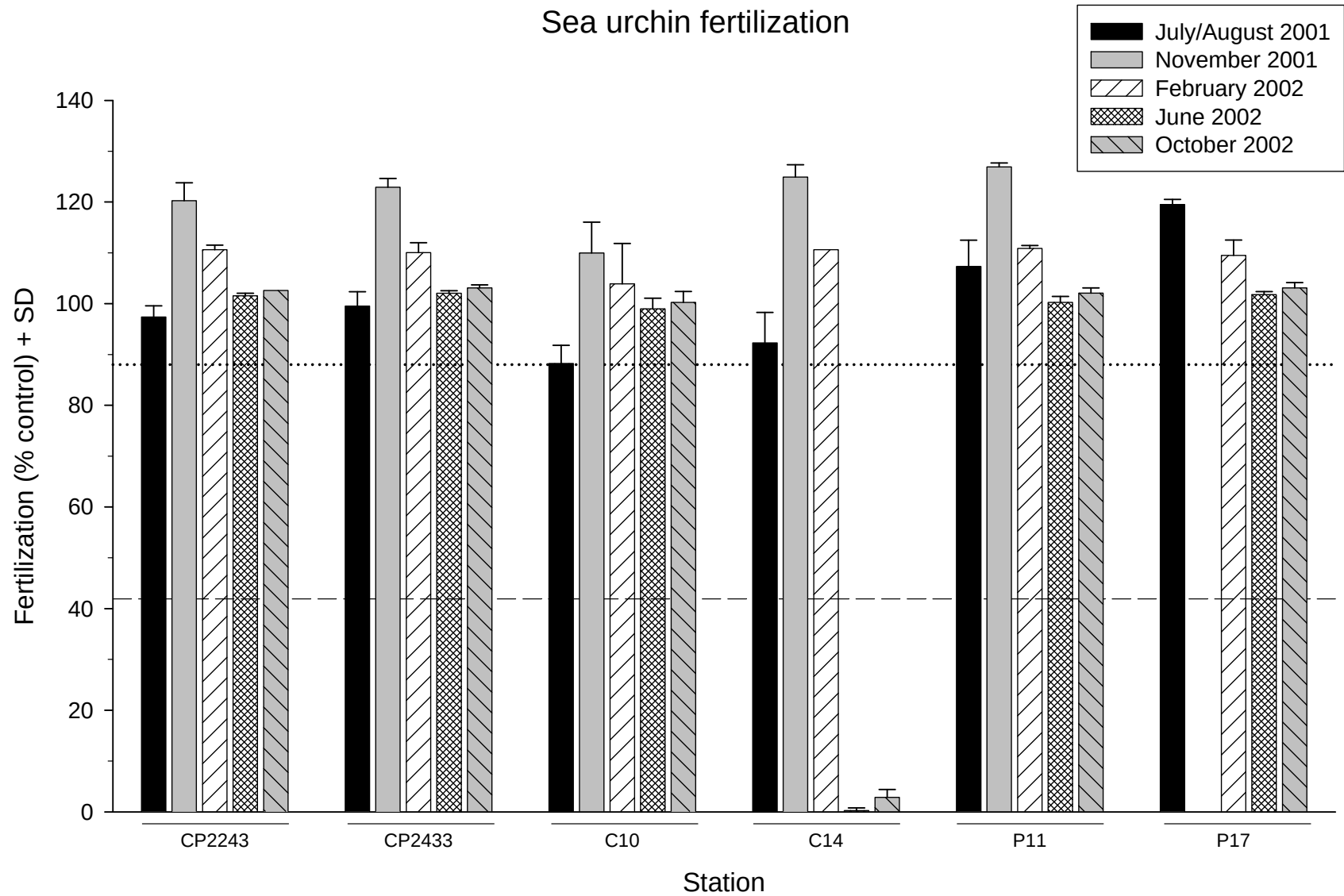
Figure 16. Sea urchin fertilization in quarterly pore water samples. Data are control adjusted. The dotted line is the 88% development threshold. The dashed line is the lower 95% prediction limit from the Baseline Pool.
