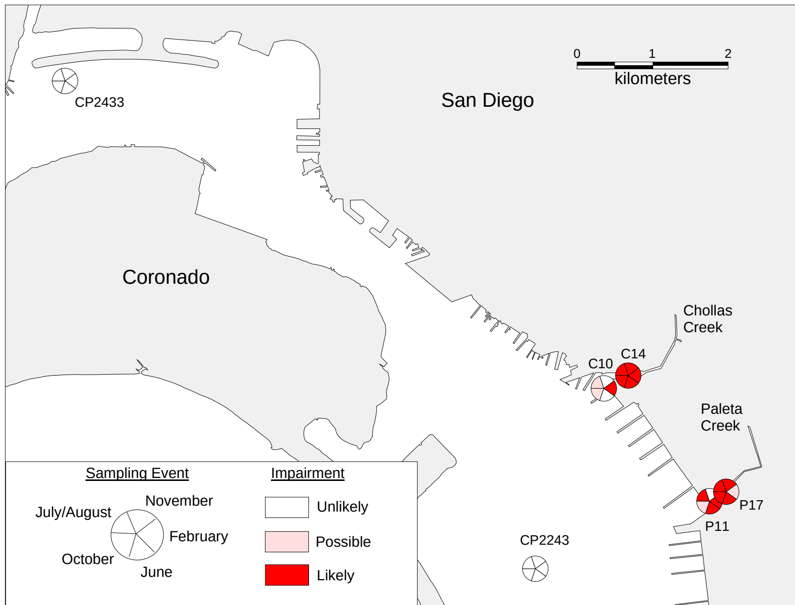
Figure 24. Aquatic life impairment weight of evidence for San Diego Bay temporal sampling study.
