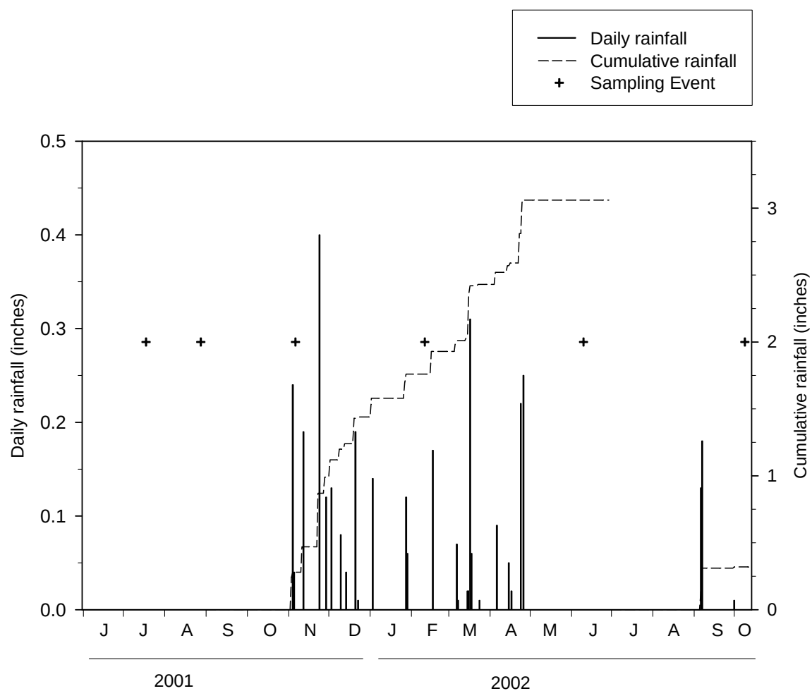
Figure 2. Rainfall amounts and seasonal totals during the quarterly sampling events. The 2001-2002 season was the driest on record, with only 28% of the normal total rainfall.
