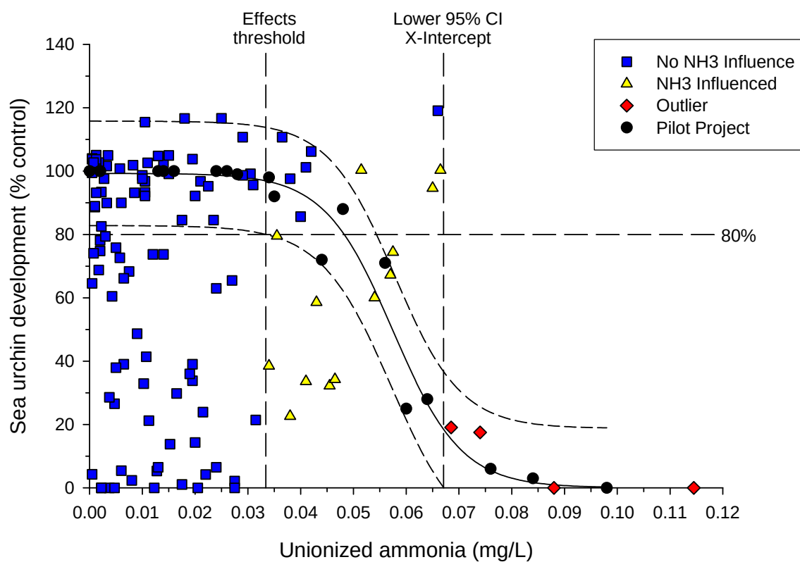
Figure C3. Adjusted sea urchin embryo development results that exclude the effect of ammonia for the NH 3 influenced samples.
