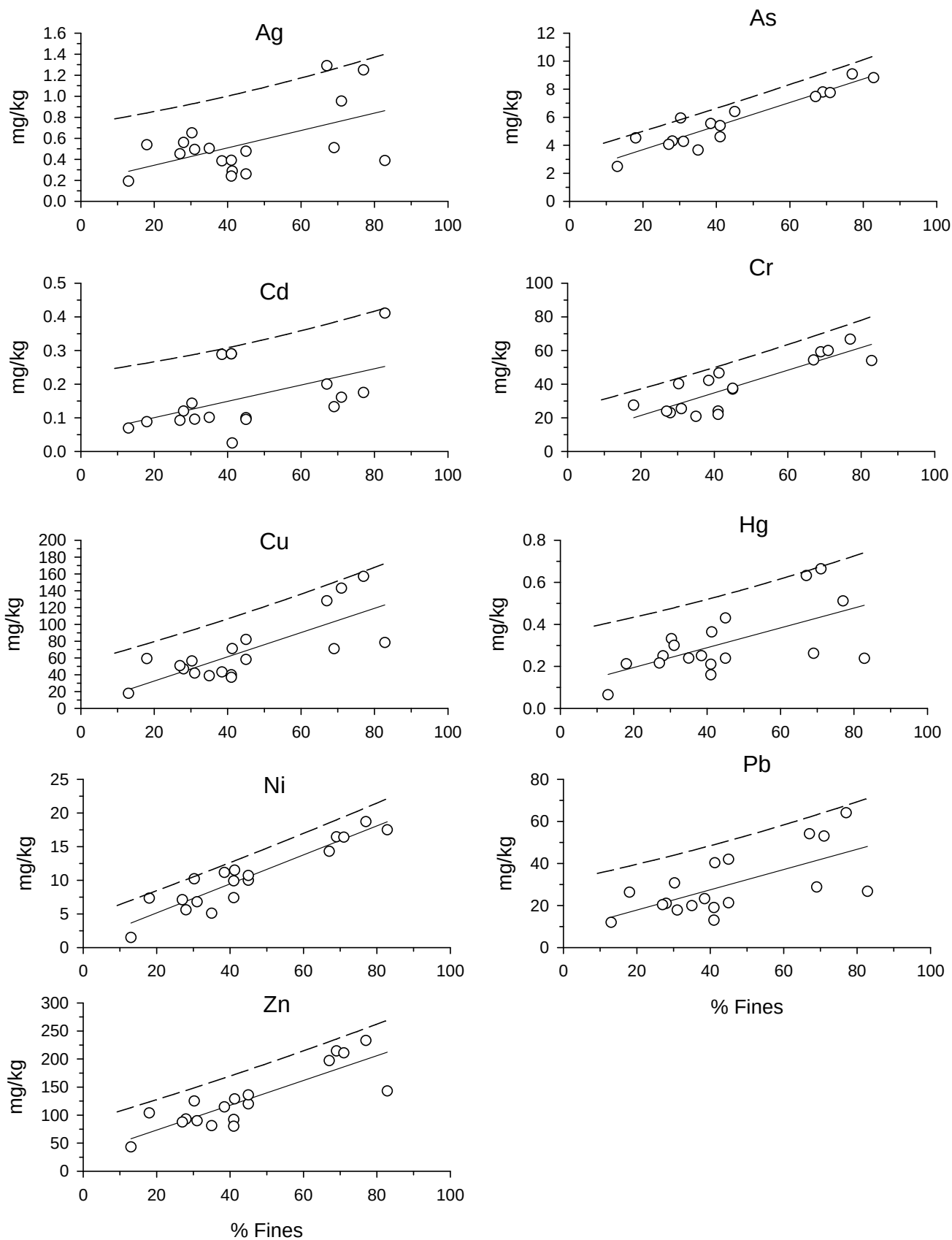
Figure B1. % Fines:metals plots from the Baseline Pool. The solid line is the relationship from linear regression. The dashed line is the threshold (predicted value + 95% prediction interval).
