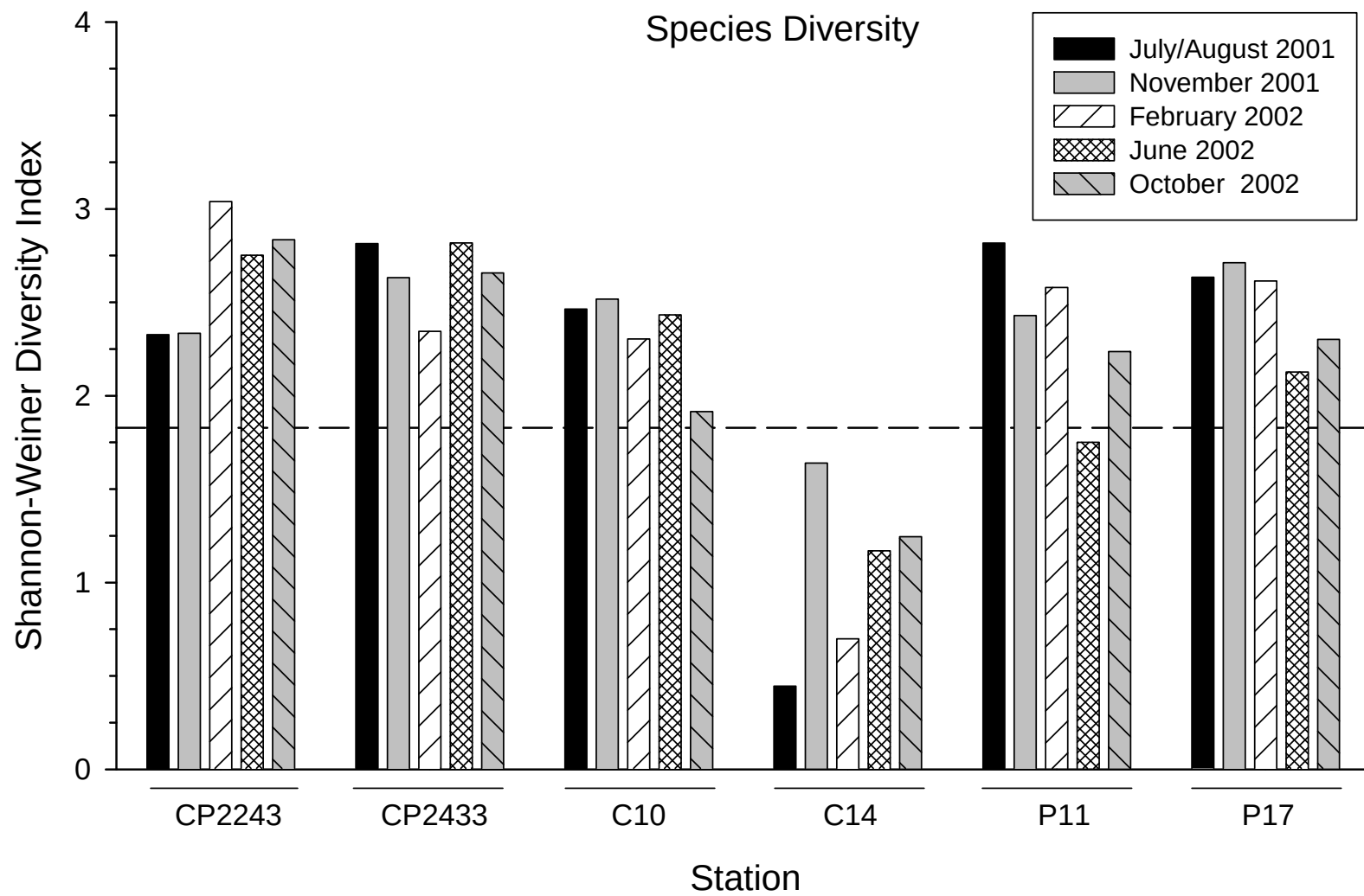
Figure 19. Diversity of benthic macrofauna at each station in the quarterly samples. The dashed line is the 95% prediction limit from the Baseline Pool.
