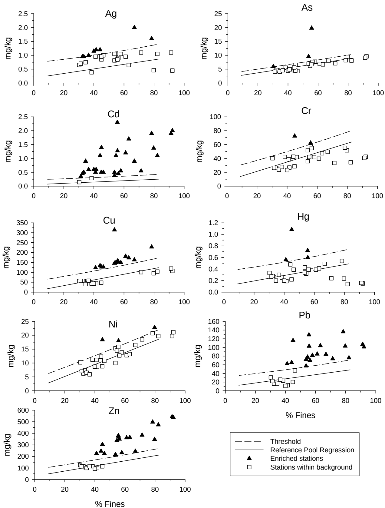
Figure B2. %Fines:metals plots from Chollas and Paleta Creek stations overlaid on the threshold and regression lines from the Baseline Pool. Sites which fall below the threshold are considered uncontaminated. Sites which lie above the threshold are considered enriched.
