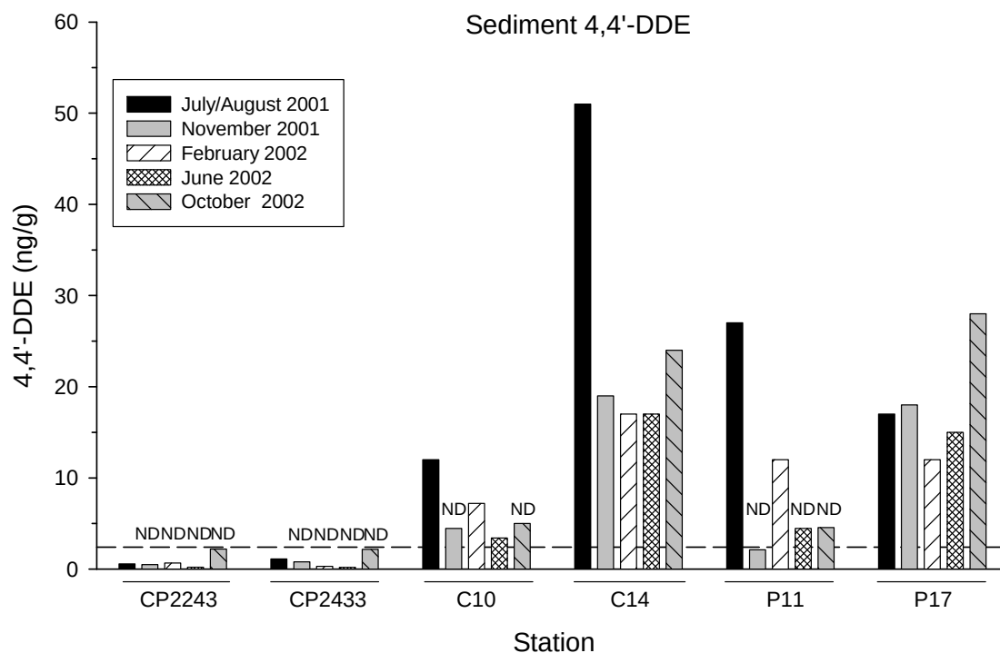
Figure 11. Concentrations of 4,4'-DDT and 4,4'-DDE in the quarterly sediment samples. The dashed line is the 95% prediction limit from the Baseline Pool. ND = not detected. The method detection limit varied by DDT isomer, and by analysis.
