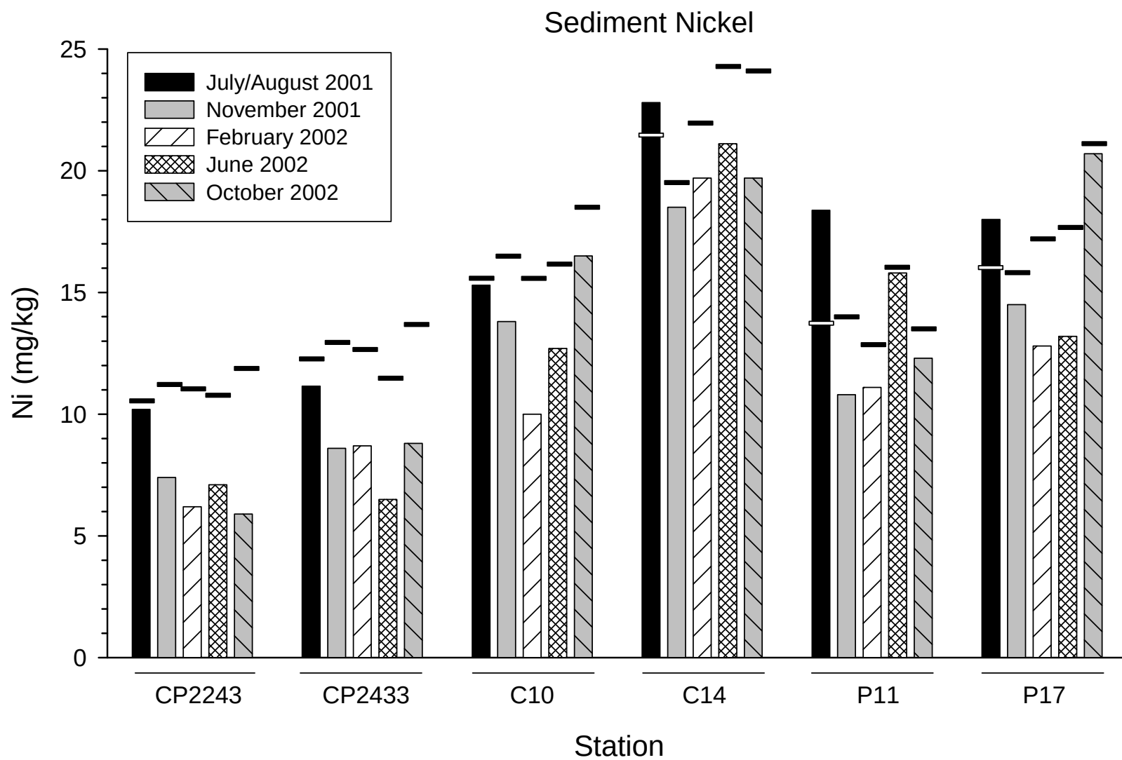
Figure 7. Concentrations of nickel in the quarterly sediment samples. The dashes are threshold values calculated from the Baseline Pool using metals:%fines regression analysis. The ERM for Ni (not shown) is 51.6 mg/kg.
