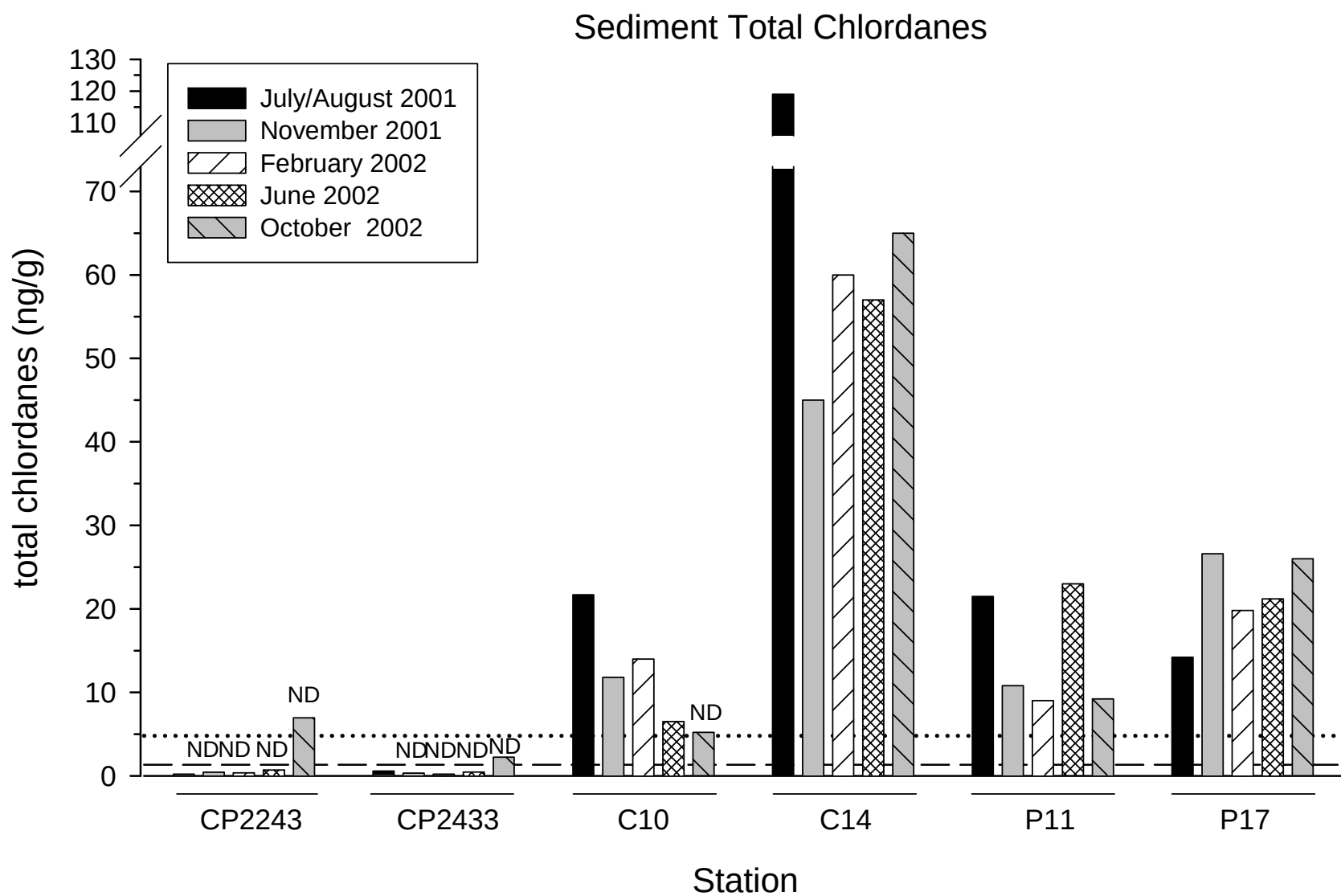
Figure 12. Concentrations of total chlordanes in the quarterly sediment samples. ND = non-detect treated as equal to half the method detection limit, which varied by analysis. The dashed line is the 95% prediction limit from the Baseline Pool. The dotted line is the PEL.
