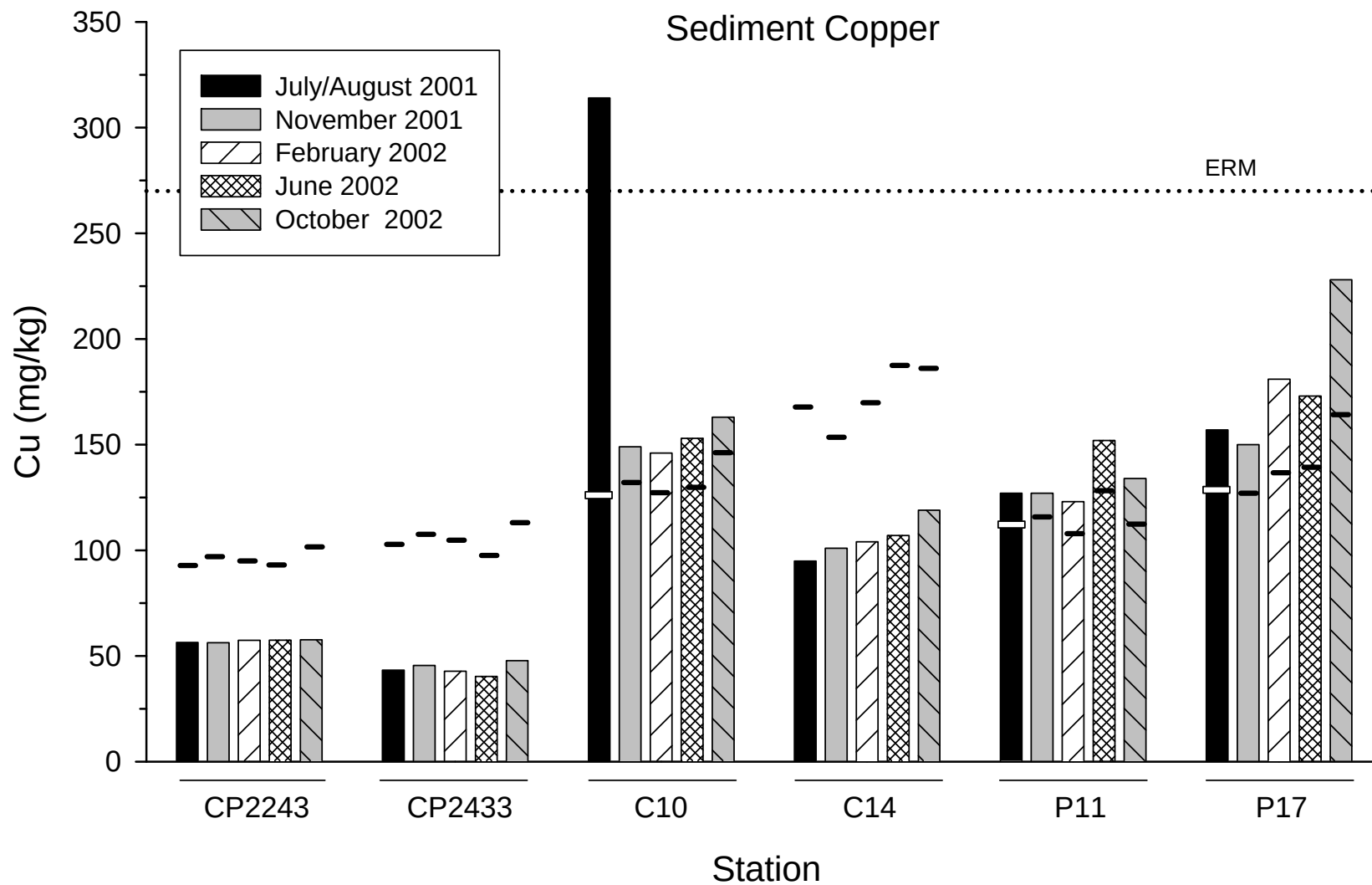
Figure 5. Concentrations of copper in the quarterly sediment samples. The dashes are threshold values calculated from the Baseline Pool using metals:%fines regression analysis. The dotted line is the ERM.
