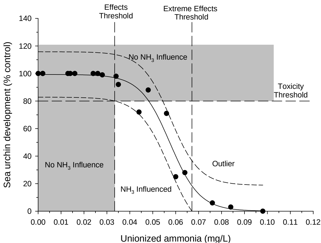
Figure C1. Effect of unionized ammonia on sea urchin embryo development. The plotted points are from experiments using seawater spiked with various concentrations of ammonia. The three categories (No NH 3 influence, NH 3 influenced, Outlier) reflect the concentration of unionized ammonia and level of normal embryo development observed.
