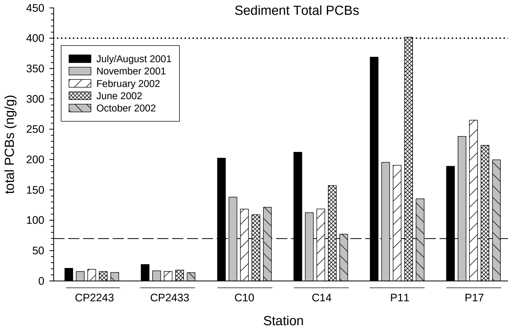
Figure 10. Concentrations of total PCBs in the quarterly sediment samples. The dashed line is the 95% prediction limit from the Baseline Pool. The dotted line is the consensus-based guideline for total PCBs.
