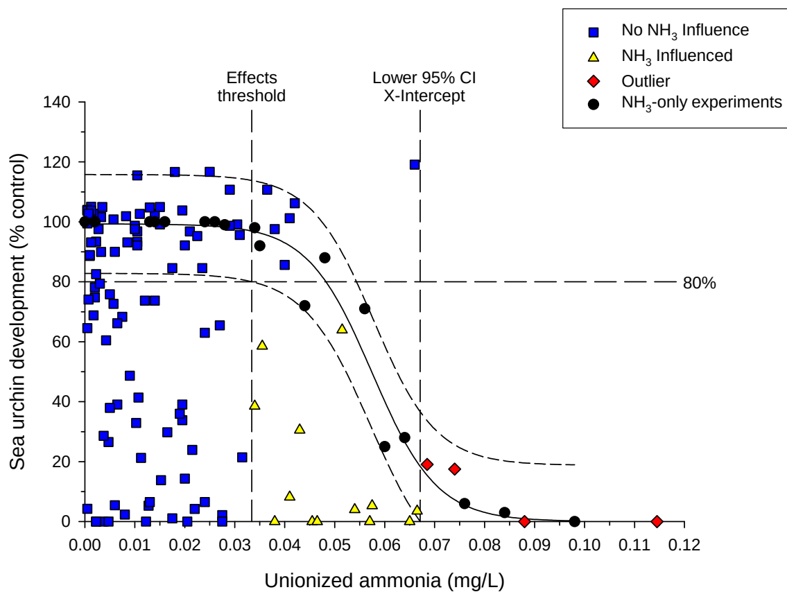
Figure C2. Sea urchin embryo development and unionized ammonia concentrations from Chollas and Paleta Creek stations, the San Diego Bay reference sites, and ammonia-only experiments. The San Diego Bay samples are categorized by influence of ammonia.
