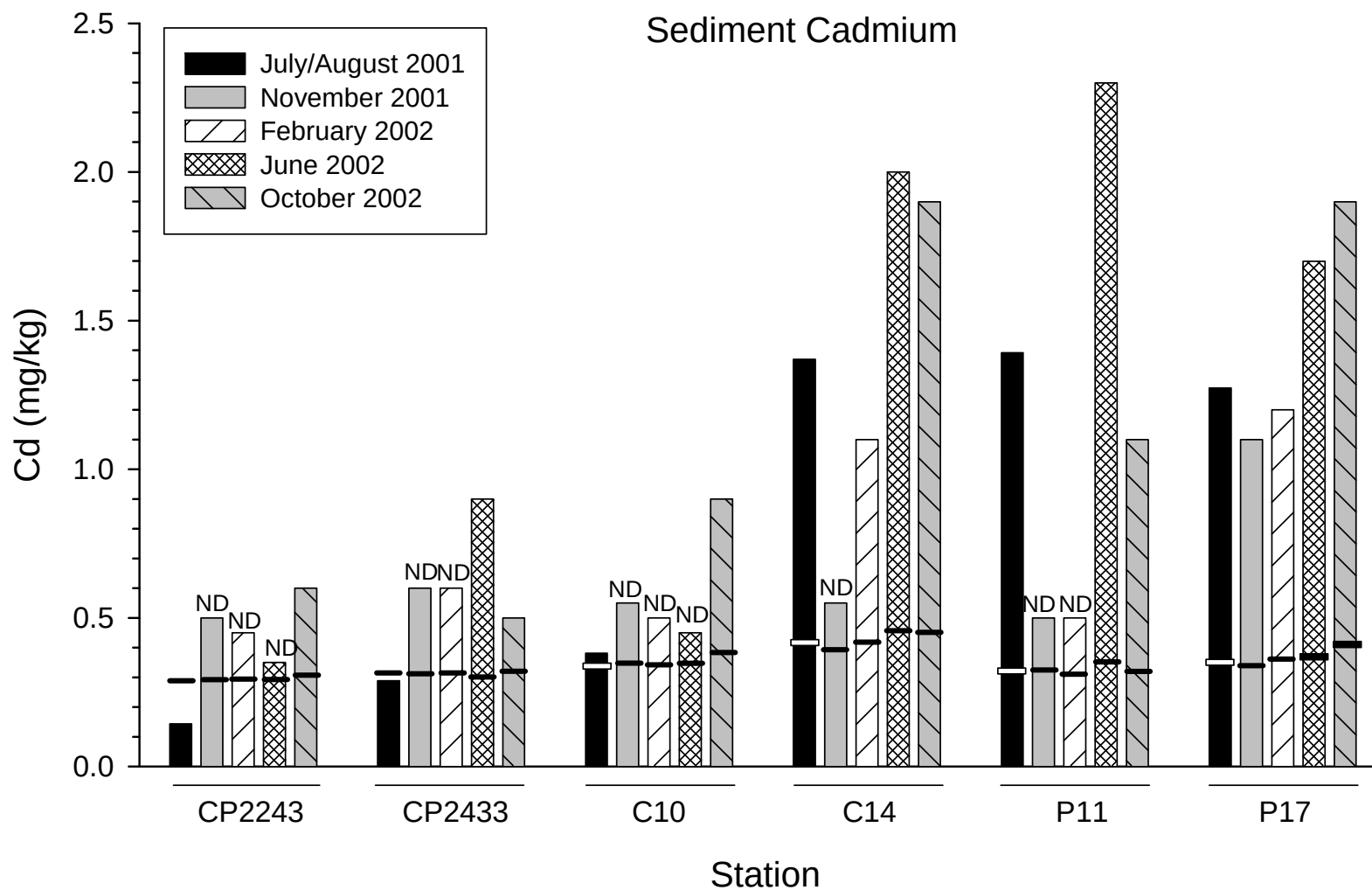
Figure 3. Concentrations of cadmium in quarterly sediment samples. ND = non-detect treated as equal to half the reporting level, which varied by analysis. The dashes are threshold values calculated from the Baseline Pool using metals:%fines regression analysis. The ERM for Cd (not shown) is 9.6 mg/kg.
