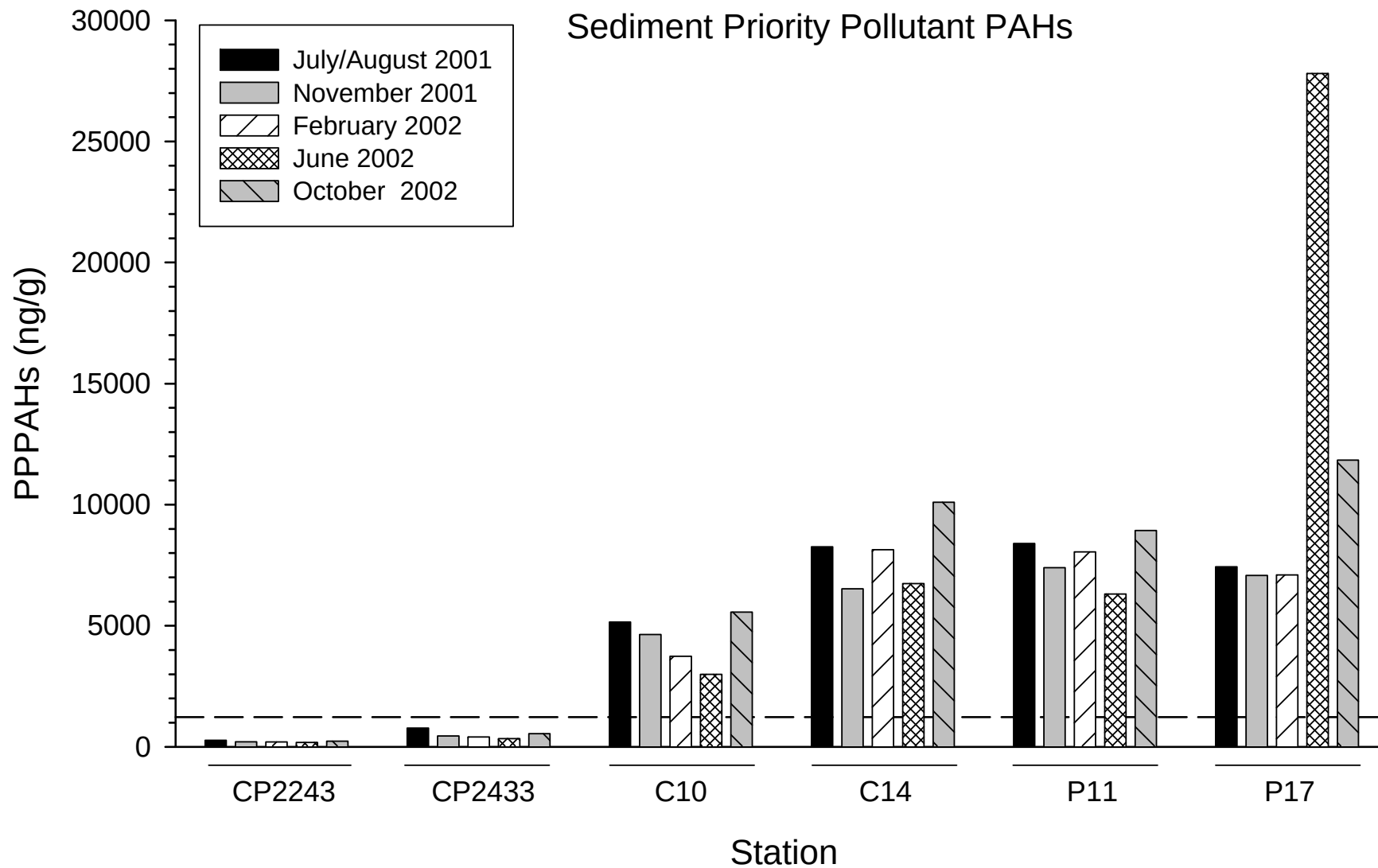
Figure 9. Concentrations of priority pollutant PAHs in the quarterly sediment samples. The dashed line is the 95% prediction limit from the Baseline Pool.
