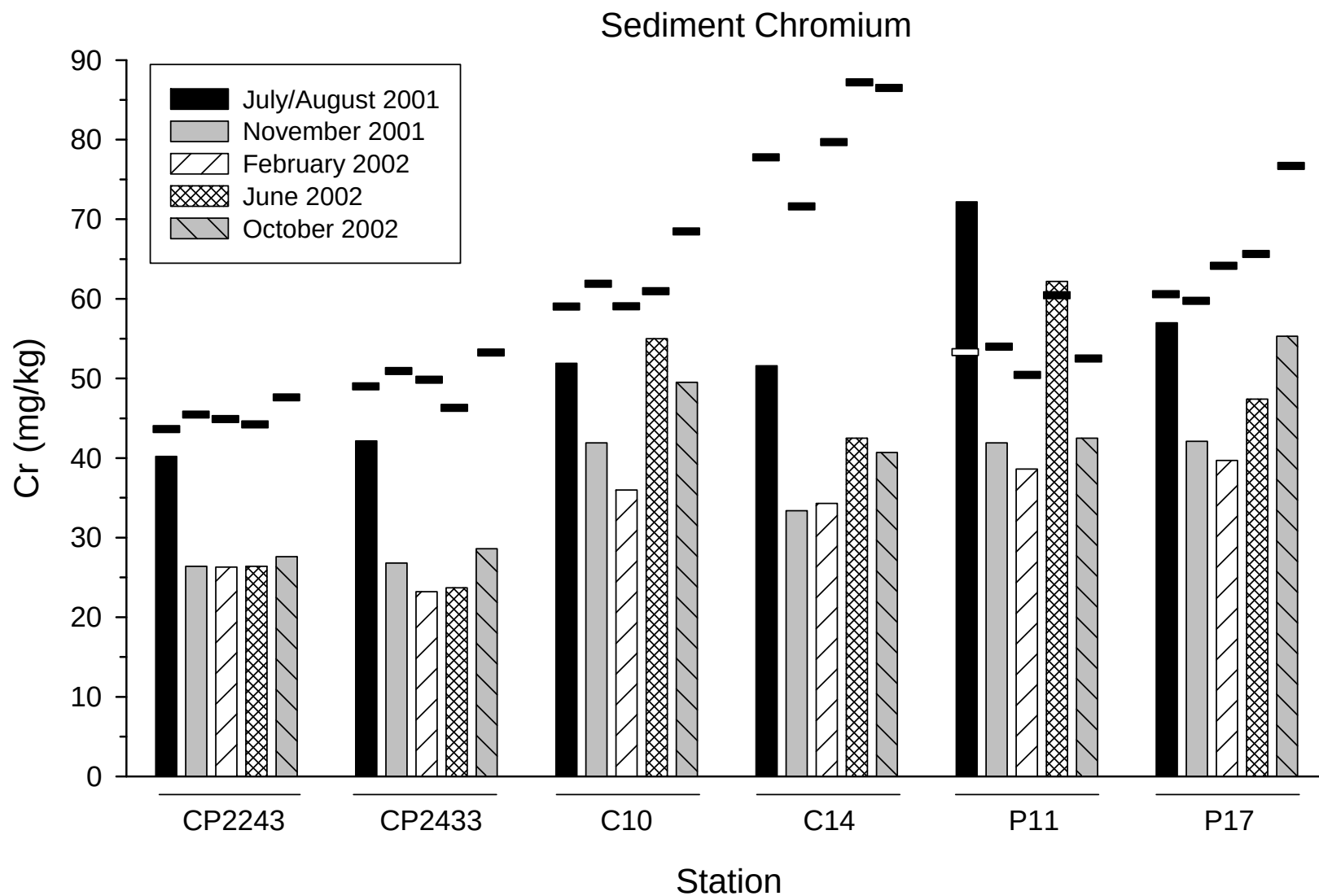
Figure 4. Concentrations of chromium in the quarterly sediment samples. The dashes are threshold values calculated from the Baseline Pool using metals:%fines regression analysis. The ERM for Cr (not shown) is 370 mg/kg.
