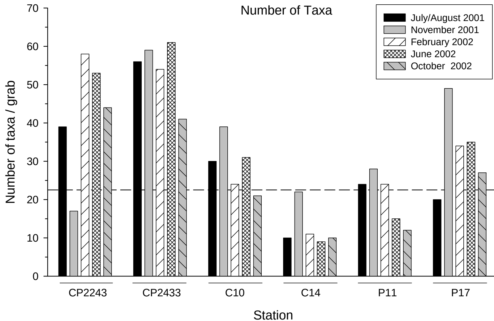
Figure 18. Number of macrofauna taxa at each station in the quarterly samples. The dashed line is the 95% prediction limit from the Baseline Pool.
