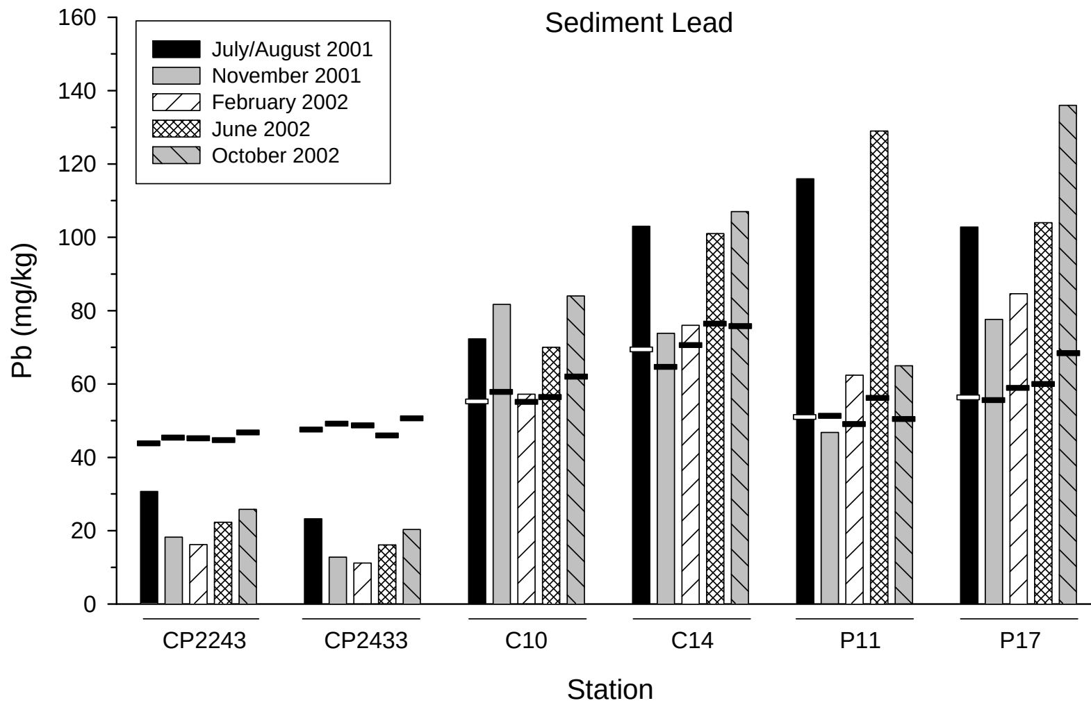
Figure 6. Concentrations of lead in the quarterly sediment samples. The dashes are threshold values calculated from the Baseline Pool using metals:%fines regression analysis. The ERM for Pb (not shown) is 218 mg/kg.
