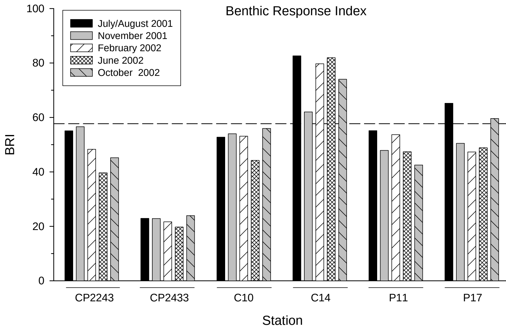
Figure 20. Benthic Response Index at each station in the quarterly samples. The dashed line is the 95% prediction limit from the Baseline Pool.
