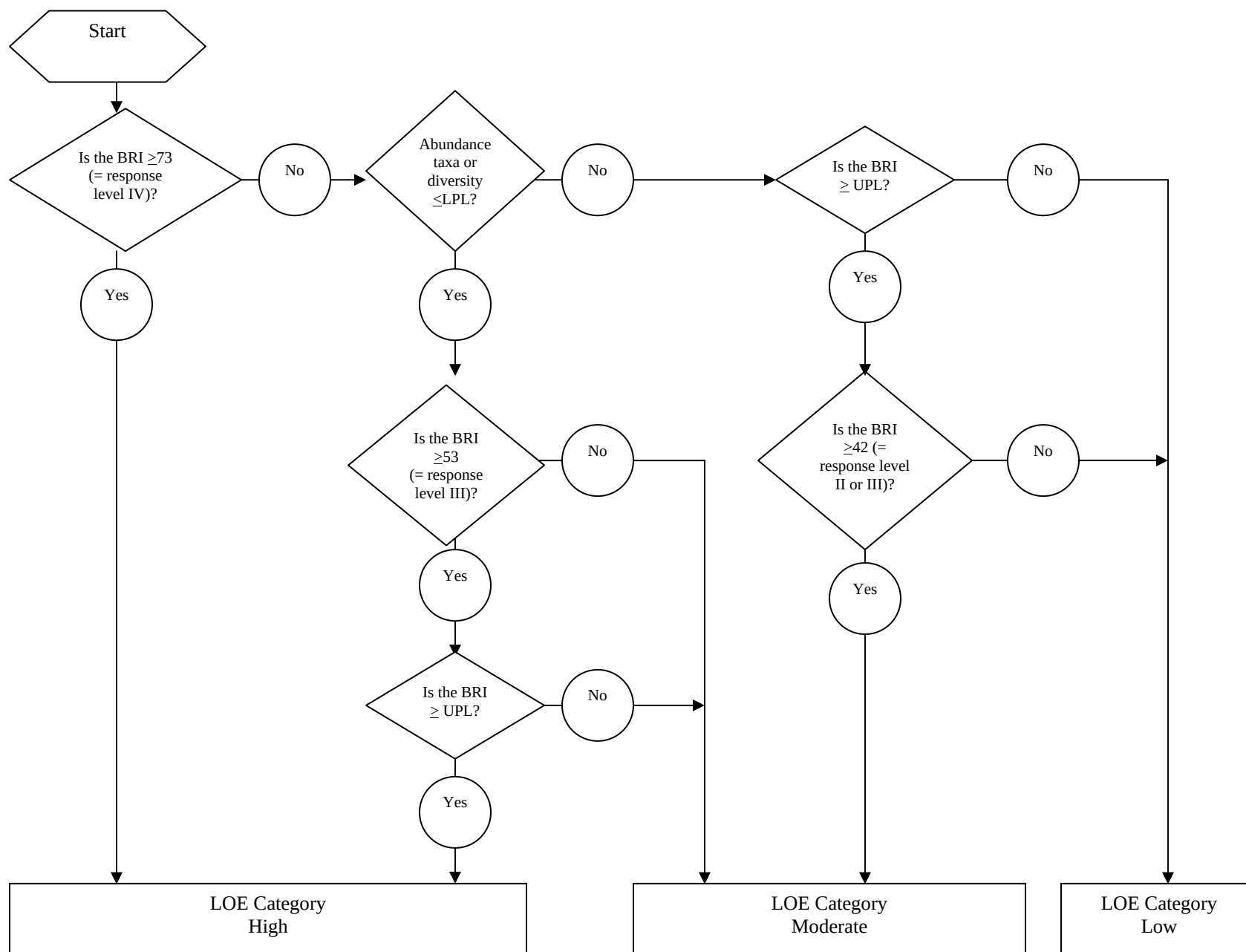
Figure 22. Benthic community Lines of Evidence flow chart.
