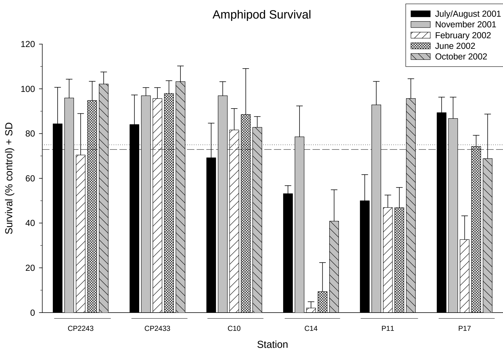
Figure 14. Amphipod survival in quarterly bulk sediment samples. Data are control adjusted. The dotted line is the 75% survival threshold. The dashed line is the lower 95% prediction limit from the Baseline Pool.
