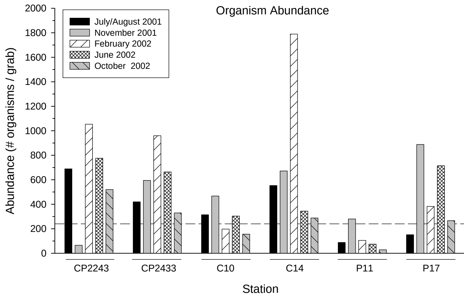
Figure 17. Macrofauna organism abundance in the quarterly samples. The dashed line is the lower 95% prediction limit from the Baseline Pool.
