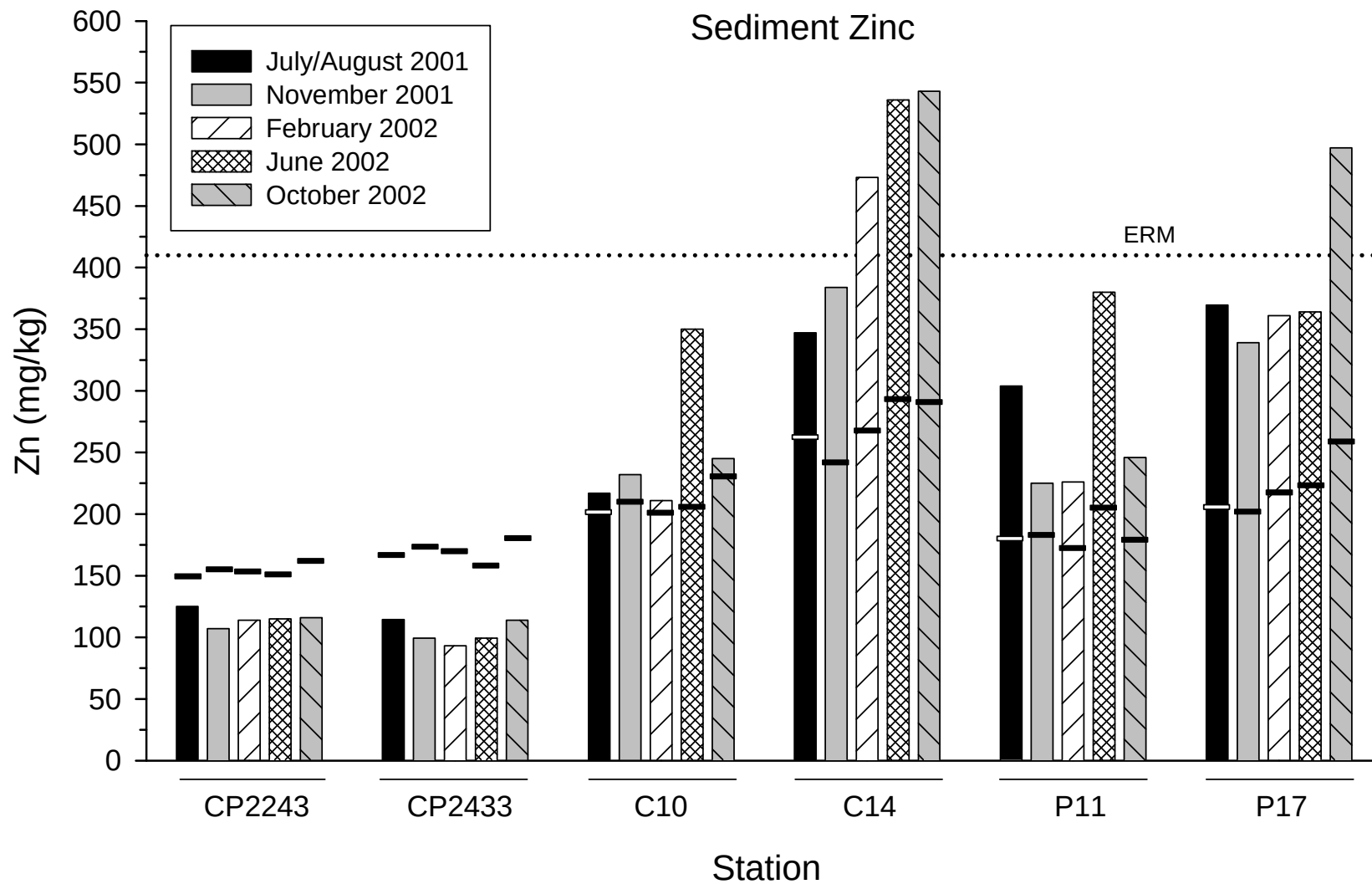
Figure 8. Concentrations of zinc in the quarterly sediment samples. The dashes are threshold values calculated from the Baseline Pool using metals:%fines regression analysis.
