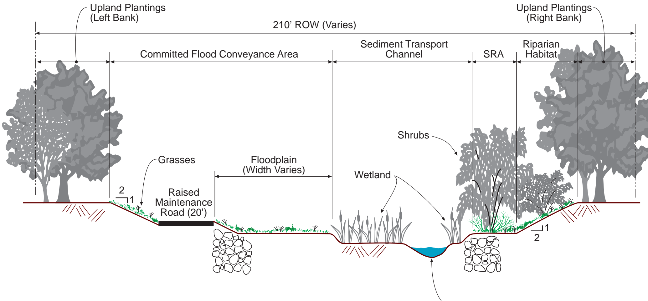
Reach 1A Typical Section Sta. 0+00 to 5+40 Length = 500' Earthen Channel Not To Scale
