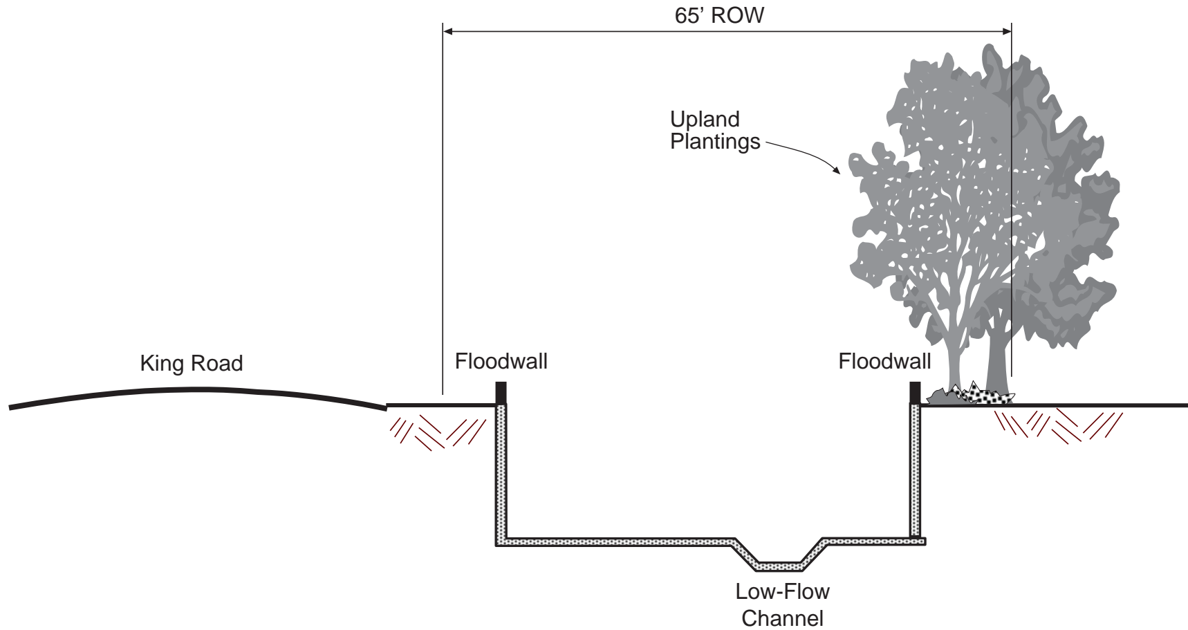
Reach 2 Typical Section Sta. 39+00 to 51+00 Length = 1200' Rectangular Concrete Channel Not To Scale
