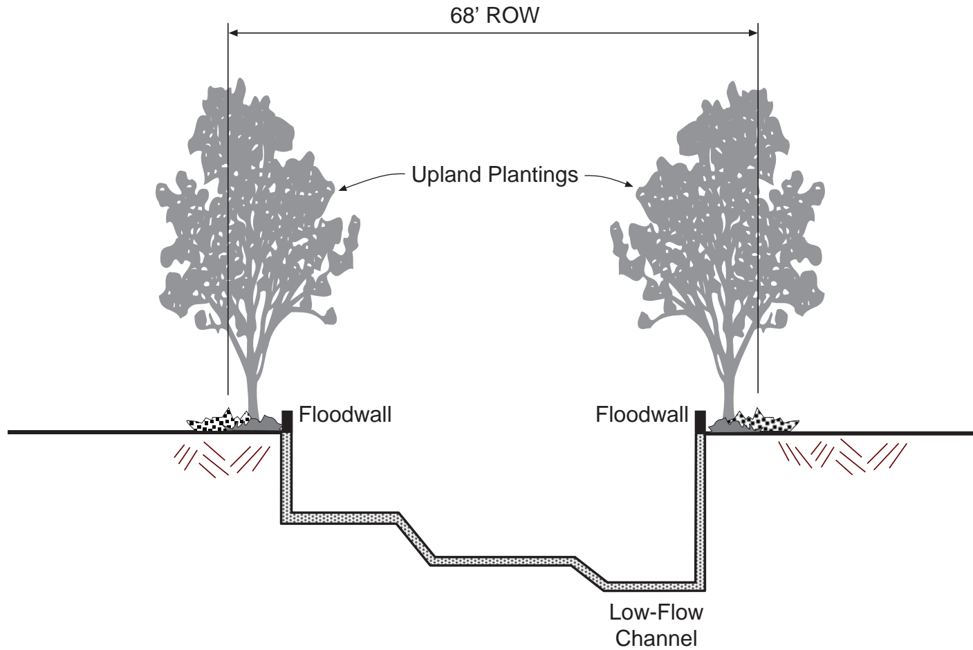
Reach 3B Typical Section Sta. 70+00 to 79+75 Length = 925' Concrete Channel Not To Scale
