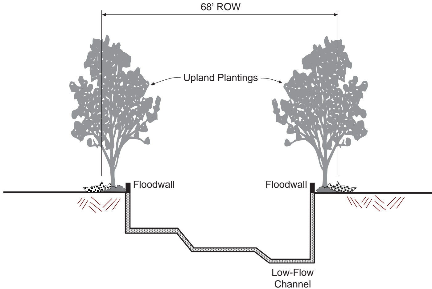
Reach 3C Typical Section Sta. 79+75 to 87+00 Length = 725' Concrete Channel Not To Scale
