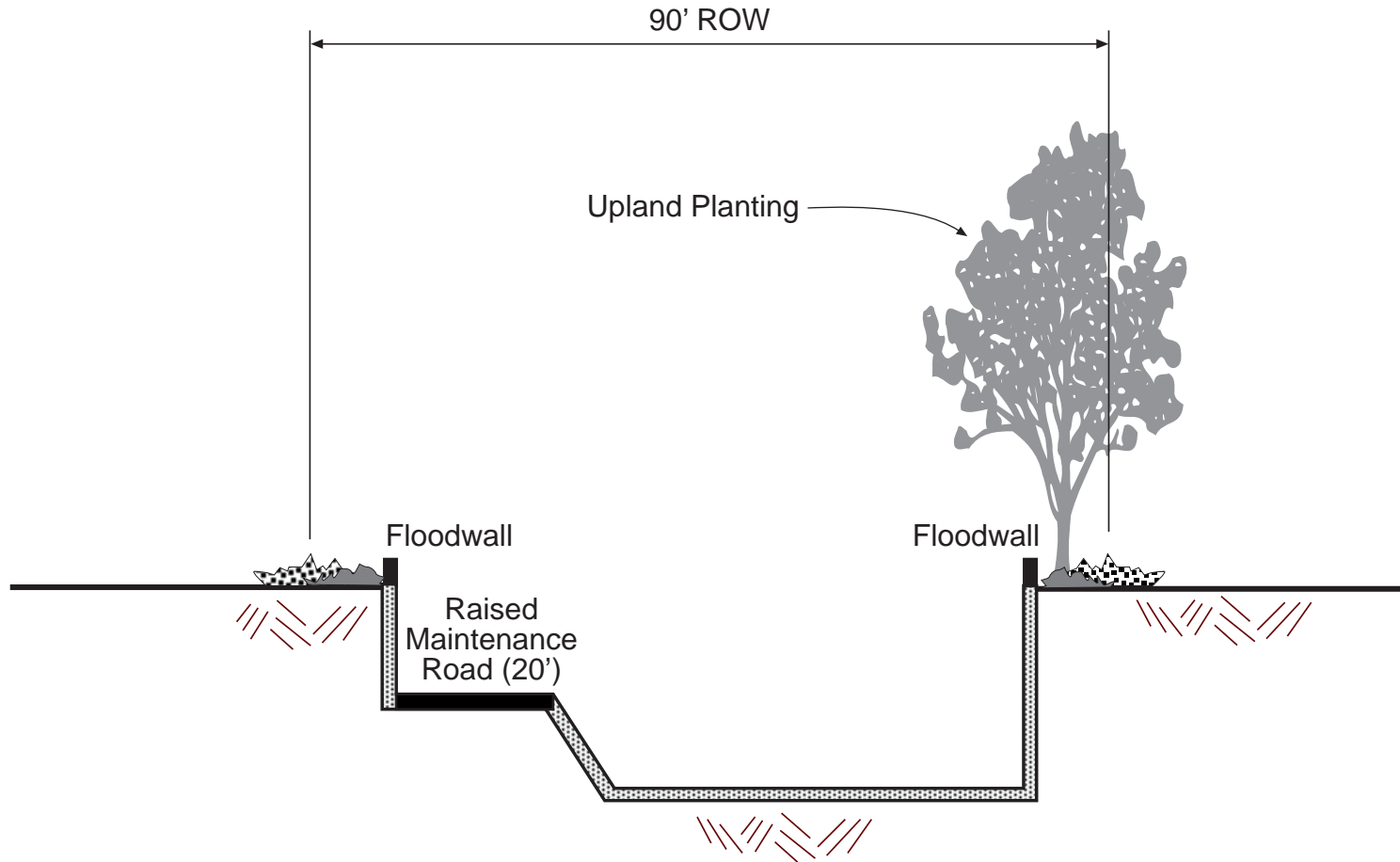
Reach 4A Typical Section Sta. 128+00 to 130+20 Length = 220' U-Frame Concrete Channel/Sediment Trap
