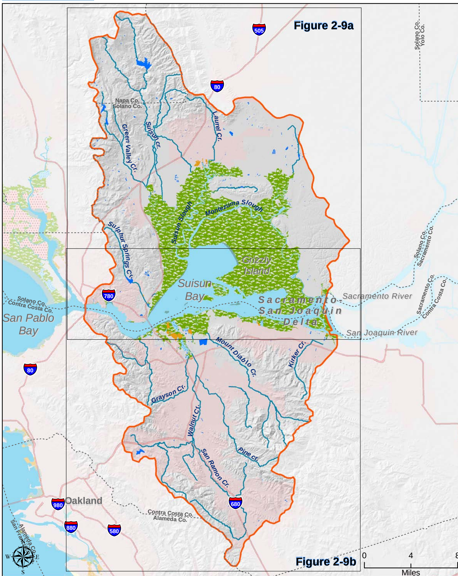
Figure 2-9 Suisun Basin
