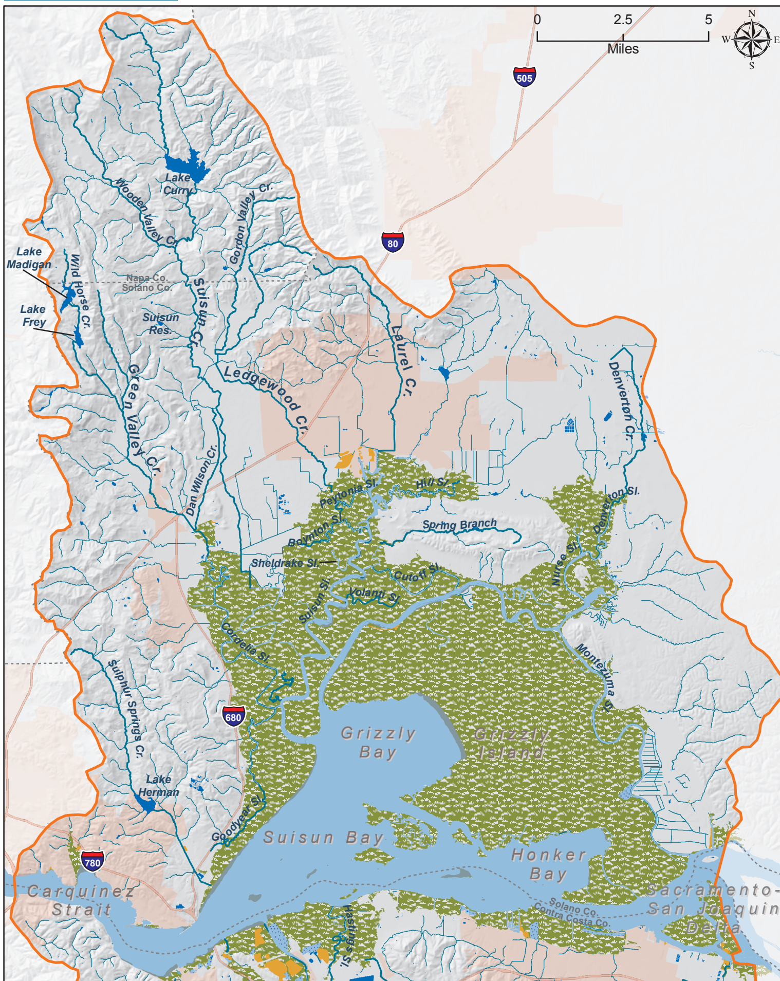
Figure 2-9a Suisun Basin
