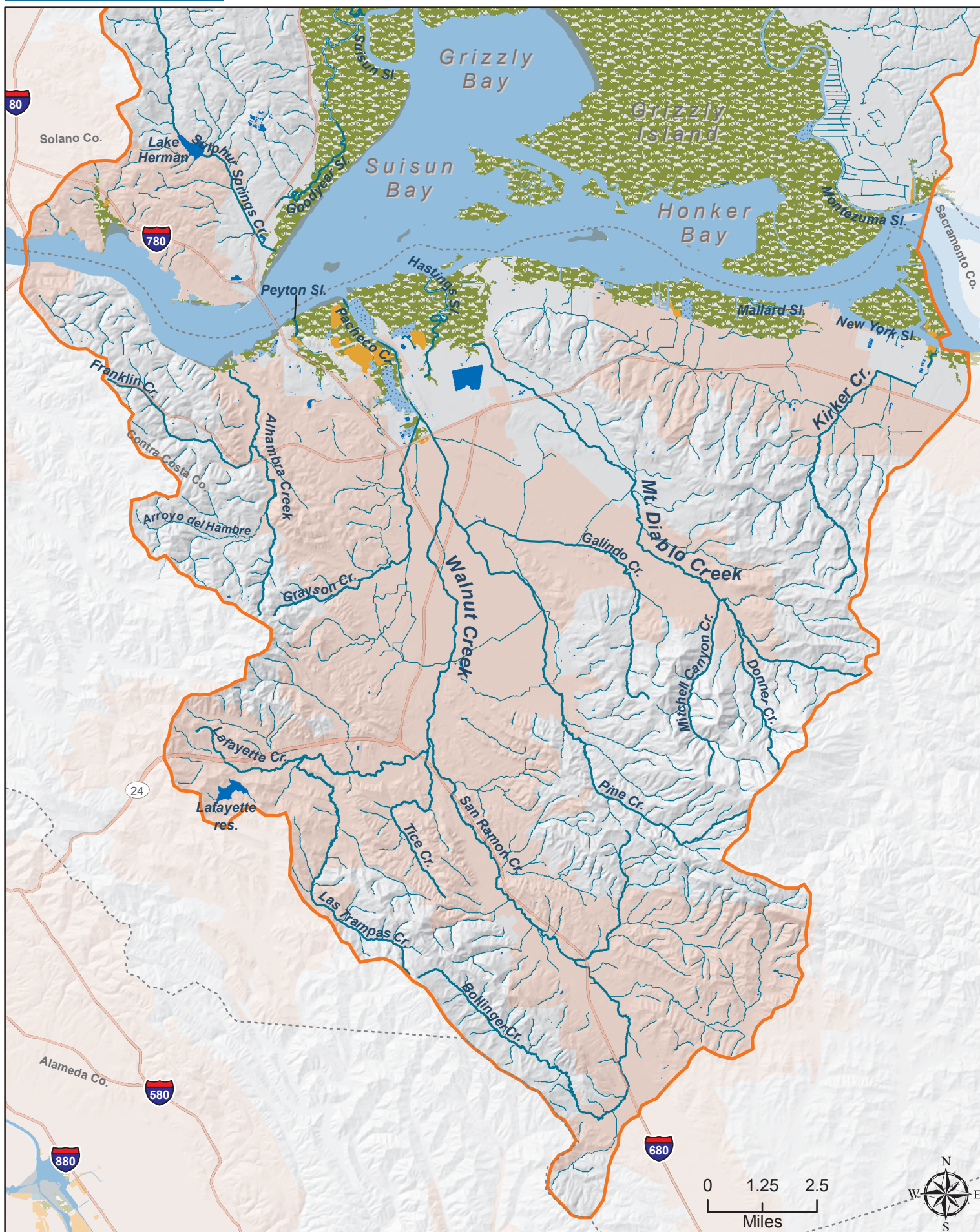
Figure 2-9b Suisun Basin
