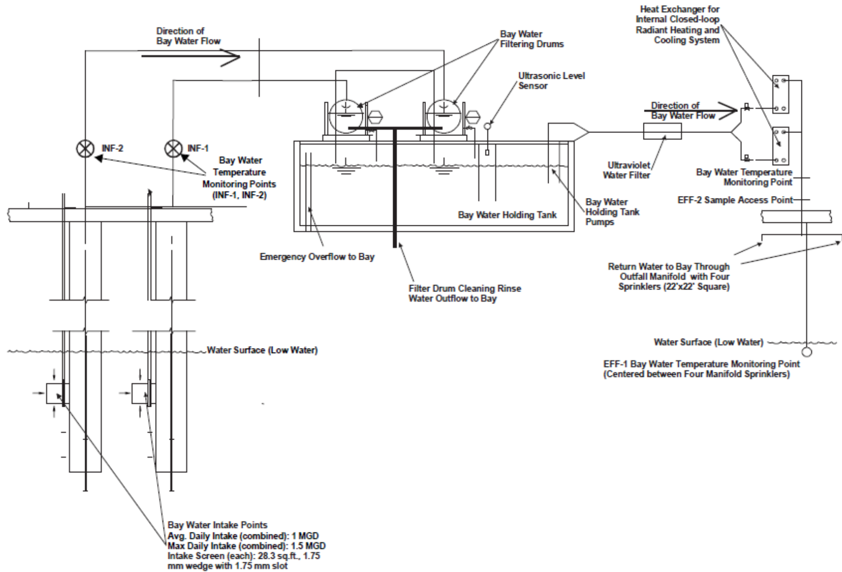
Figure C-2. Flow Schematic
