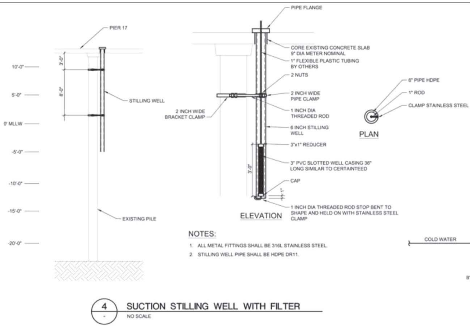
Figure C-7. Fog Bridge Desalination System Intake Details
