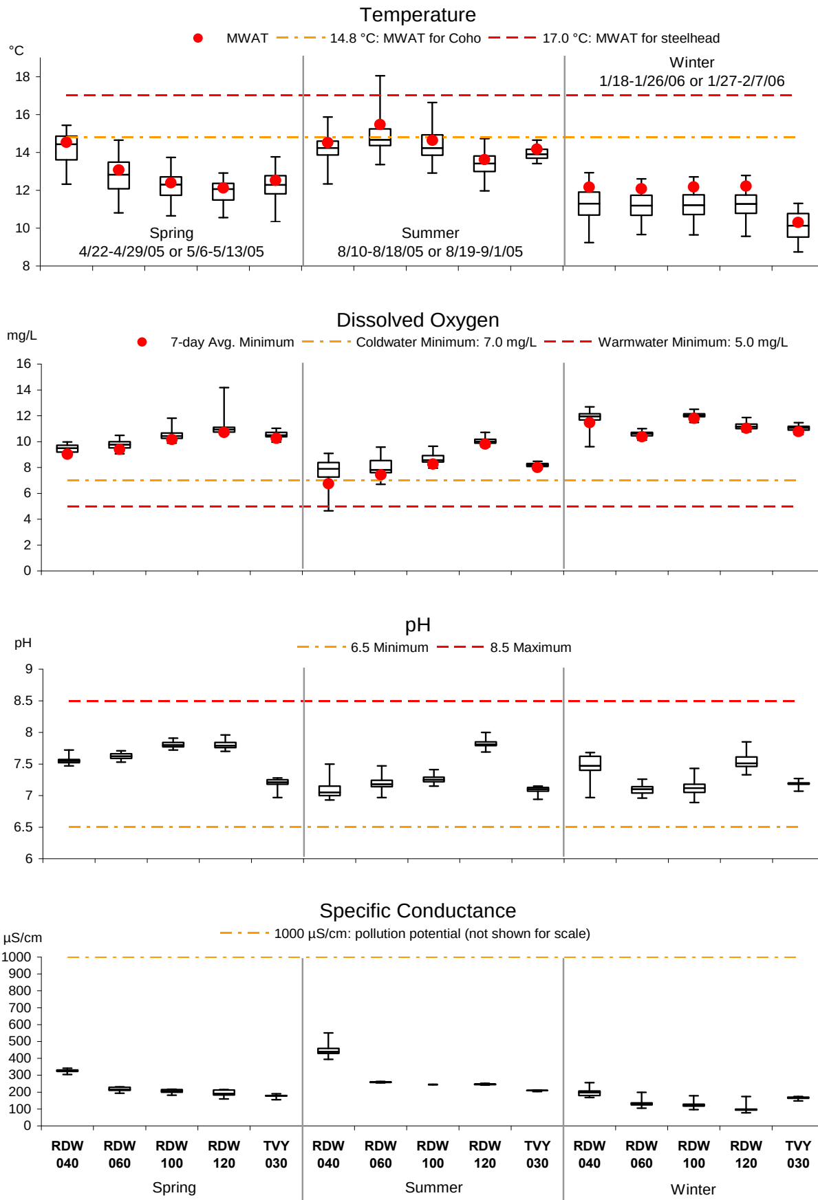
Figure C.4-2b: Continuous field monitoring summaries for Redwood and Tennessee Valley Creeks in 2005-2006
