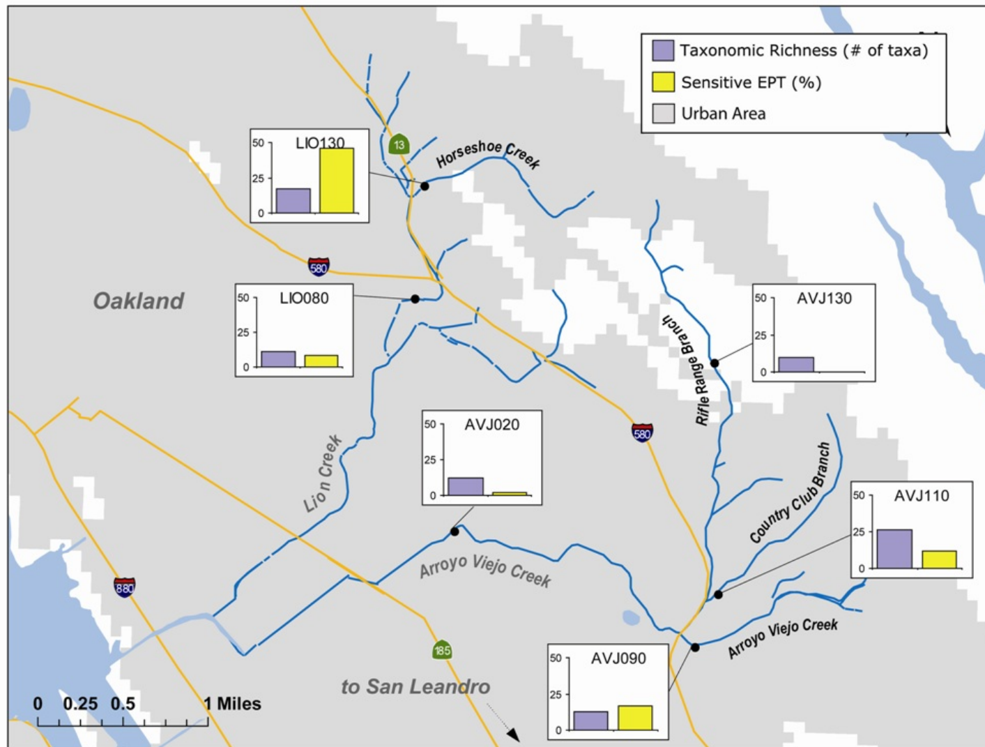
Figure 3.2-2b: Results of selected BMI metrics in the central East Bay (south Oakland) watersheds: Lion and Arroyo Viejo Creeks
