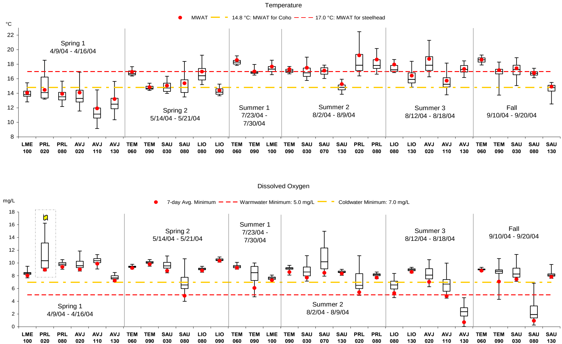
Figure 3.2-2: Continuous field monitoring summaries for temperature and dissolved oxygen in the central East Bay creeks during the spring, summer, and fall of 2004.
