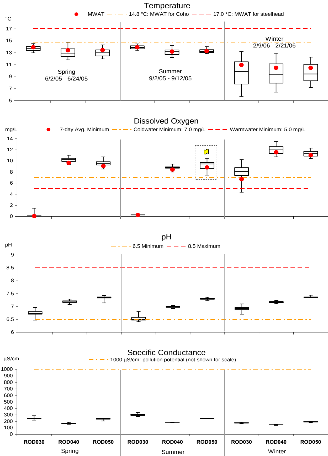
Figure C.4-2d: Continuous field monitoring summaries for Rodeo Creek in 2005-2006
