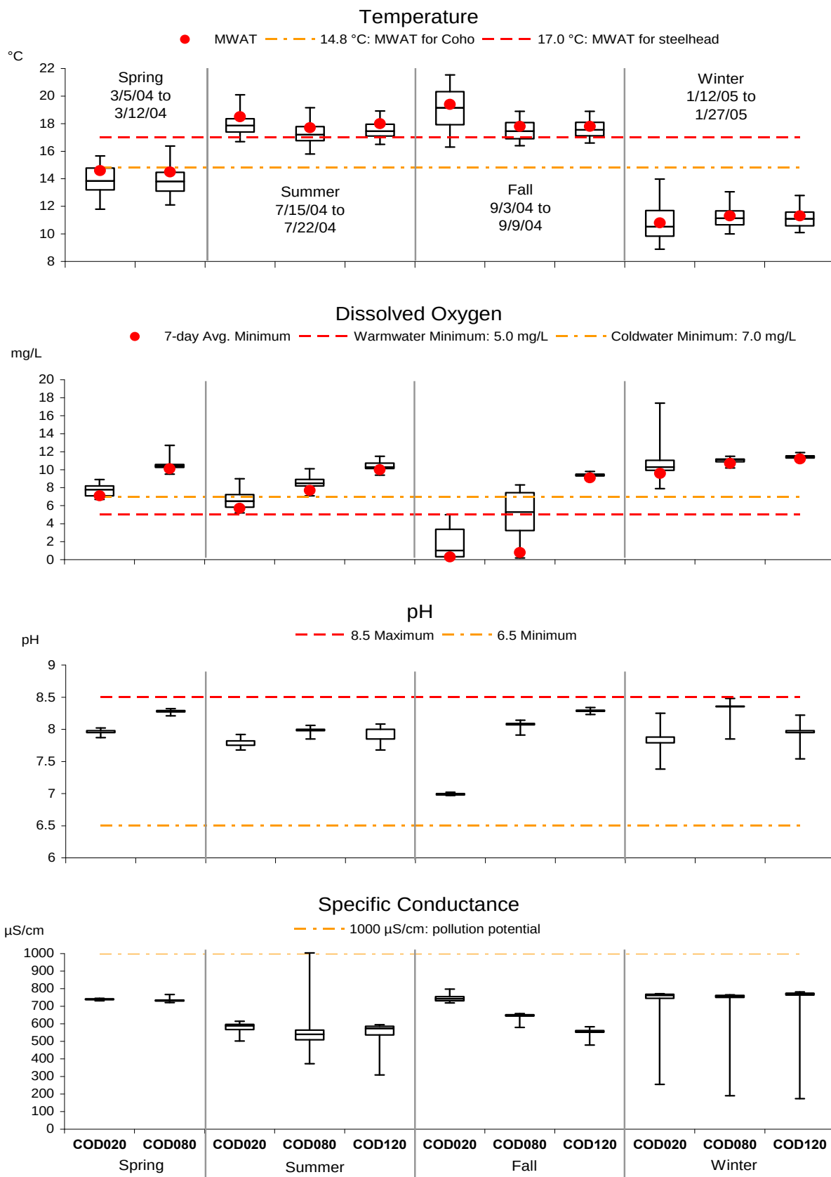
Figure C.1-2b: Continuous field monitoring summaries for Codornices Creek in 2004-2005
