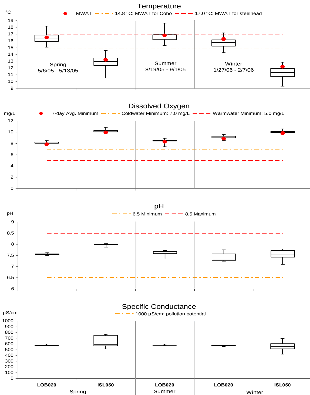
Figure 3.5-1: Continuous field monitoring summaries for San Francisco watersheds: Lobos and Islais Creeks
