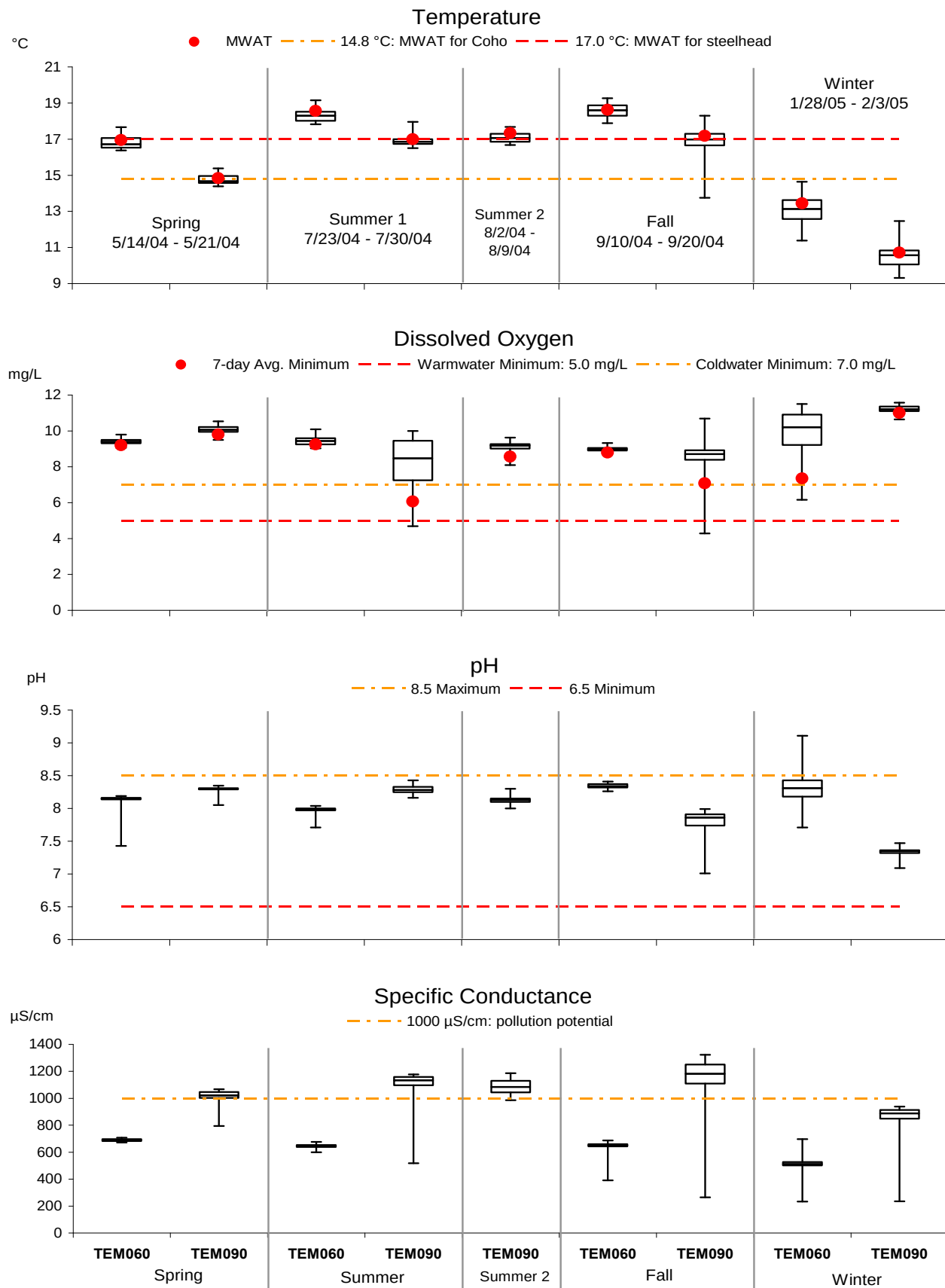
Figure C.2-2a: Continuous field monitoring summaries for Temescal Creek in 2004-2005
