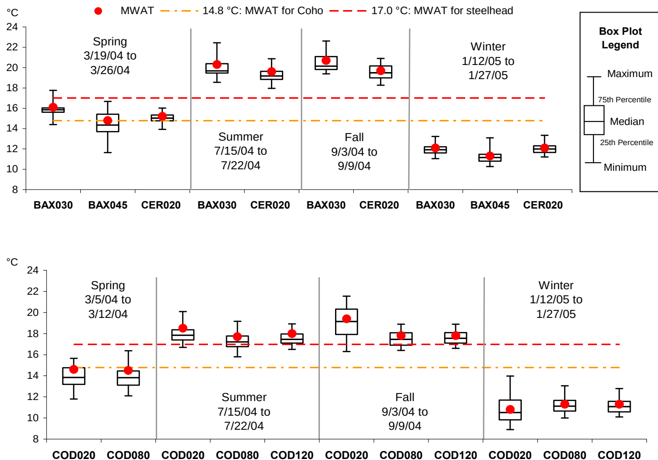
Figure 3.1-2a: Continuous temperature monitoring summaries for Baxter, Cerrito and Codornices Creeks
