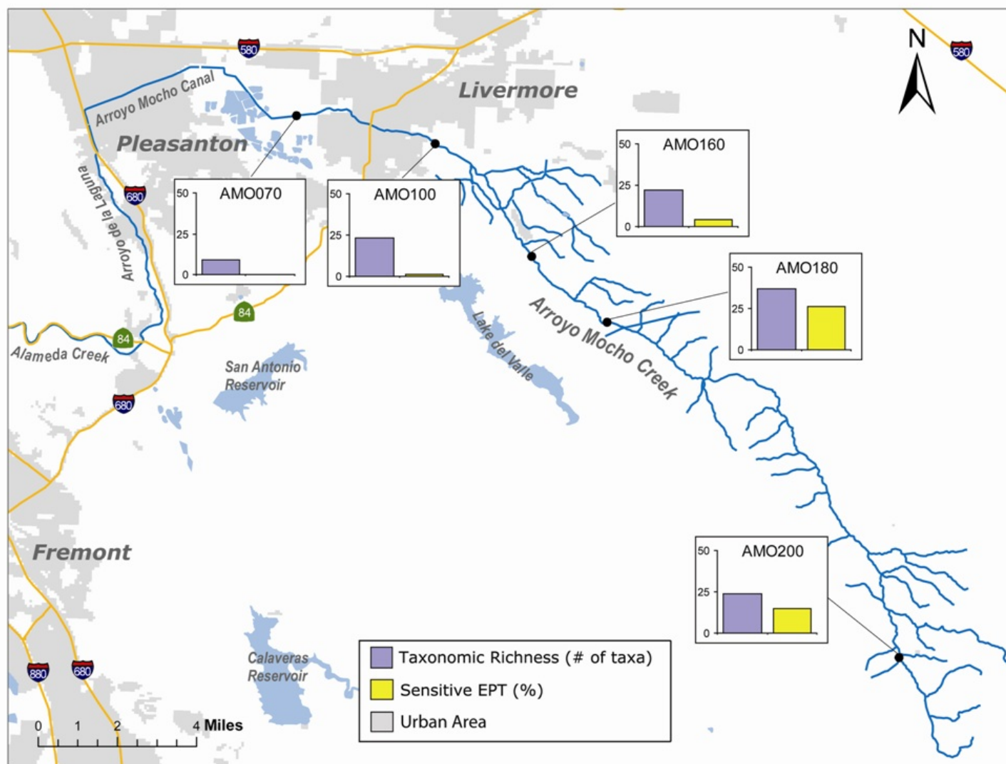
Figure 3.3-1: Results of selected BMI metrics in the Arroyo Mocho watershed
