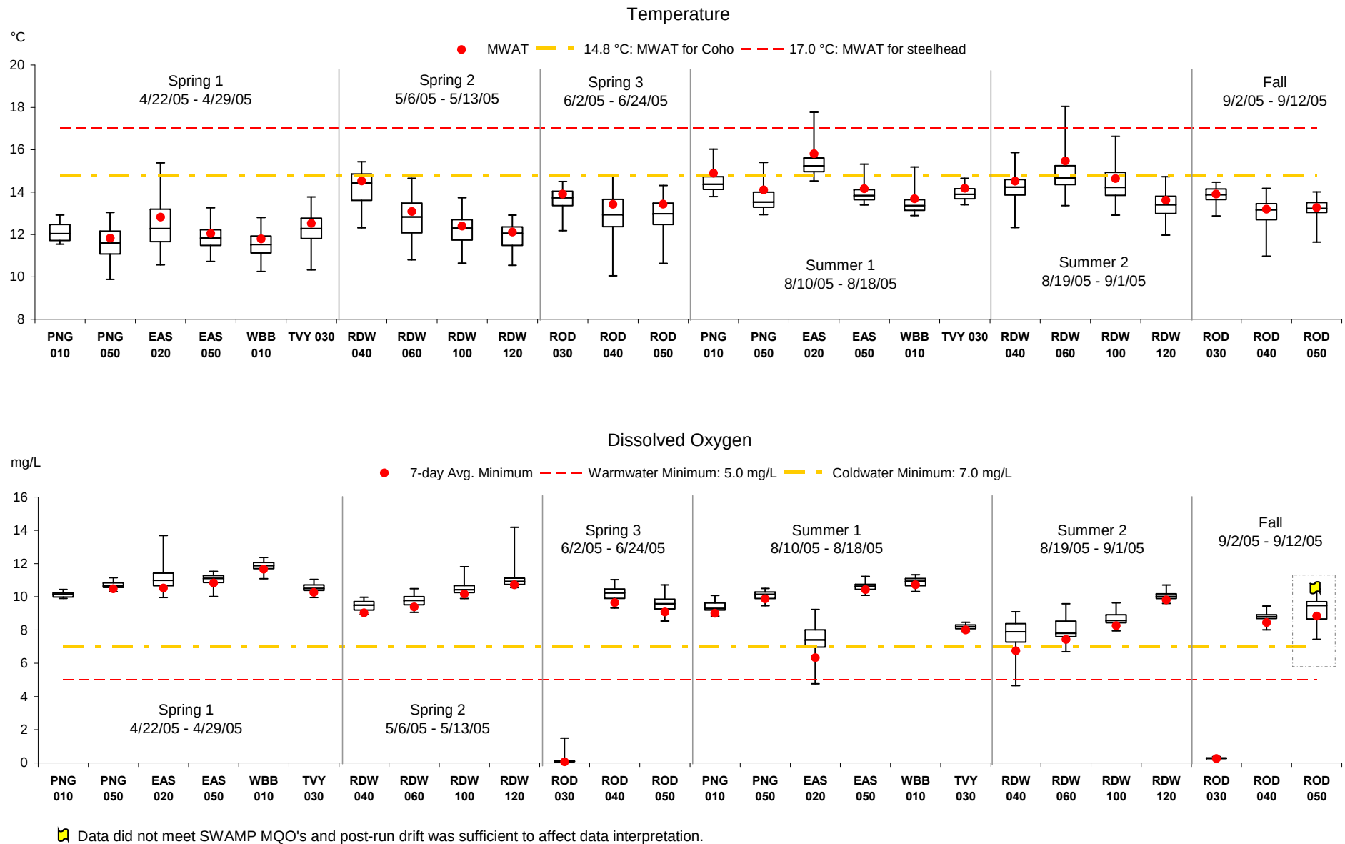
Figure 3.4-2: Continuous field monitoring summaries for temperature and dissolved oxygen in Marin County watersheds during the spring, summer, and fall of 2005
