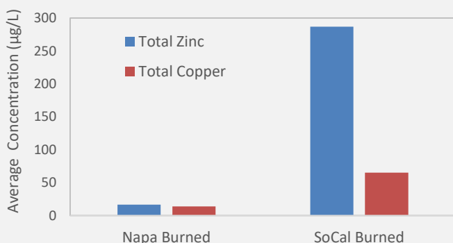
Figure 5. Comparison of metal concentrations in post-fire storm samples for Napa River and Southern California (Stein et al., 2012).
