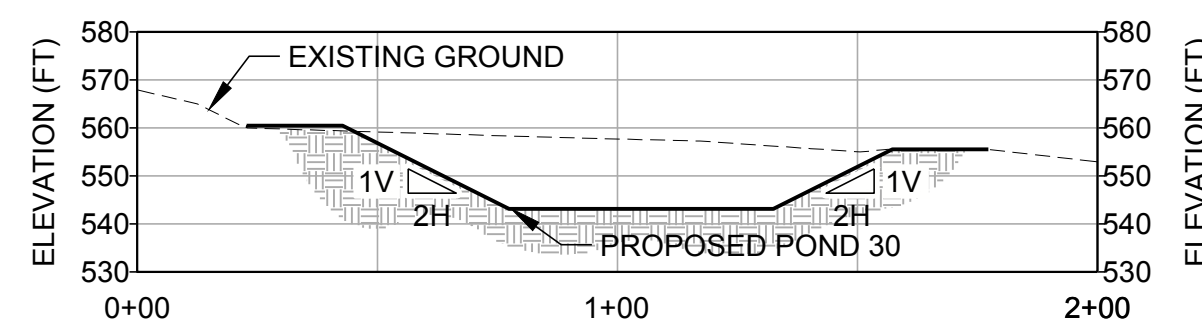
SCALE A B CROSS-SECTION B C-0002
