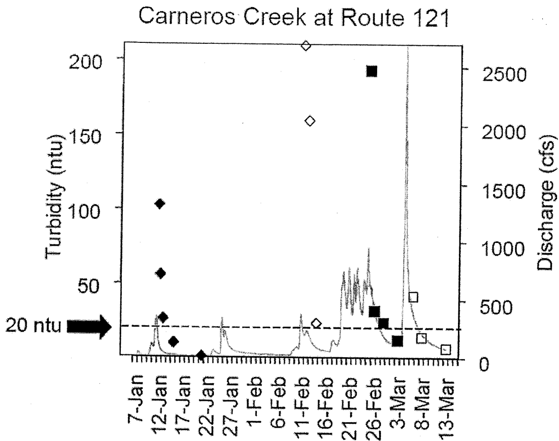
Figure 4. Scatter plot of results from Stillwater and Dietrich (2002) showing turbidity in Carneros Creek showing spikes over 50 ntu on minor storm events, suggesting chronic pulses of turbidity associated with land use.
