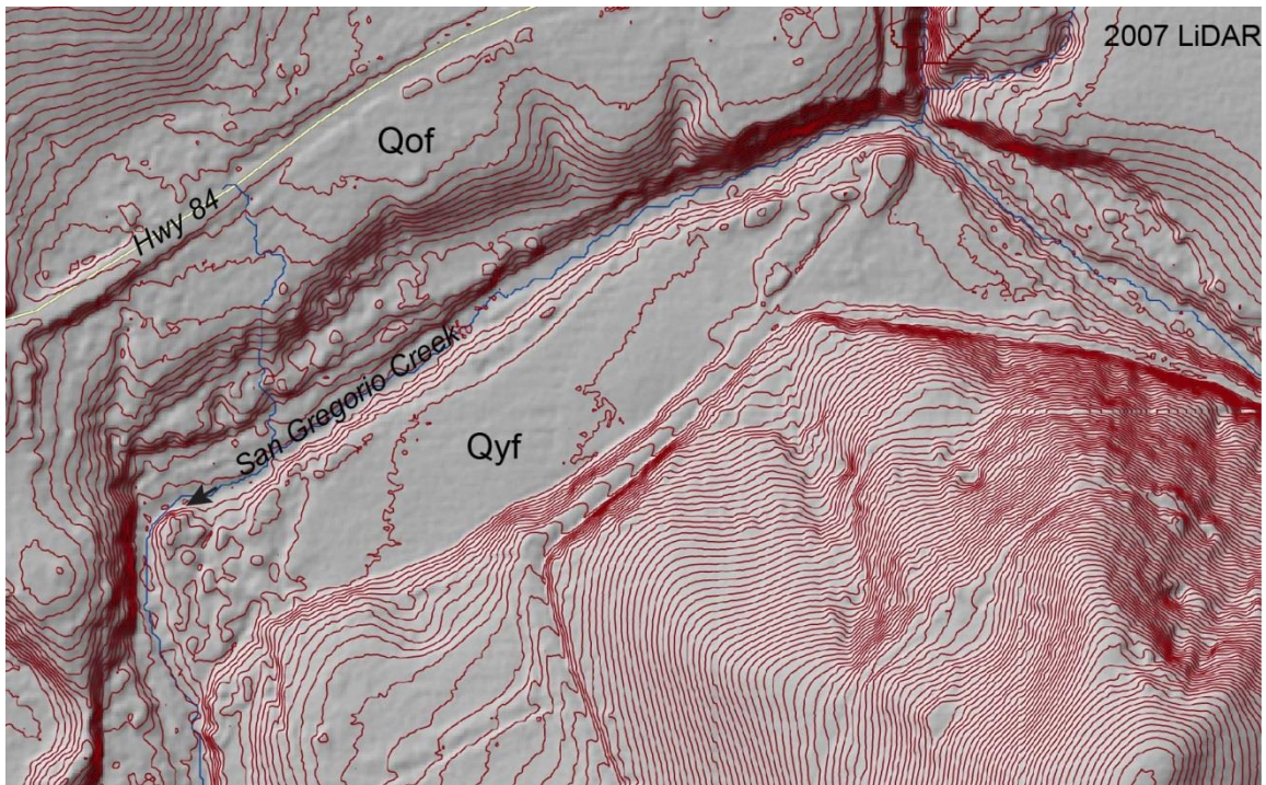
Figure 3. Elevation contours (contour interval 3 ft) that illustrate the relative elevation of the older Pleistocene and younger Holocene surfaces in the downstream portion of San Gregorio Creek.
