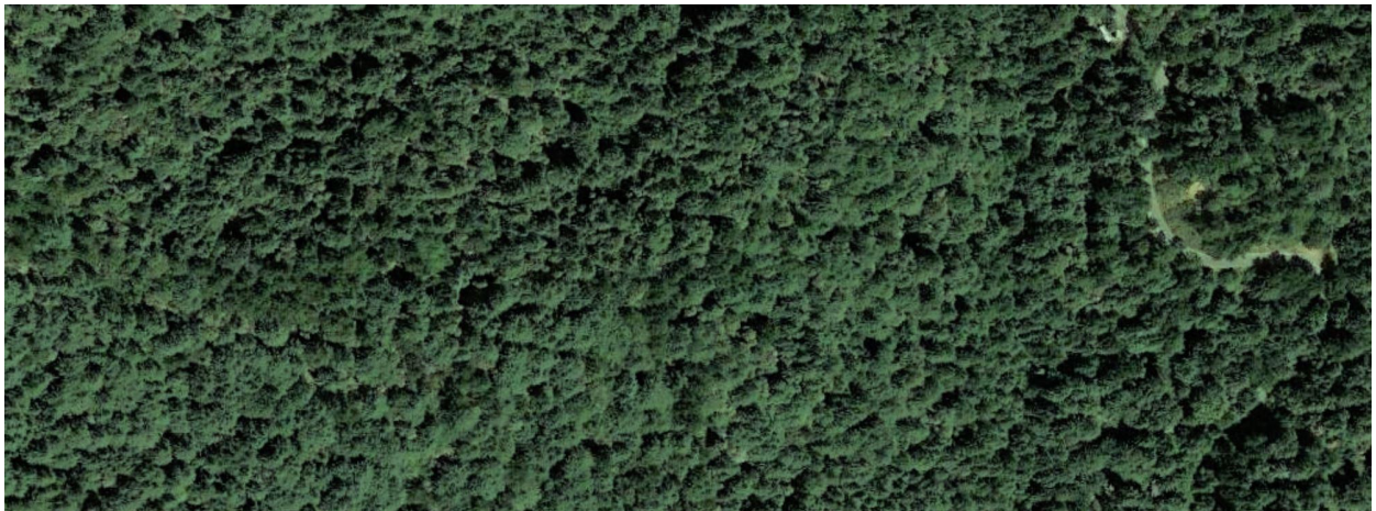
2000 air photo showing recovered forest canopy with no areas of bare surface cover
