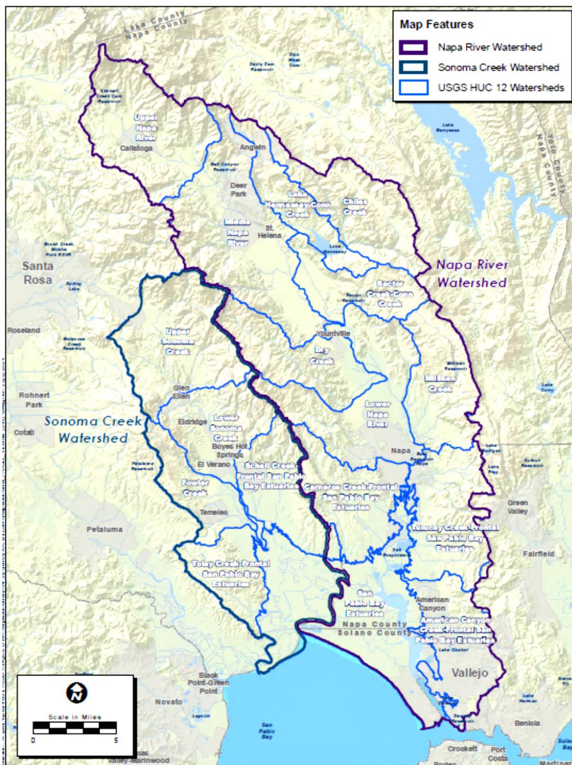
Figure 6-1: HUC 12 Watersheds
