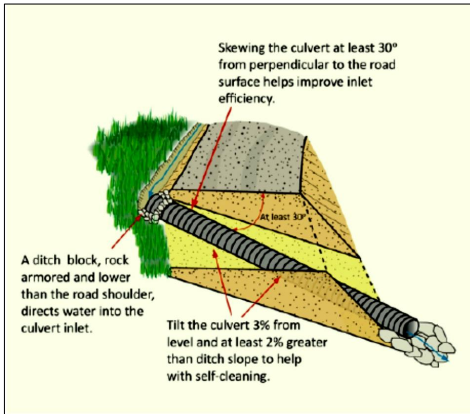
Figure 2-13: Schematic illustration of a typical ditch relief culvert. Note: The ditch relief culvert is installed at the base of the road fill.
