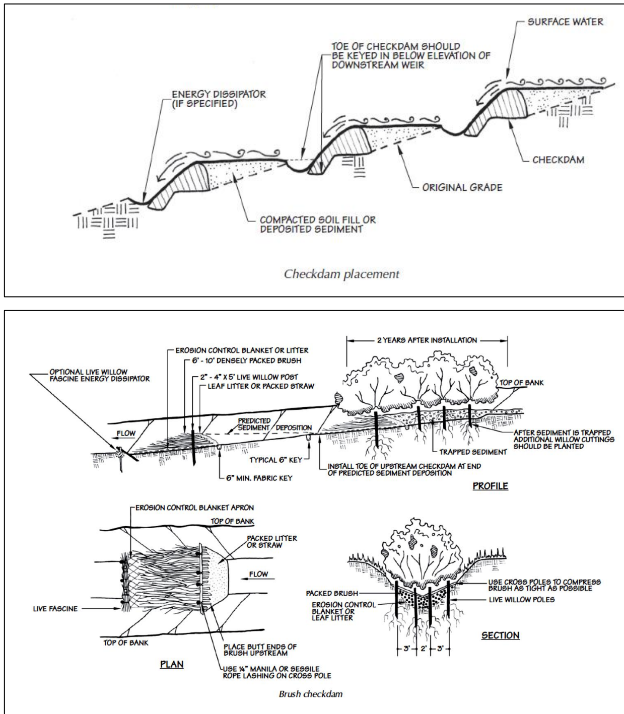
Schematic illustration of a brush check dam (Source: Marin RCD, 2007)
