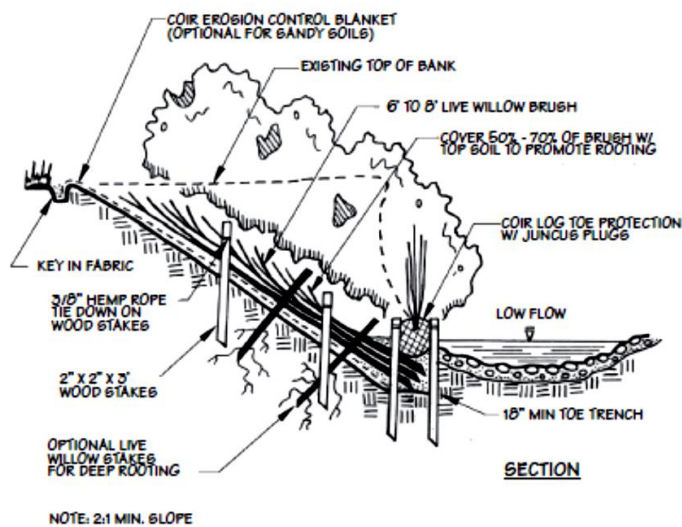
Brush mattress, section view
