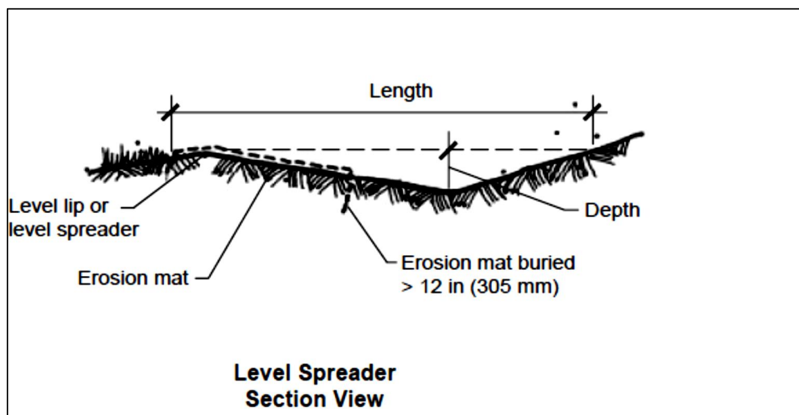
Figure 2-7: Conceptual layout of a level spreader
