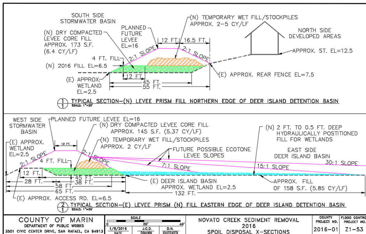
Figure 17. The cross-section of the proposed beneficial reuse, with the engineered core shown in green, and the ecotone in blue. (Image: MCWCFCFCD)
