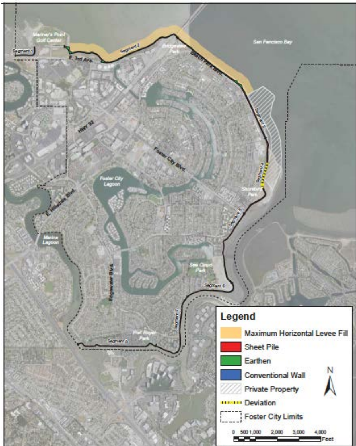
Figure 21. The proposed horizontal levee alternative along Segment 2 of the Foster City levees. (Image: Foster City)
