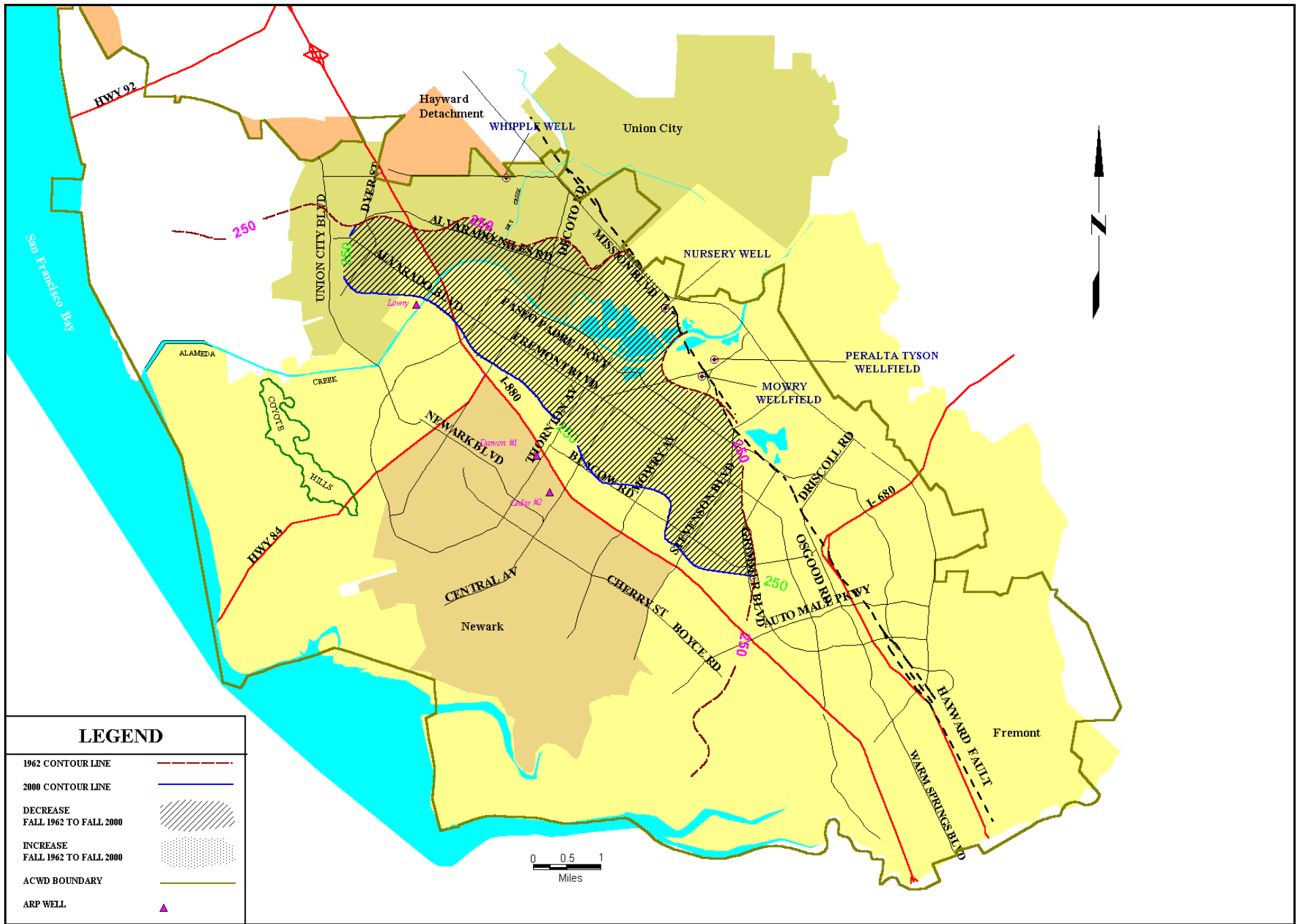
Figure 12: Comparison of 1962 and 2000 250-ppm Chloride Contours, Newark Aquifer (Source: Alameda County Water District)
