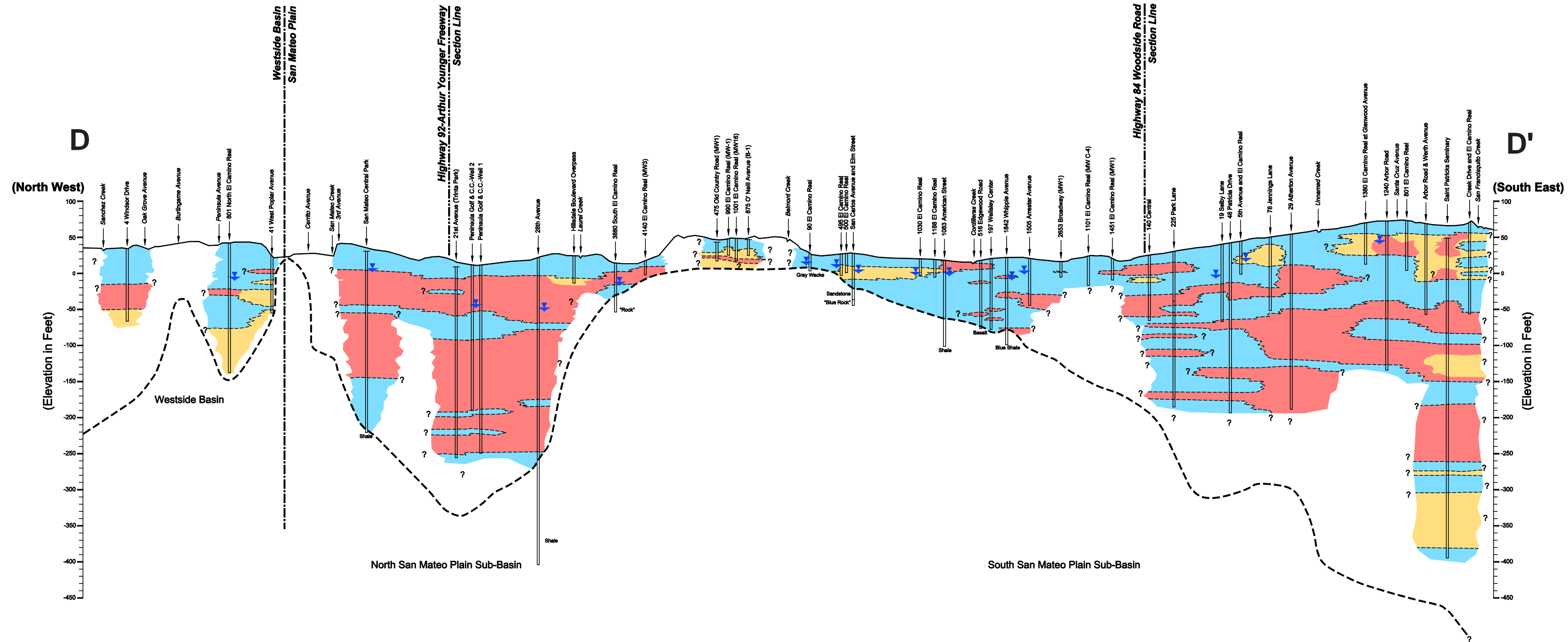
Geologic Cross-Section El Camino Real - Highway 82
