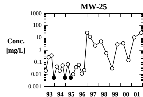
CHART 3.5-1b Summary of Monitoring Well Zinc Concentrations for the Period 1993-2001 (Solid Circles are Detection Limit and Empty Circles are Measured Values)
