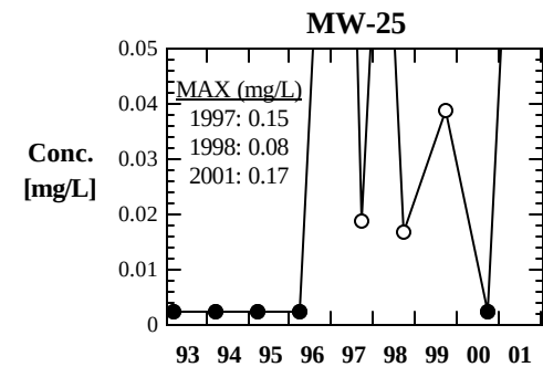
CHART 3.5-1a Summary of Monitoring Well Copper Concentrations for the Period 1993-2001 (Solid Circles are Detection Limit and Empty Circles are Measured Values)
