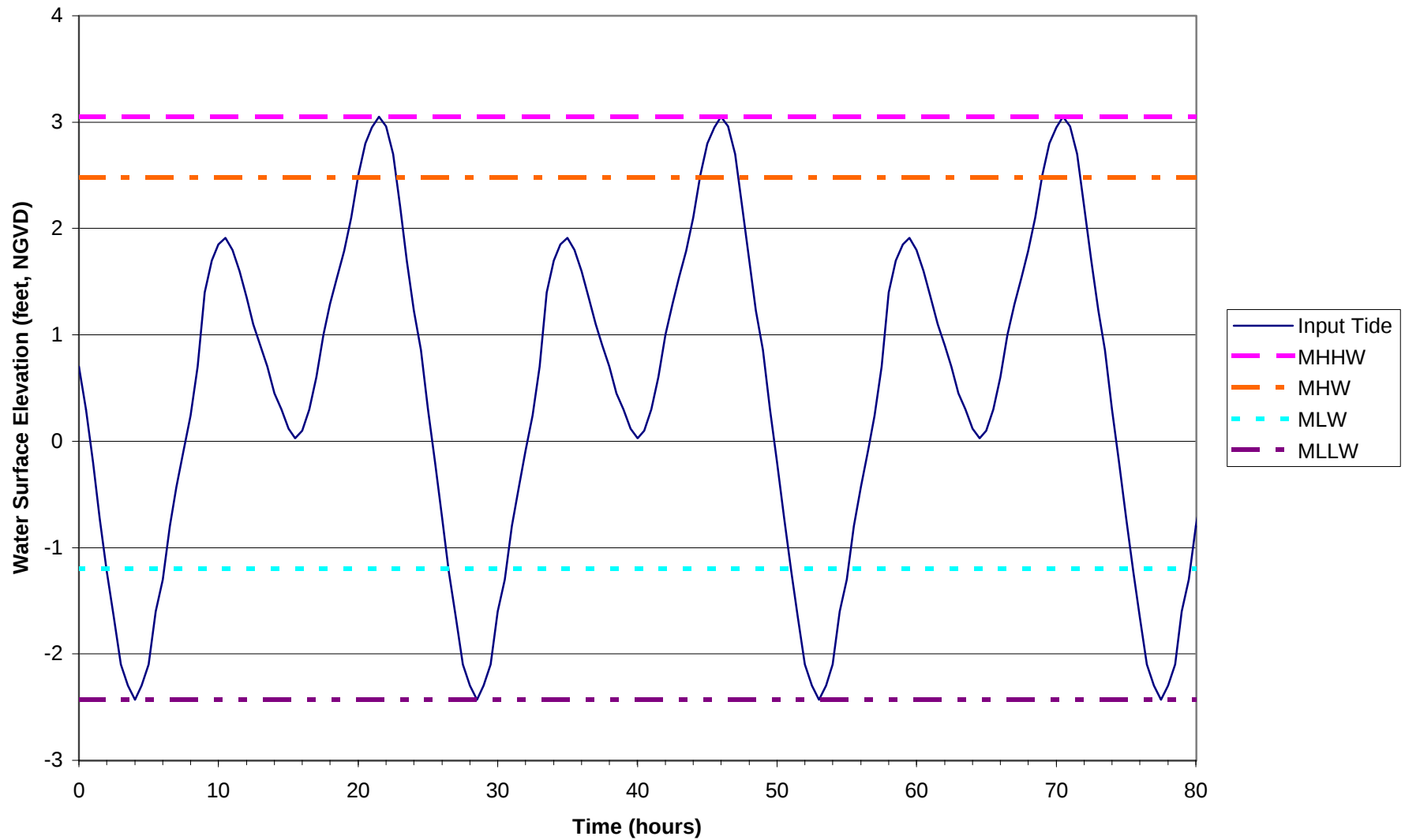
Figure 3.3-3. Synthesized Average Suisun Point Input Tide
