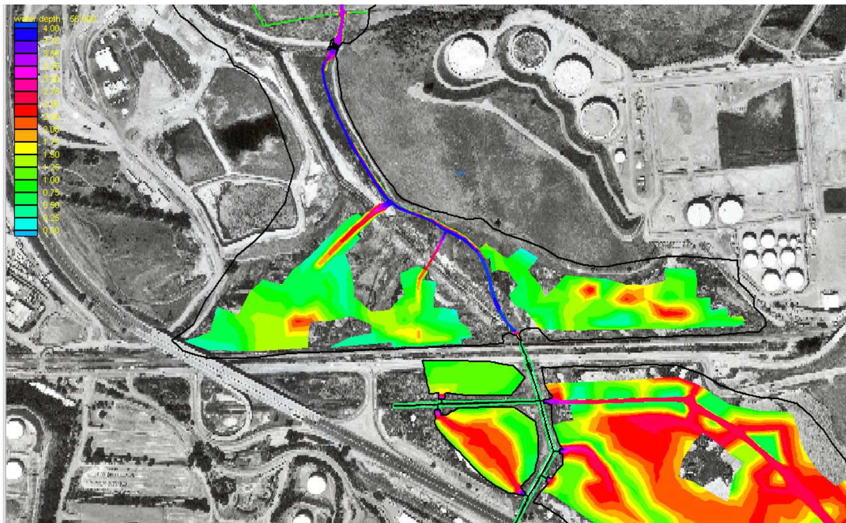
Figure 3.3-5b. Water Depth at Mean Lower Low Water South of the Tide Gates for Scenario 3
