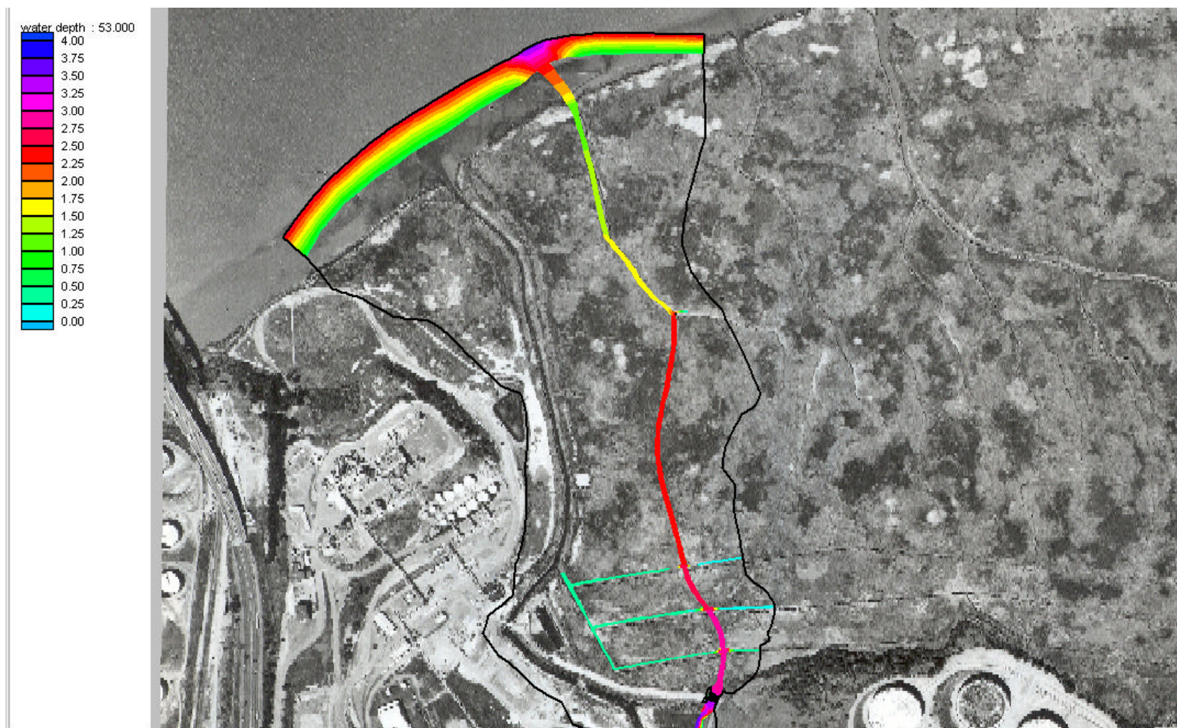
Figure 3.3-5a. Water Depth at Mean Lower Low Water North of the Tide Gates for Scenario 3
