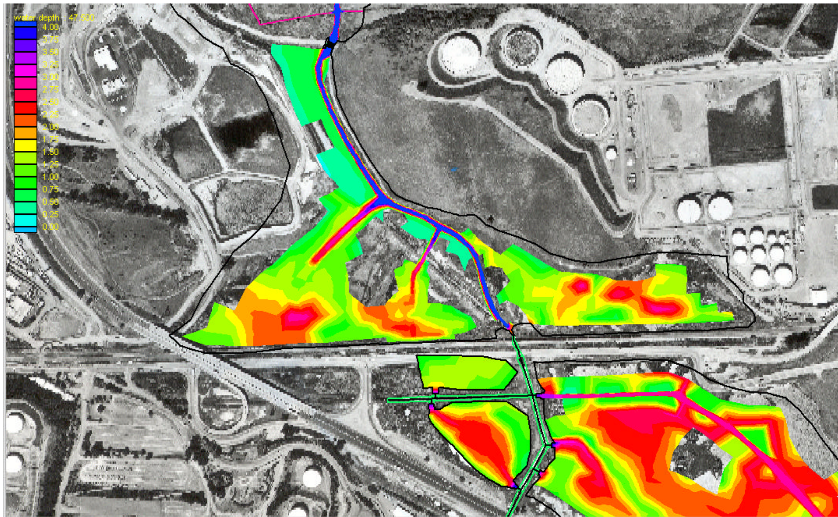
Figure 3.3-4b. Water Depth at Mean Higher High Water South of the Tide Gates for Scenario 3
