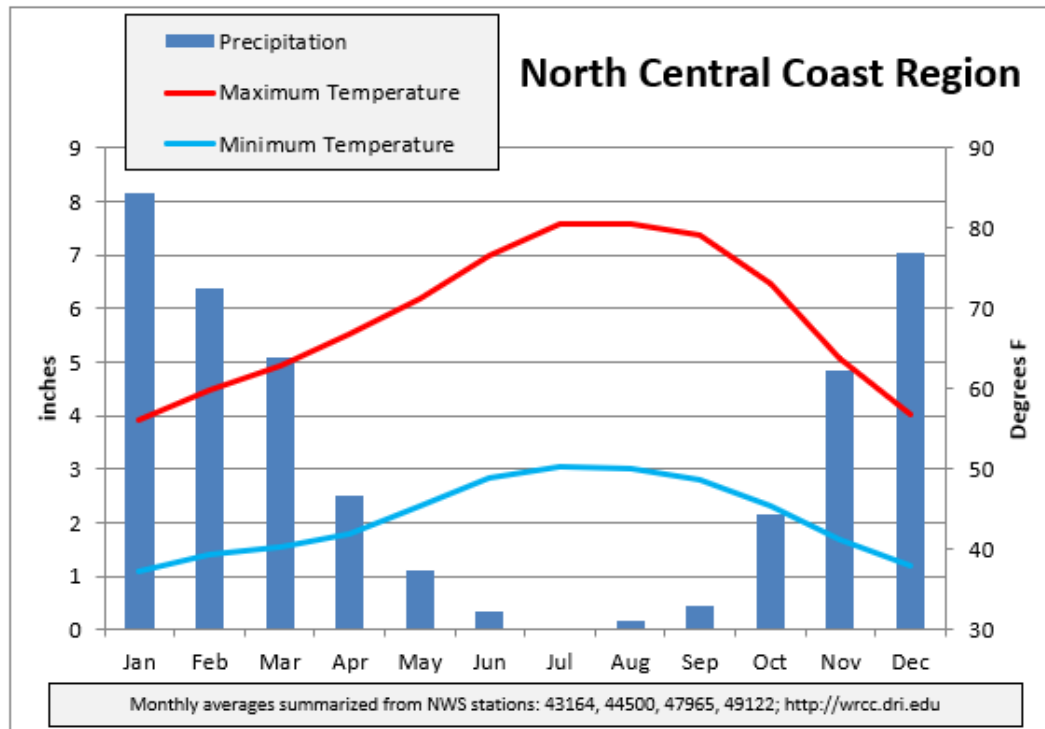
Chart A-11. Average annual patterns of temperature and precipitation in the North Central Coast Region.
