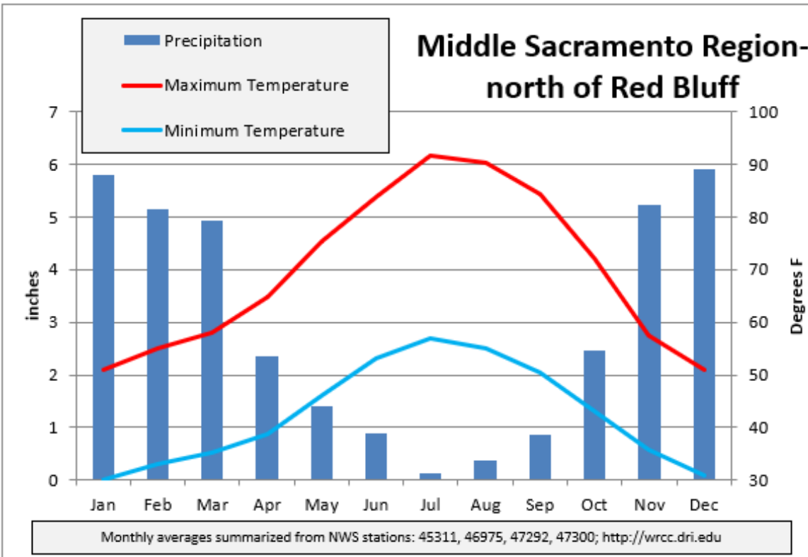
Chart A-6. Average annual patterns of temperature and precipitation in the Middle Sacramento Region, north of Red Bluff.
