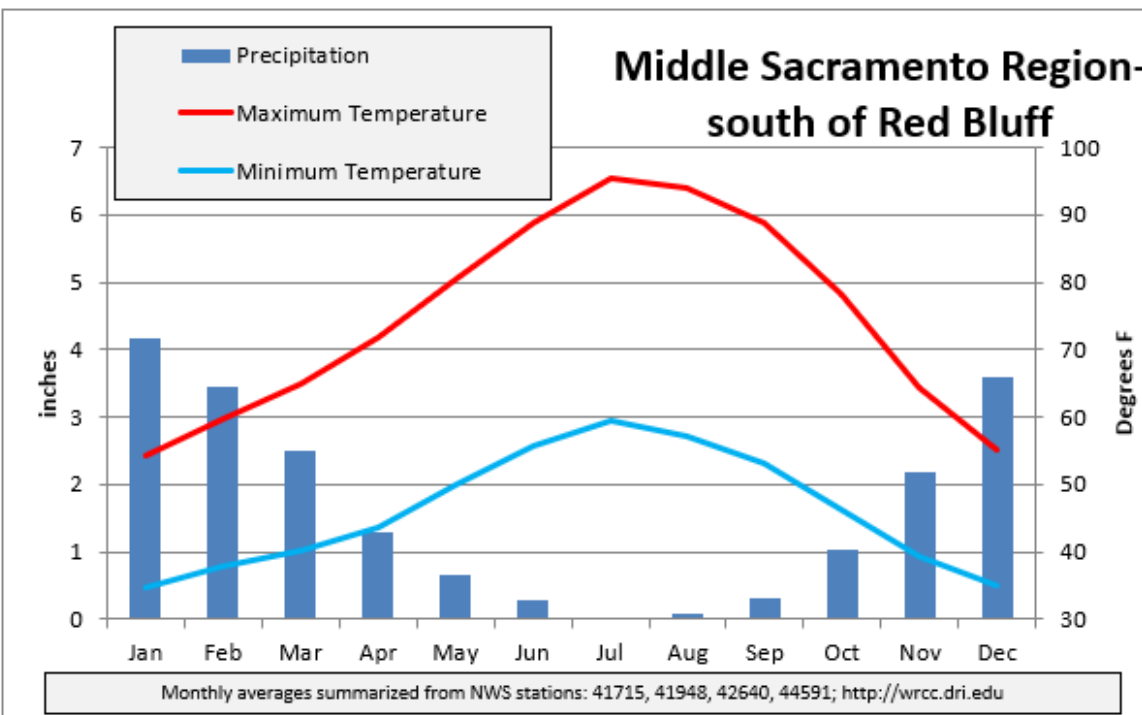
Chart A-7. Average annual patterns of temperature and precipitation in the Middle Sacramento Region, south of Red Bluff.
