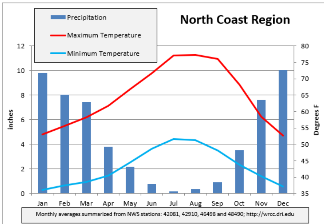
Chart A-5. Average annual patterns of temperature and precipitation in the North Coast Region.
