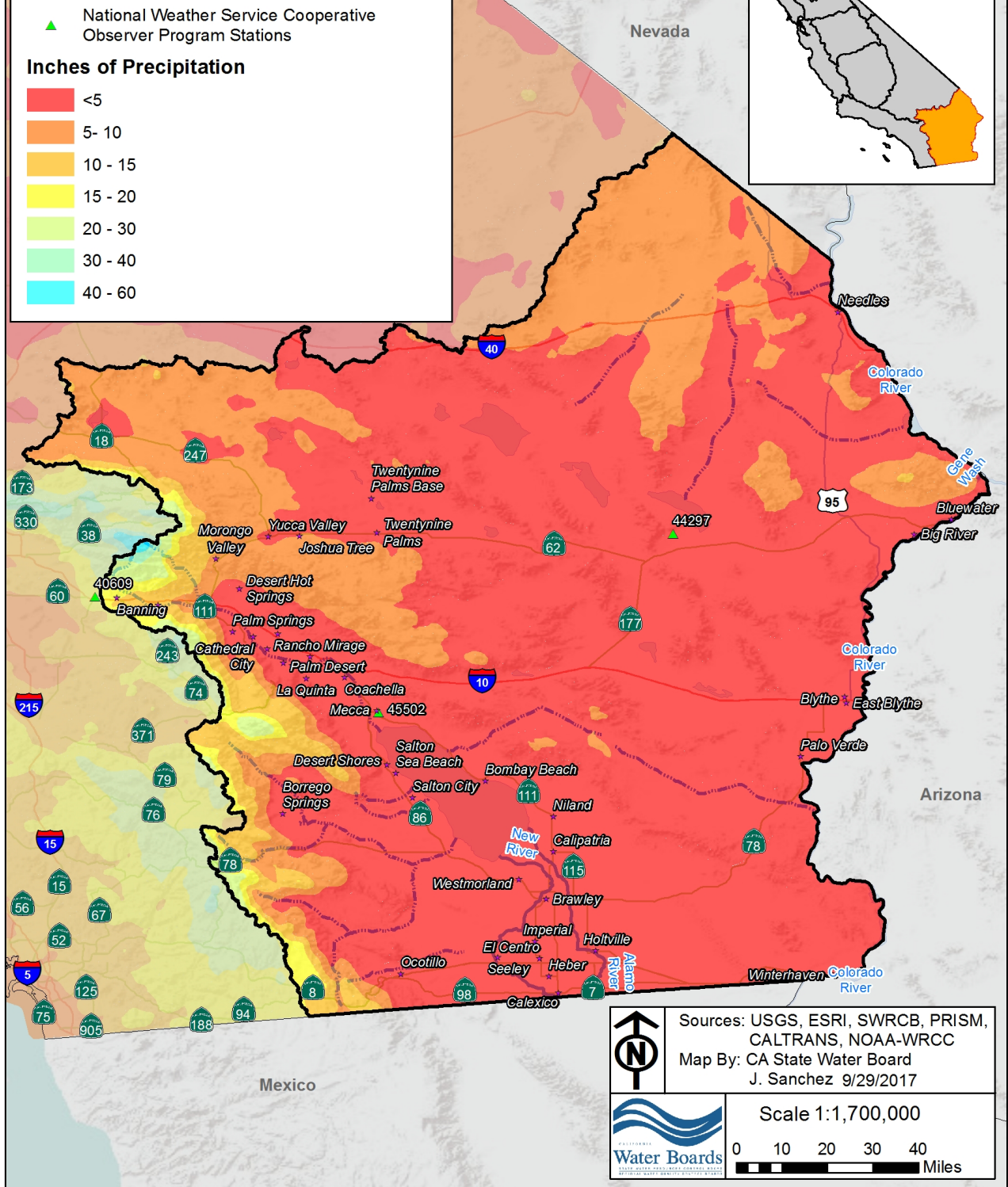
Figure A-77. South East Desert Region- Average Annual Precipitation (1981-2010)
