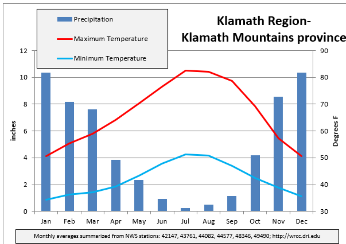
Chart A- 1. Average annual patterns of temperature and precipitation in the Klamath Region, Klamath Mountains province.
