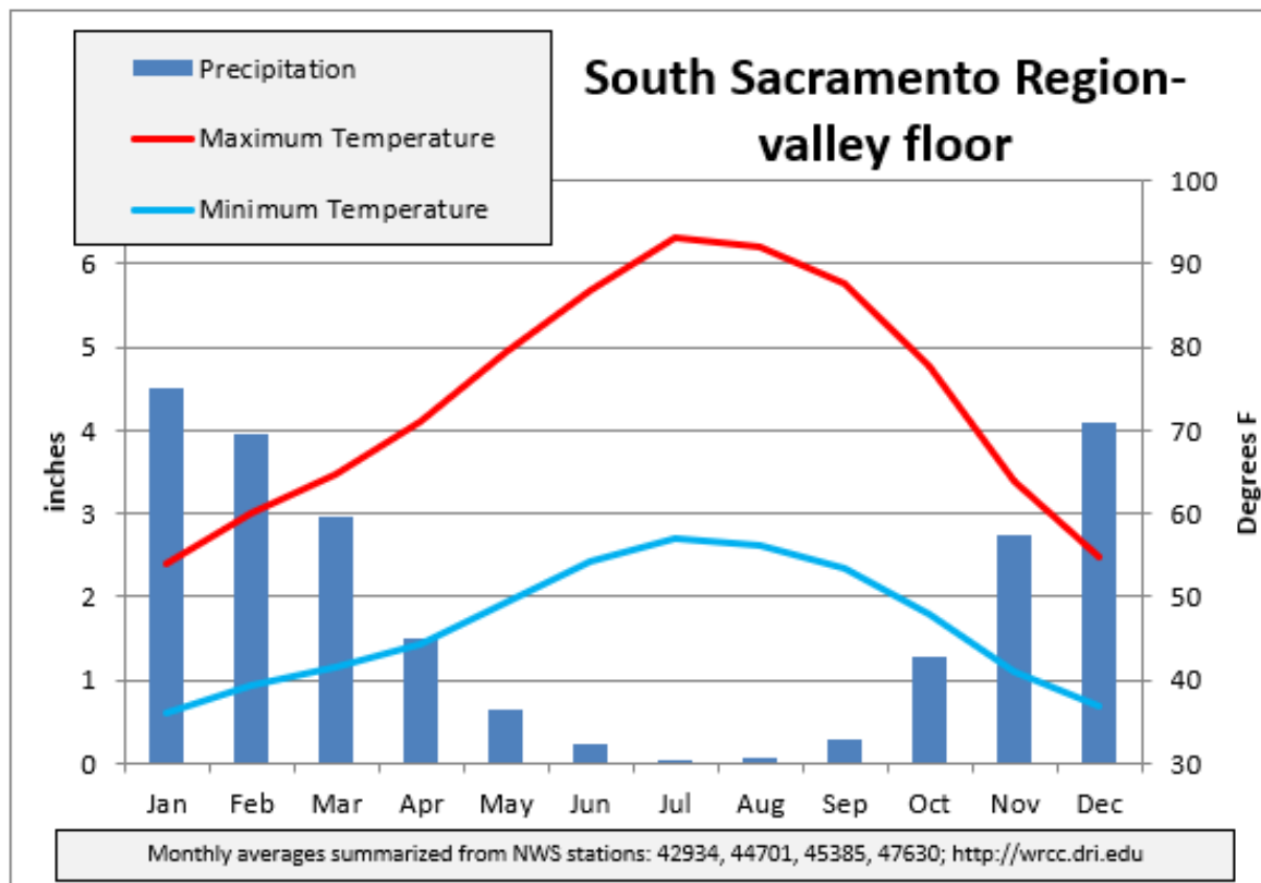
Chart A-8. Average annual patterns of temperature and precipitation in the South Sacramento Region, valley floor.
