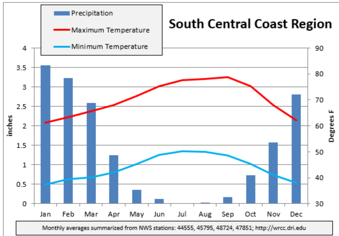
Chart A-12. Average annual patterns of temperature and precipitation in the South Central Coast Region.
