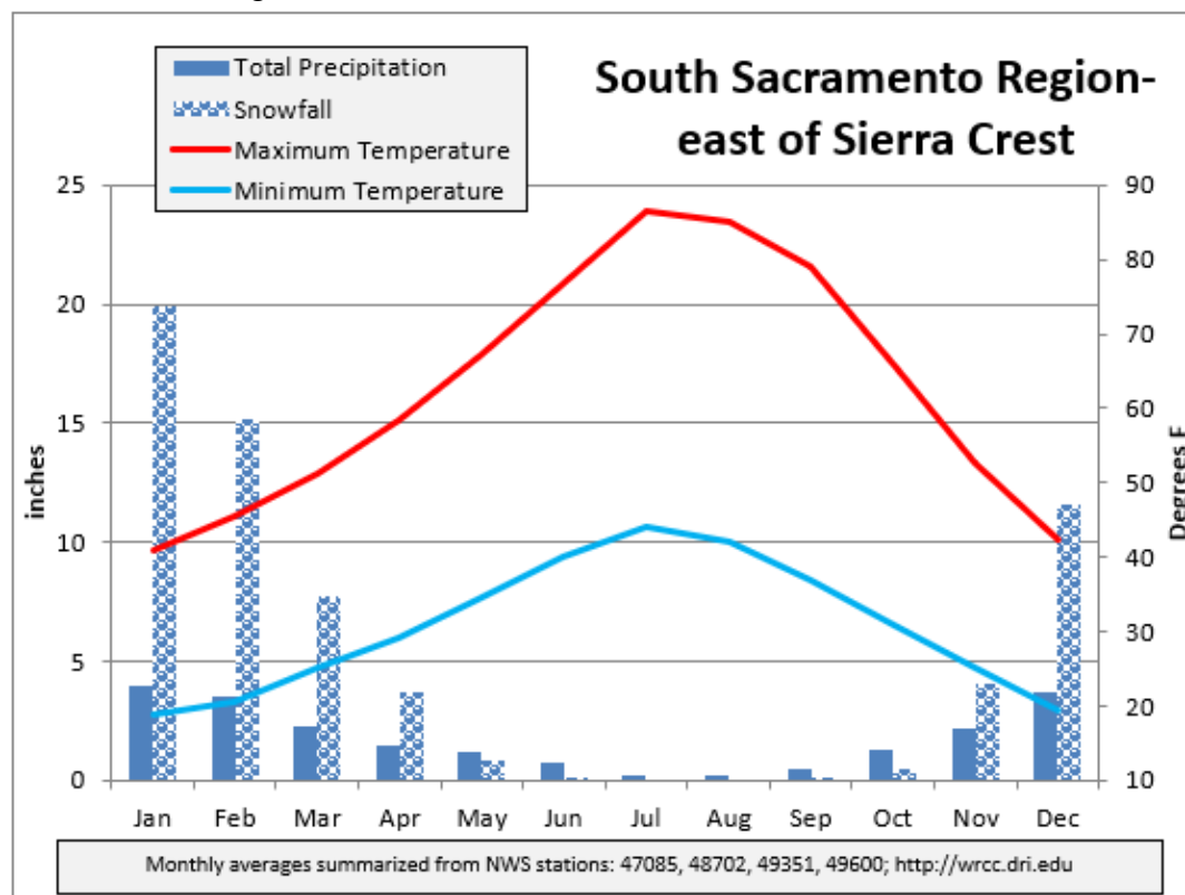
Chart A-10. Average annual patterns of temperature and precipitation in the South Sacramento Region, east of Sierra Crest.
