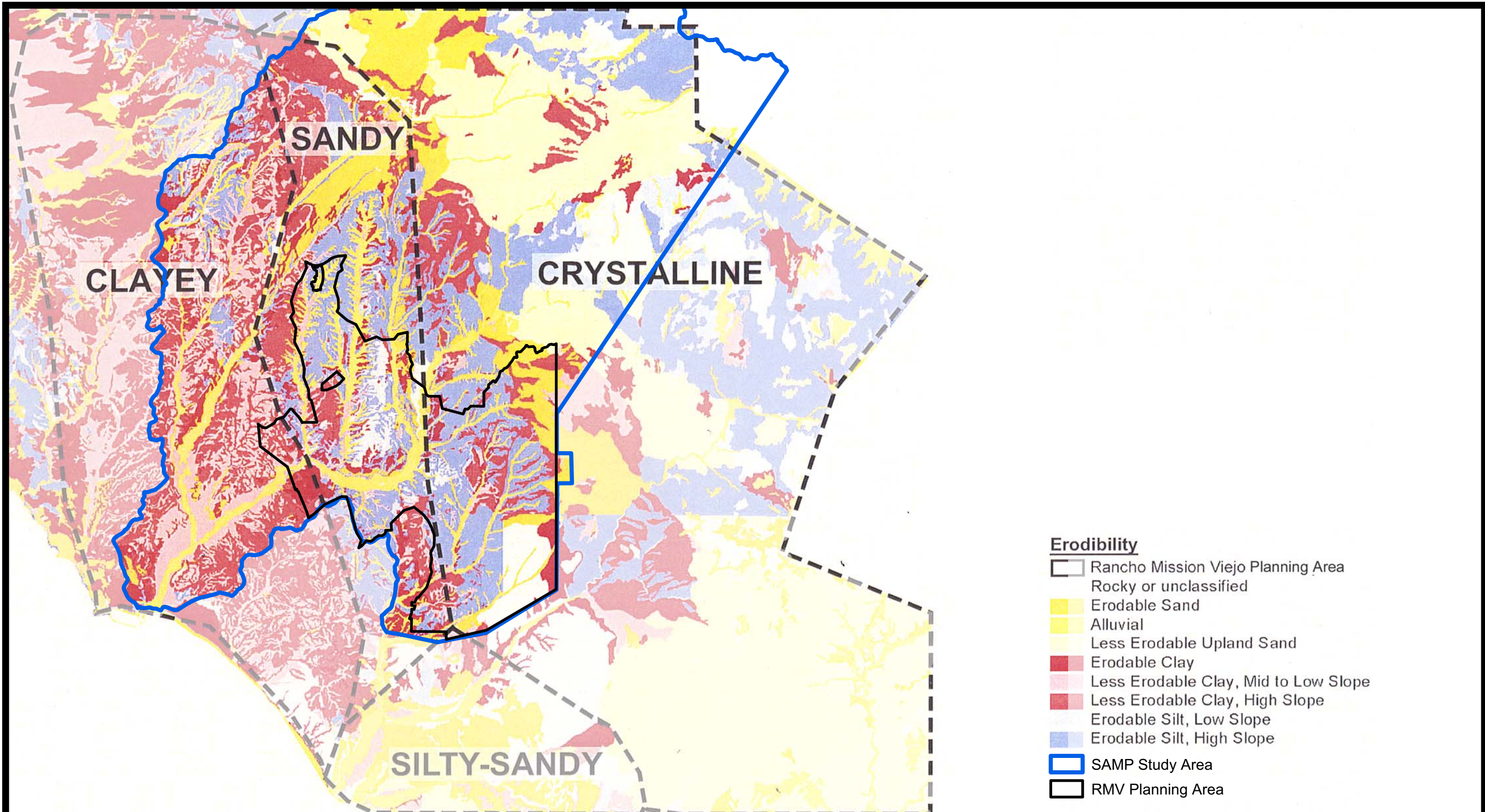
Landscape-scale Terrains and Shallow Substrate Erodibility
