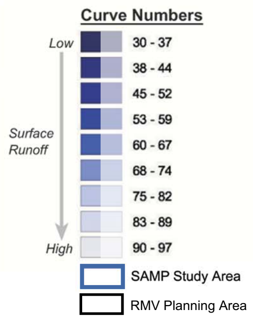
Distribution of Soil Conservation Service Runoff Curve Numbers for the San Juan Creek Watershed
