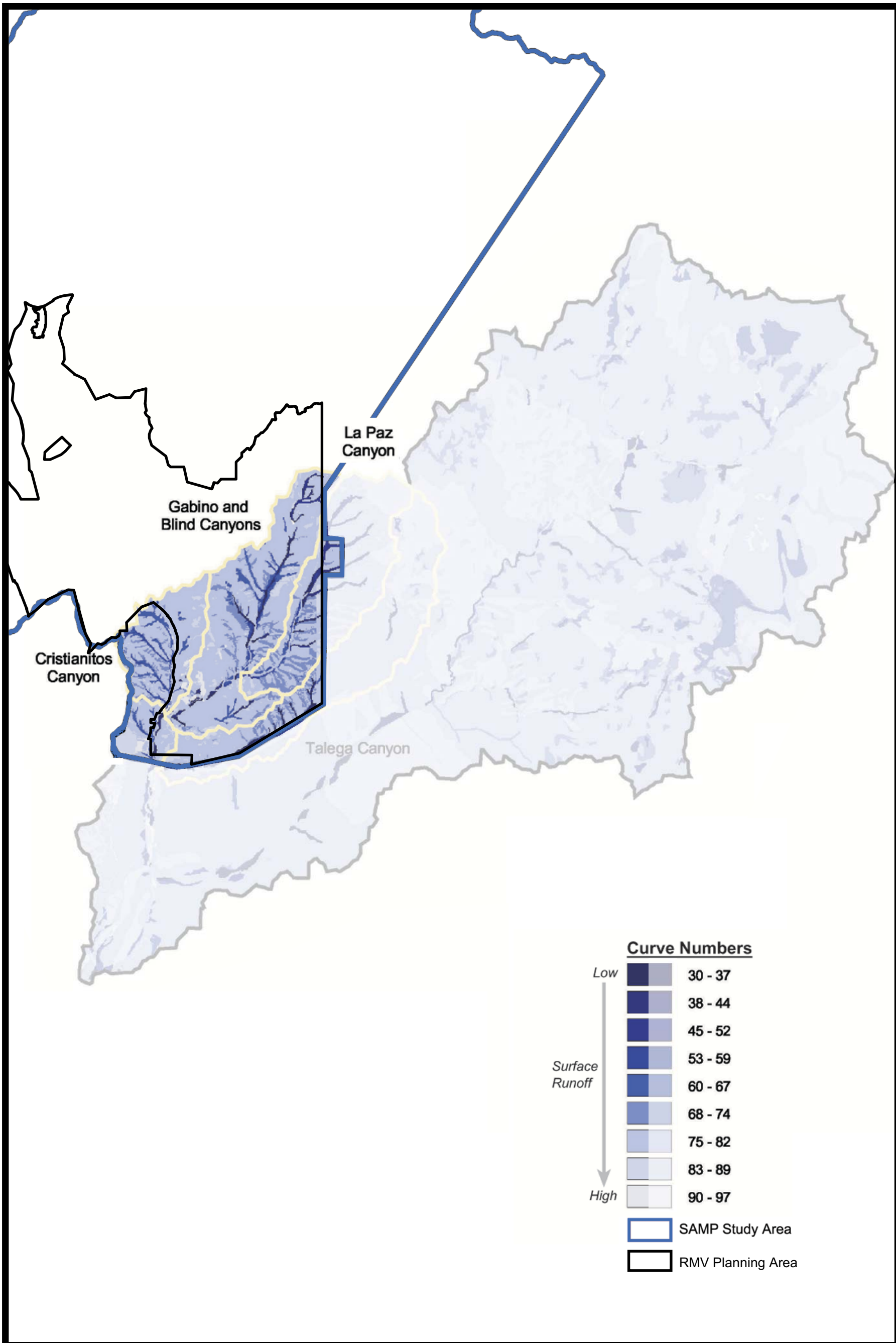
Distribution of Soil Conservation Service Runoff Curve Numbers for the San Mateo Creek Watershed
