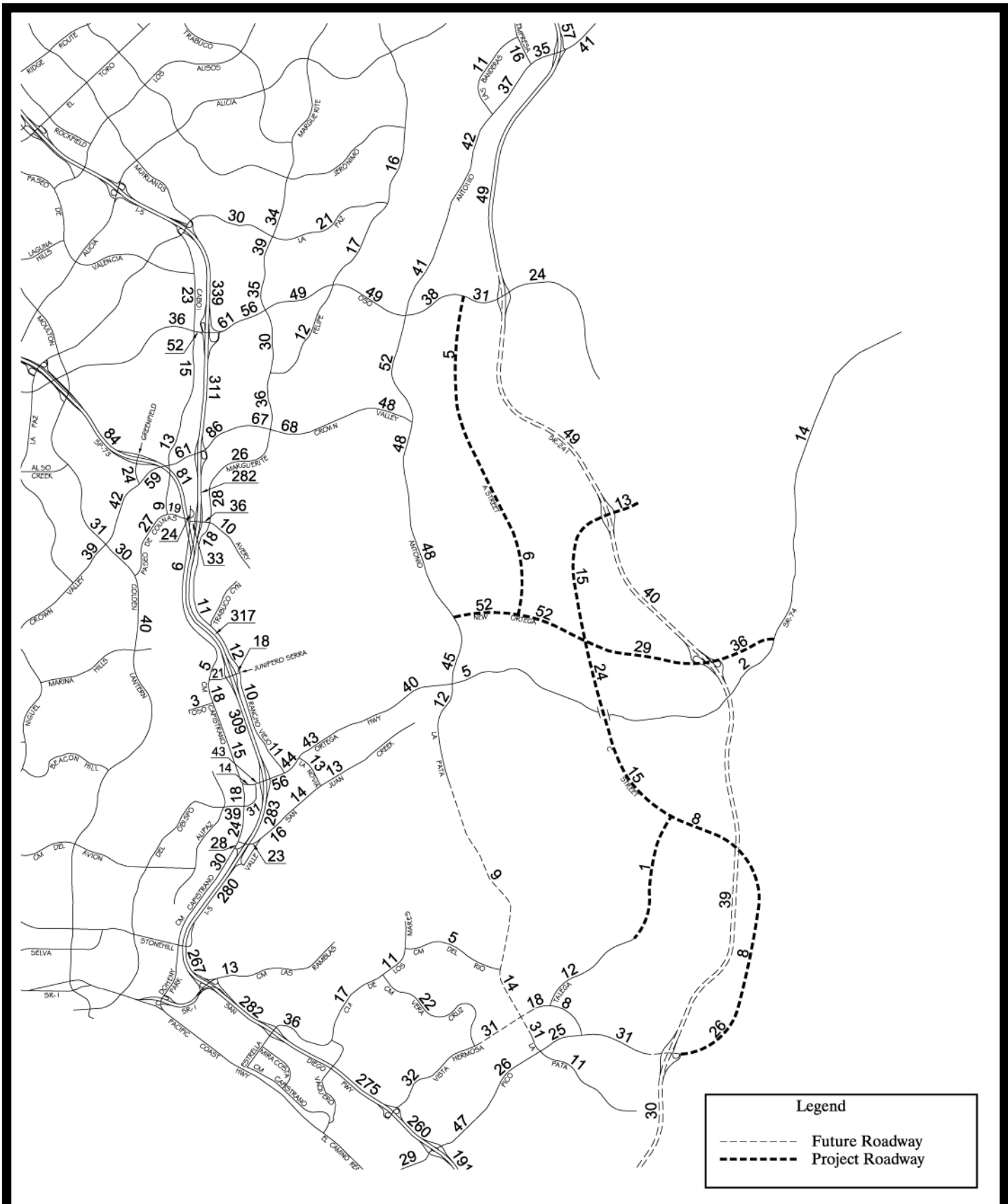
2025 + Alternative B-10 Modified Buildout: ADT Volumes (000s) (Committed Circulation System with La Pata and SR-241 Extension)
