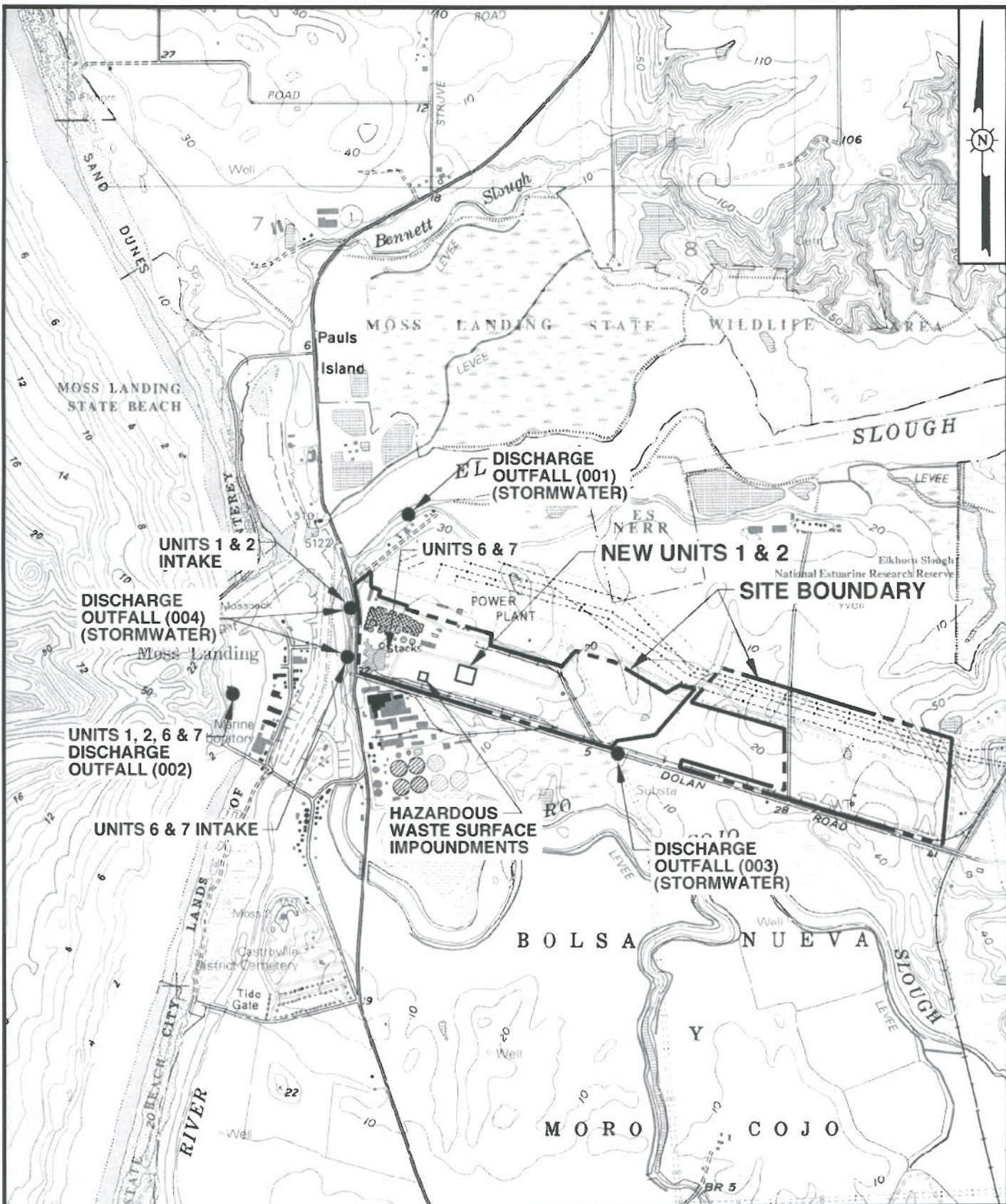
Figure 1 Site Map Facility Discharge Locations Moss Landing Power Plant Units 1, 2, 6 & 7
