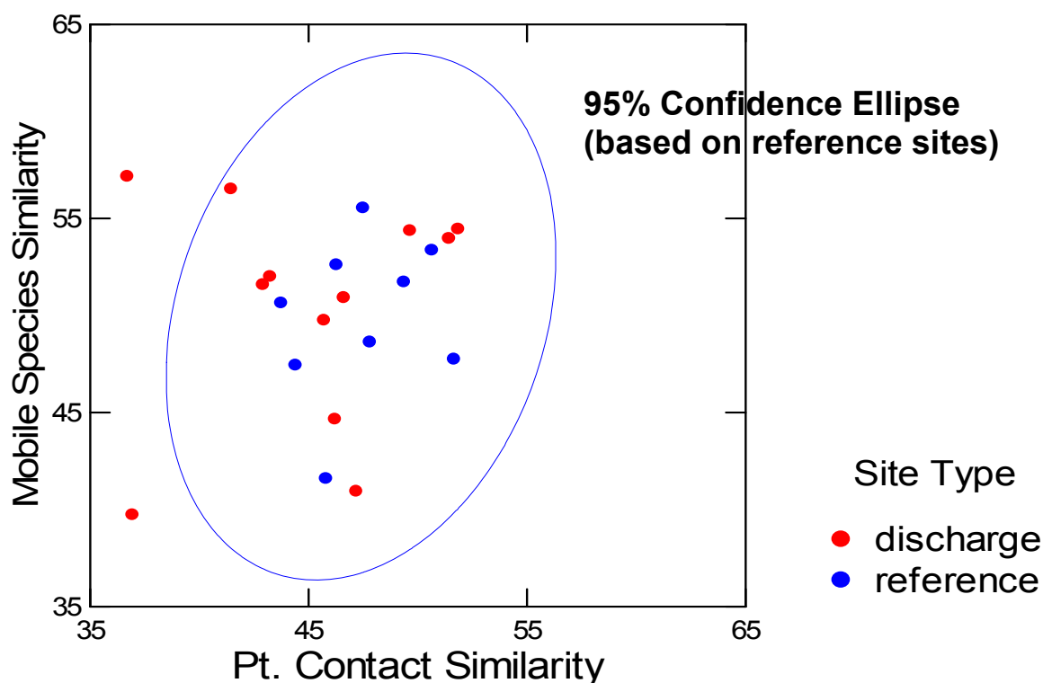
Figure 5.6.8. Similarity of Community Indices and Confidence Ellipse. Source: Pete Raimondi (UC Santa Cruz)
